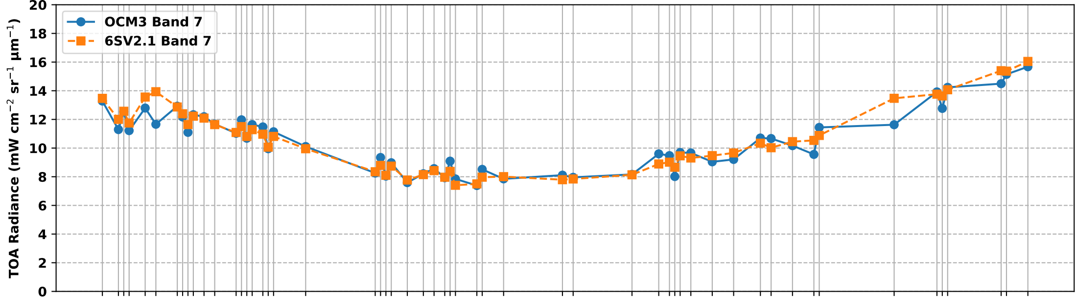
OCM3 Band 7 vs 6S Simulated Band 7 TOA Radiance over RVUS RadCalNet Site (Oct 2025 to Mar 2026)
