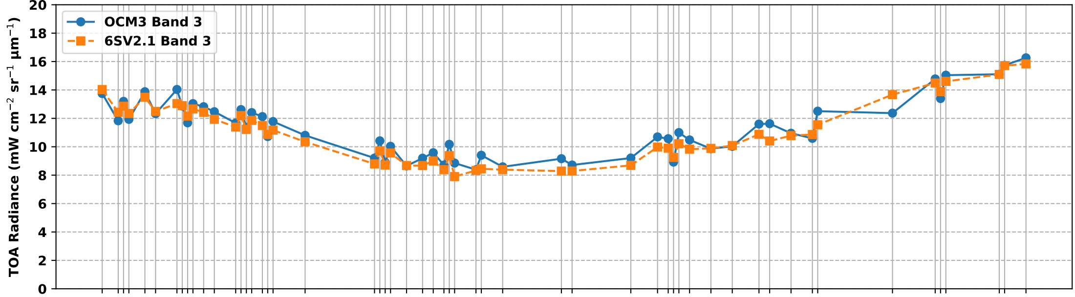
OCM3 Band 3 vs 6S Simulated Band 3 TOA Radiance over RVUS RadCalNet Site (Oct 2025 to Mar 2026)
