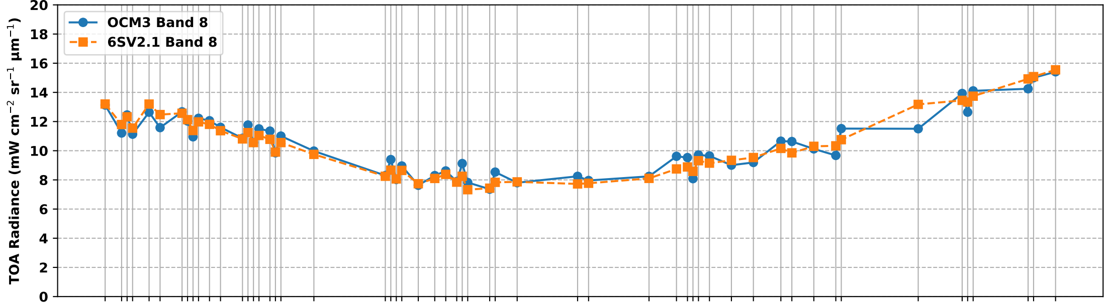
OCM3 Band 8 vs 6S Simulated Band 8 TOA Radiance over RVUS RadCalNet Site (Oct 2025 to Mar 2026)
