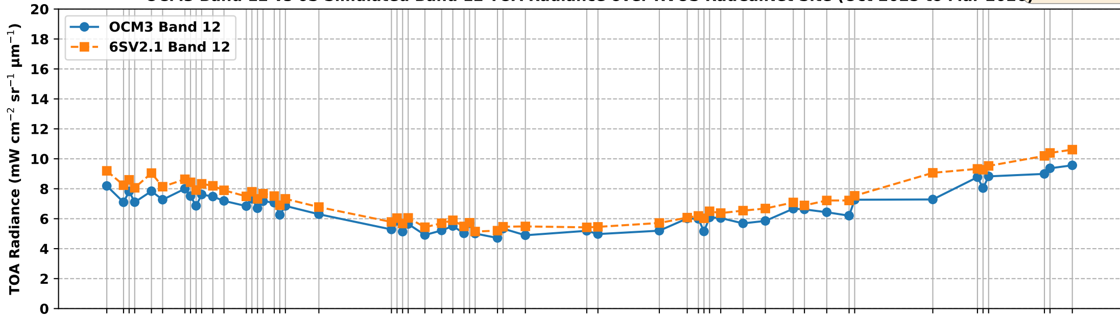
OCM3 Band 12 vs 6S Simulated Band 12 TOA Radiance over RVUS RadCalNet Site (Oct 2025 to Mar 2026)
