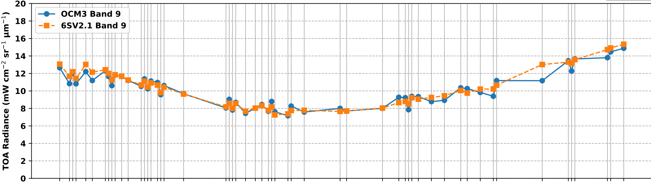
OCM3 Band 9 vs 6S Simulated Band 9 TOA Radiance over RVUS RadCalNet Site (Oct 2025 to Mar 2026)
