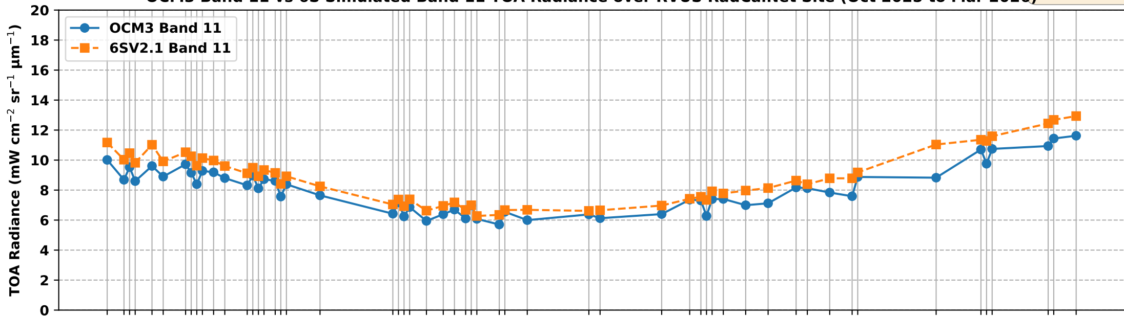
OCM3 Band 11 vs 6S Simulated Band 11 TOA Radiance over RVUS RadCalNet Site (Oct 2025 to Mar 2026)
