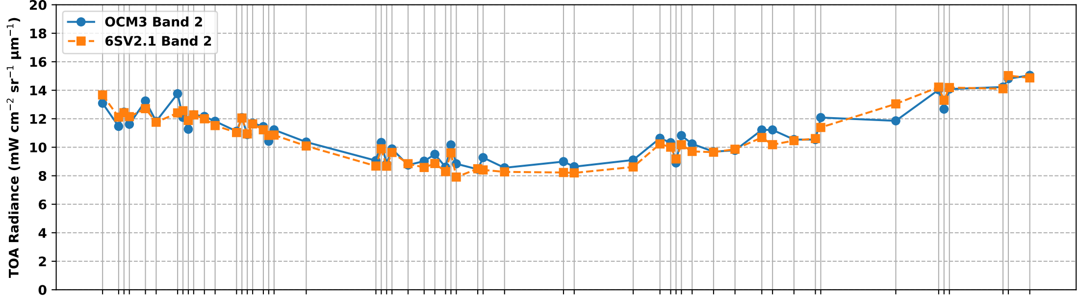
OCM3 Band 2 vs 6S Simulated Band 2 TOA Radiance over RVUS RadCalNet Site (Oct 2025 to Mar 2026)
