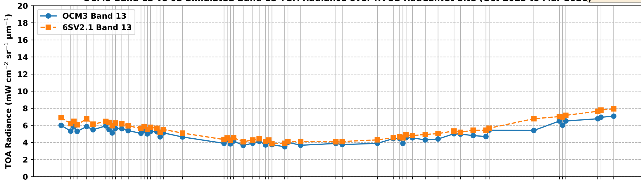
OCM3 Band 13 vs 6S Simulated Band 13 TOA Radiance over RVUS RadCalNet Site (Oct 2025 to Mar 2026)
