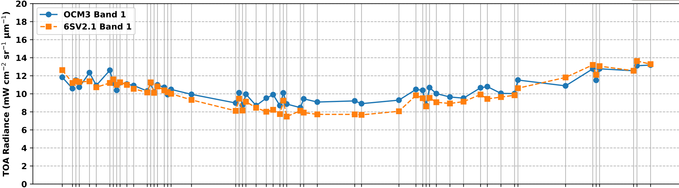
OCM3 Band 1 vs 6S Simulated Band 1 TOA Radiance over RVUS RadCalNet Site (Oct 2025 to Mar 2026)
