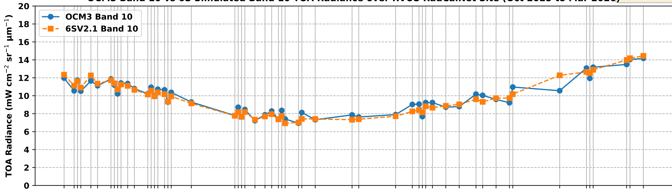
OCM3 Band 10 vs 6S Simulated Band 10 TOA Radiance over RVUS RadCalNet Site (Oct 2025 to Mar 2026)
