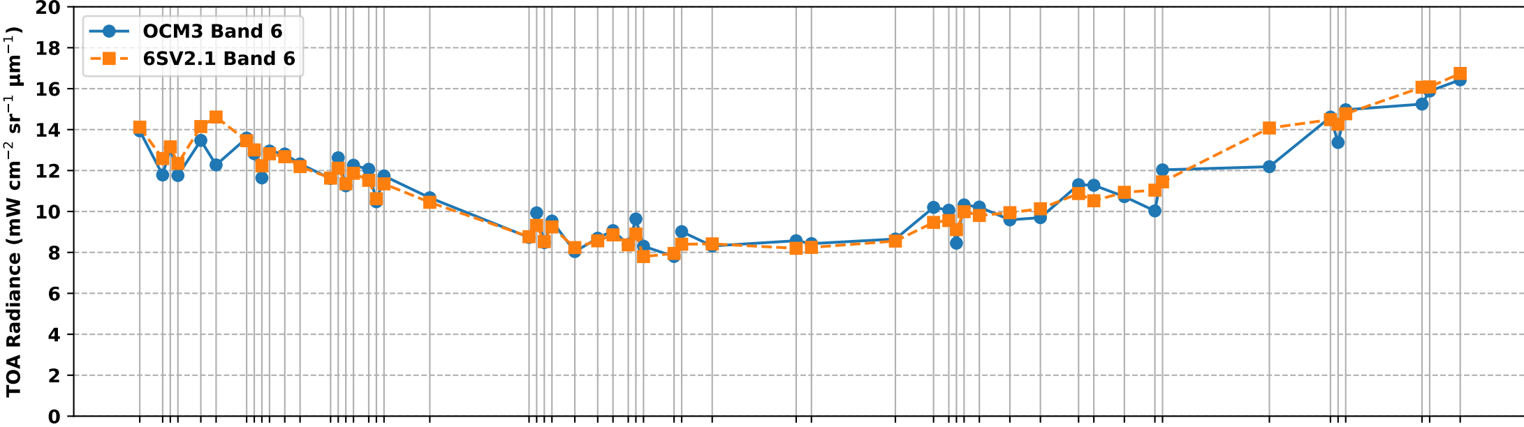
OCM3 Band 6 vs 6S Simulated Band 6 TOA Radiance over RVUS RadCalNet Site (Oct 2025 to Mar 2026)
