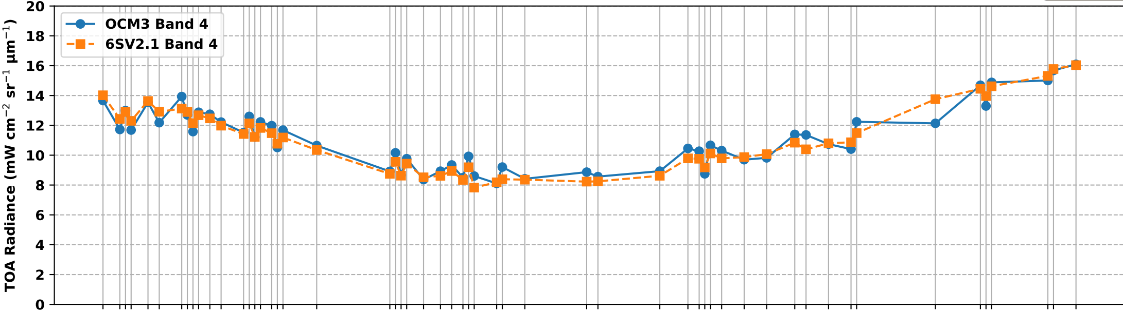
OCM3 Band 4 vs 6S Simulated Band 4 TOA Radiance over RVUS RadCalNet Site (Oct 2025 to Mar 2026)
