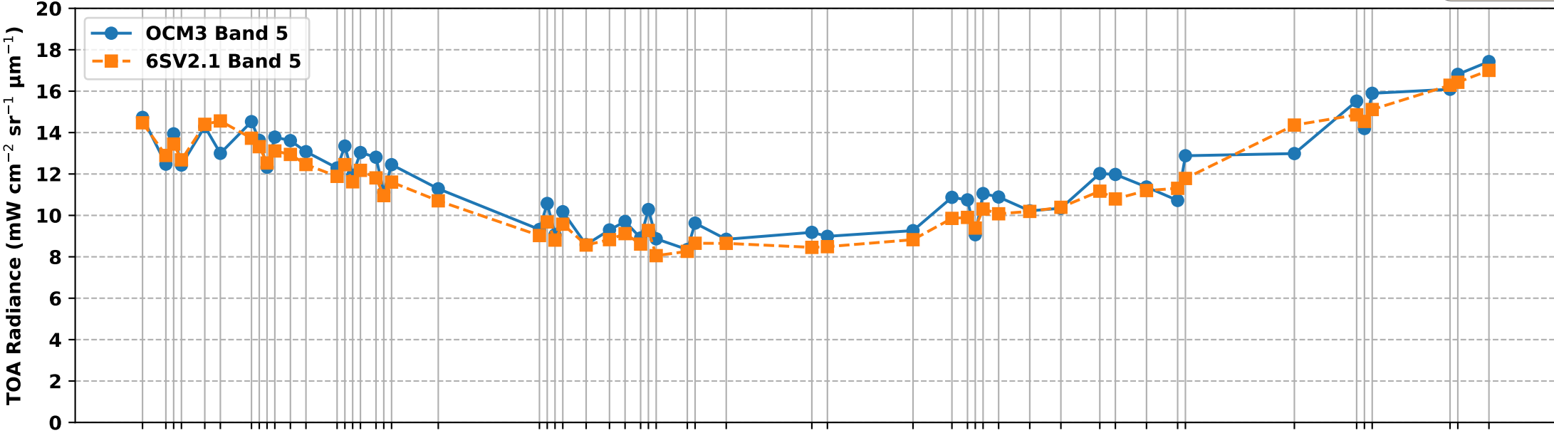
OCM3 Band 5 vs 6S Simulated Band 5 TOA Radiance over RVUS RadCalNet Site (Oct 2025 to Mar 2026)
