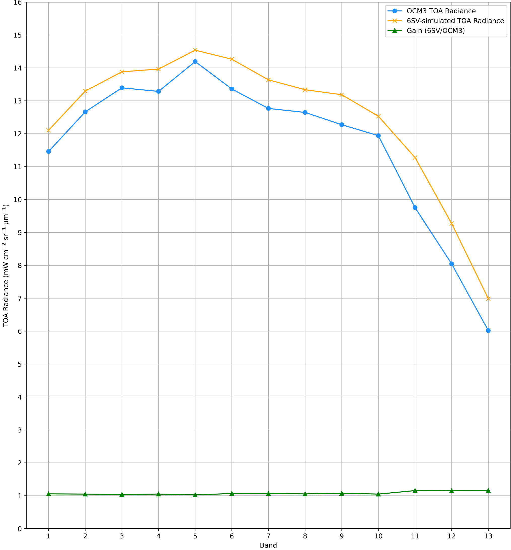
TOA Radiance (OCM3 vs. 6SV) over RVUS RadCalNet Site Lat: 38.497°, Lon: -115.69° - 08-MAR-2026 (STRIP_ID: 17334)
