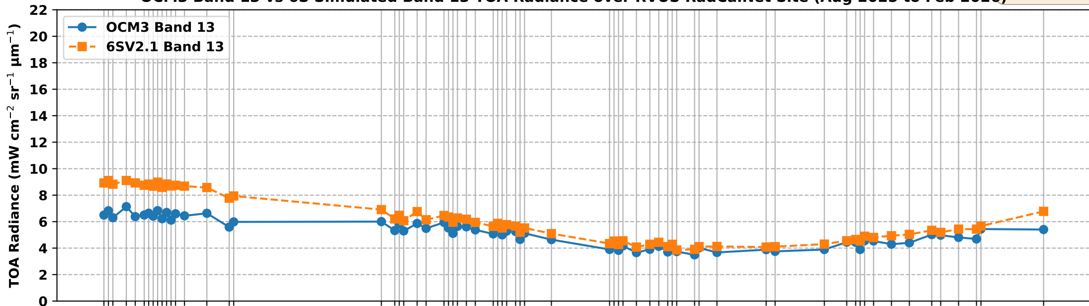
OCM3 Band 13 vs 6S Simulated Band 13 TOA Radiance over RVUS RadCalNet Site (Aug 2025 to Feb 2026)
