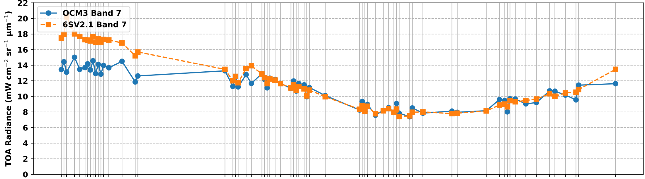
OCM3 Band 7 vs 6S Simulated Band 7 TOA Radiance over RVUS RadCalNet Site (Aug 2025 to Feb 2026)
