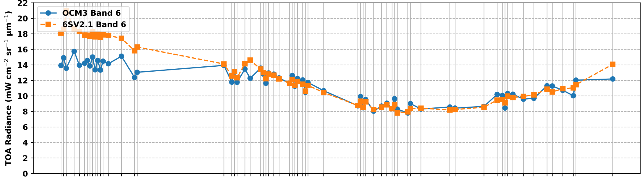
OCM3 Band 6 vs 6S Simulated Band 6 TOA Radiance over RVUS RadCalNet Site (Aug 2025 to Feb 2026)
