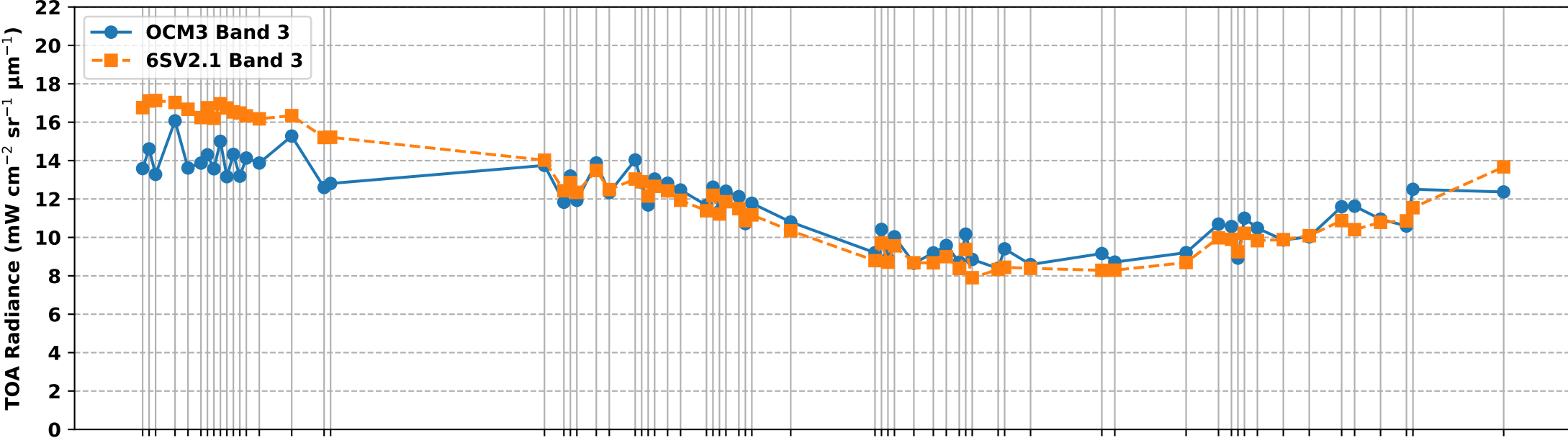
OCM3 Band 3 vs 6S Simulated Band 3 TOA Radiance over RVUS RadCalNet Site (Aug 2025 to Feb 2026)
