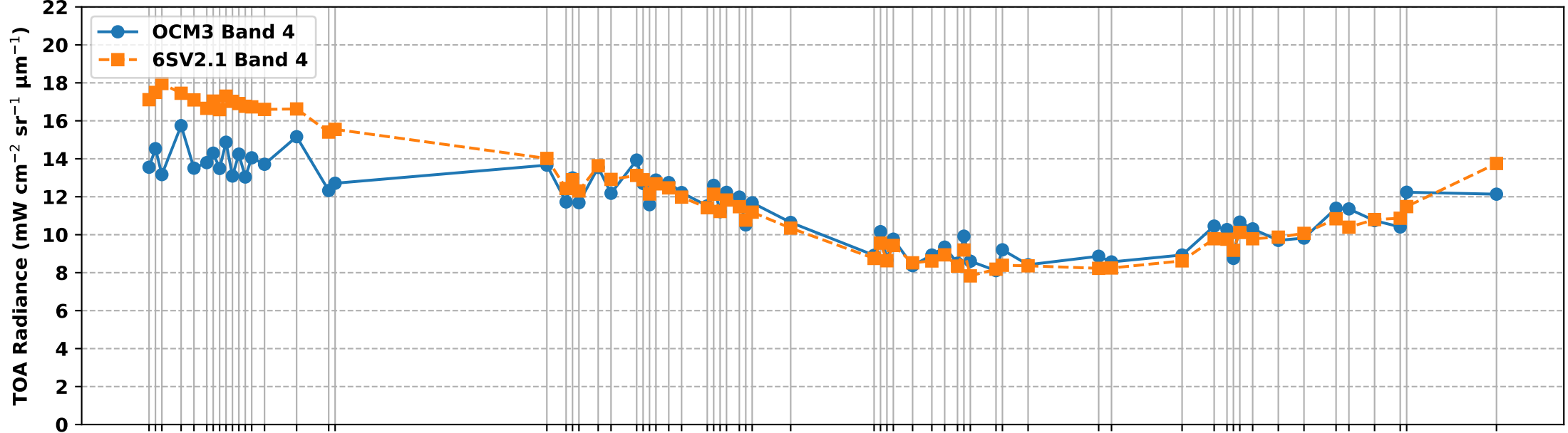
OCM3 Band 4 vs 6S Simulated Band 4 TOA Radiance over RVUS RadCalNet Site (Aug 2025 to Feb 2026)
