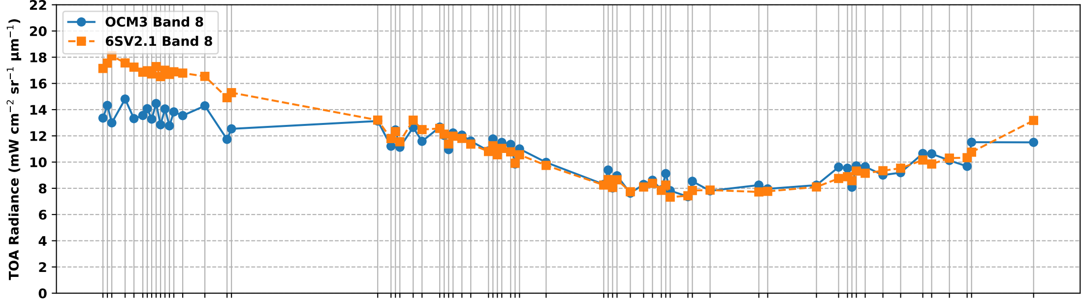
OCM3 Band 8 vs 6S Simulated Band 8 TOA Radiance over RVUS RadCalNet Site (Aug 2025 to Feb 2026)
