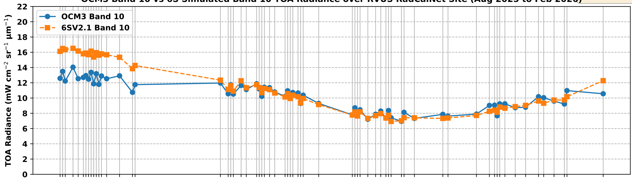
OCM3 Band 10 vs 6S Simulated Band 10 TOA Radiance over RVUS RadCalNet Site (Aug 2025 to Feb 2026)
