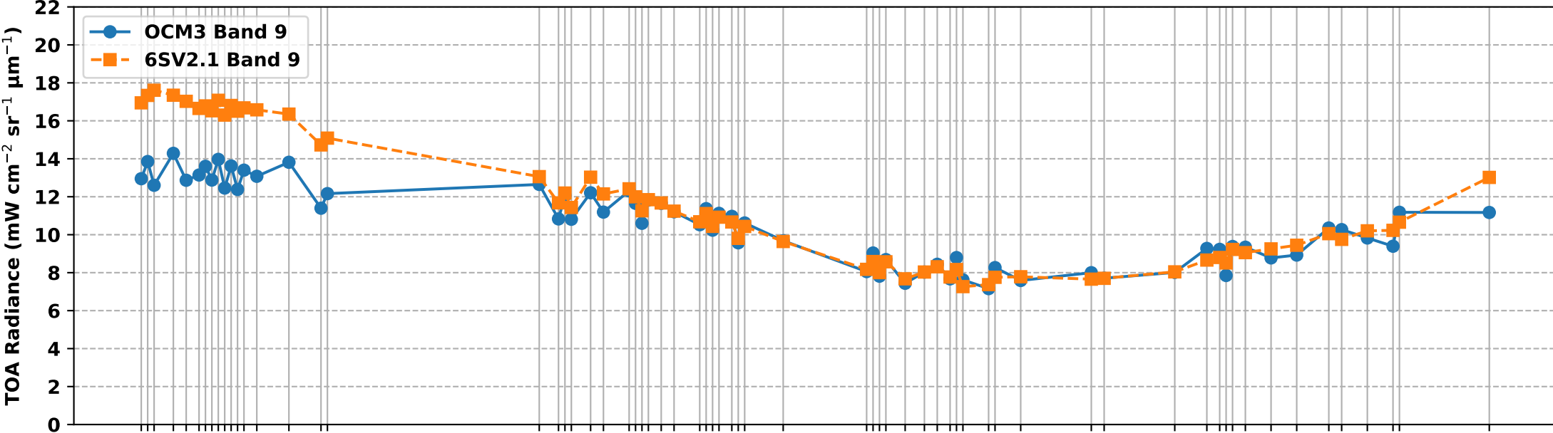
OCM3 Band 9 vs 6S Simulated Band 9 TOA Radiance over RVUS RadCalNet Site (Aug 2025 to Feb 2026)
