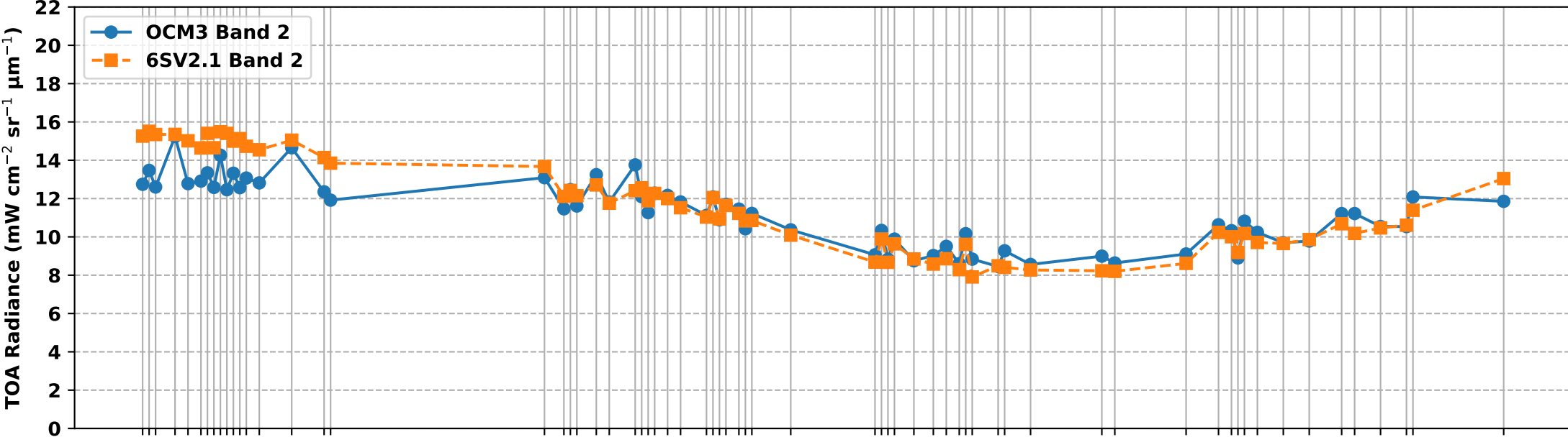
OCM3 Band 2 vs 6S Simulated Band 2 TOA Radiance over RVUS RadCalNet Site (Aug 2025 to Feb 2026)
