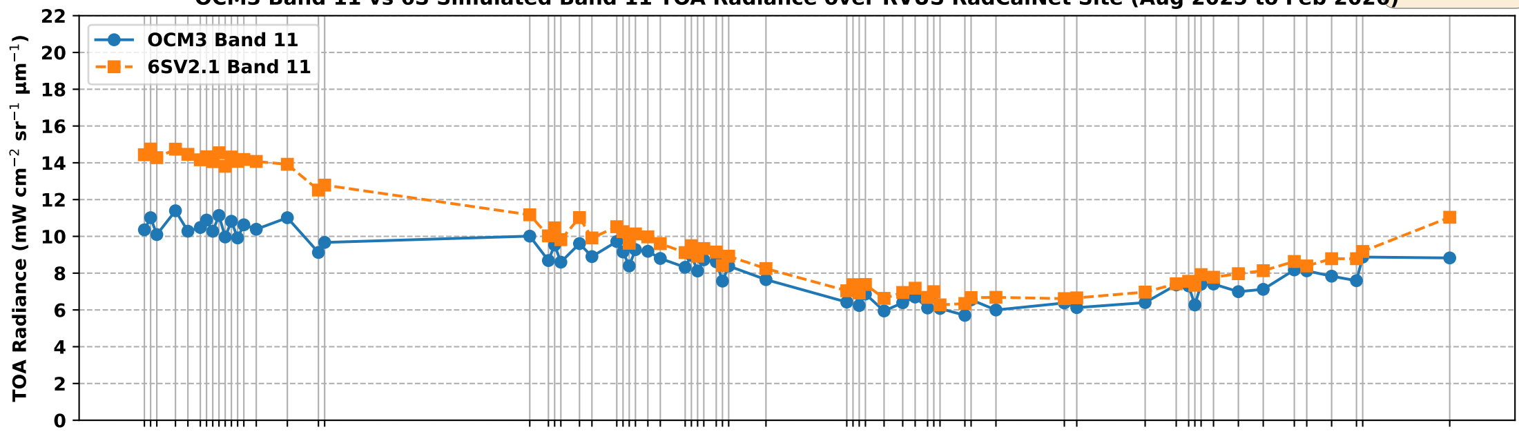
OCM3 Band 11 vs 6S Simulated Band 11 TOA Radiance over RVUS RadCalNet Site (Aug 2025 to Feb 2026)
