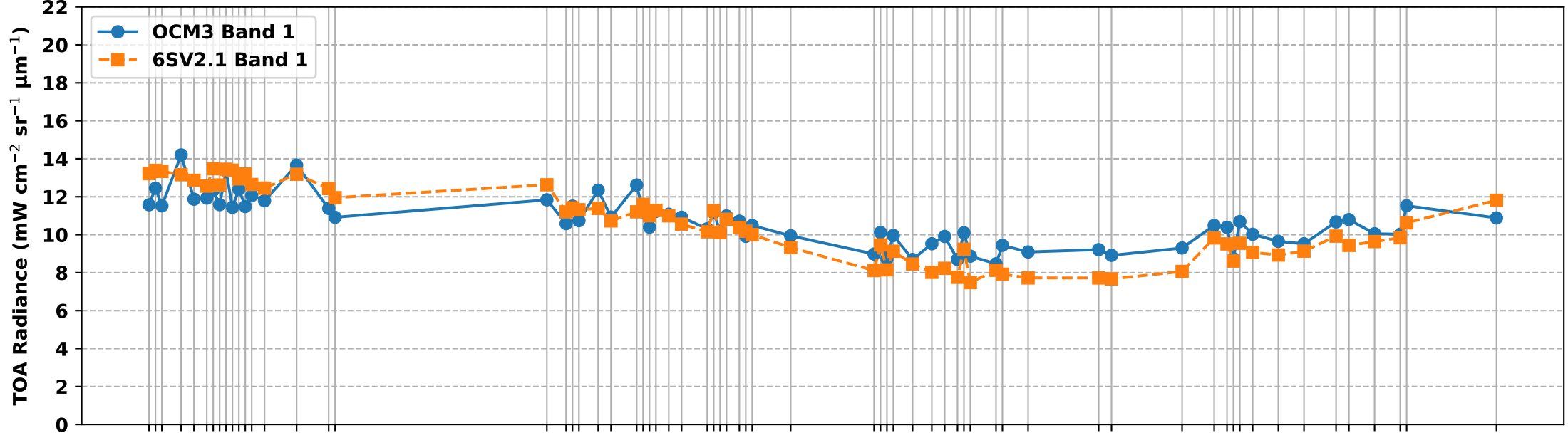
OCM3 Band 1 vs 6S Simulated Band 1 TOA Radiance over RVUS RadCalNet Site (Aug 2025 to Feb 2026)
