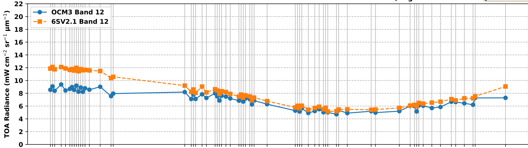
OCM3 Band 12 vs 6S Simulated Band 12 TOA Radiance over RVUS RadCalNet Site (Aug 2025 to Feb 2026)
