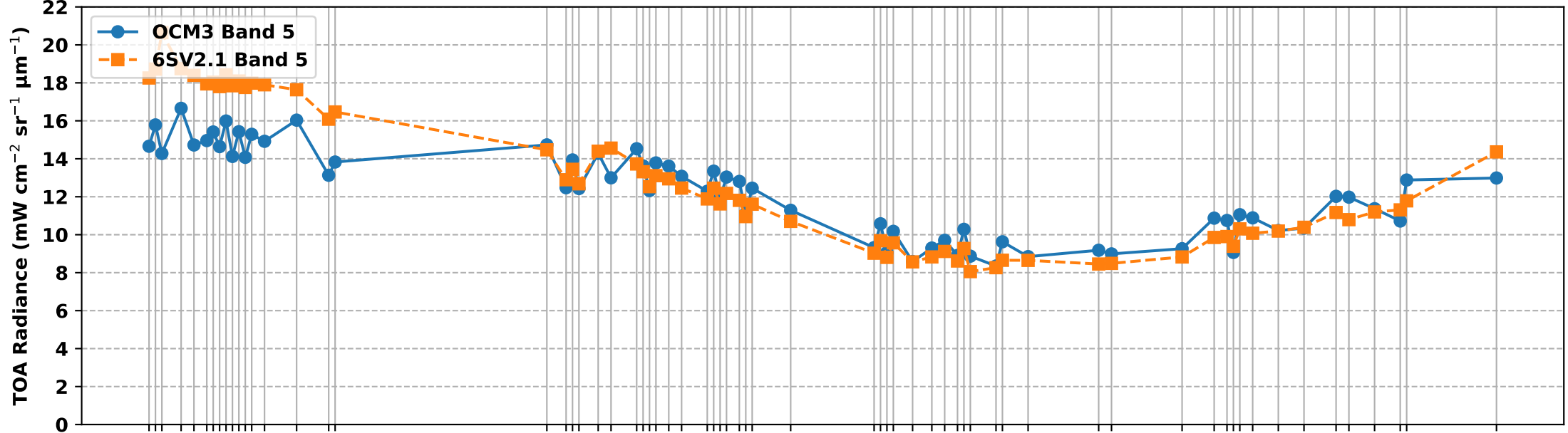
OCM3 Band 5 vs 6S Simulated Band 5 TOA Radiance over RVUS RadCalNet Site (Aug 2025 to Feb 2026)
