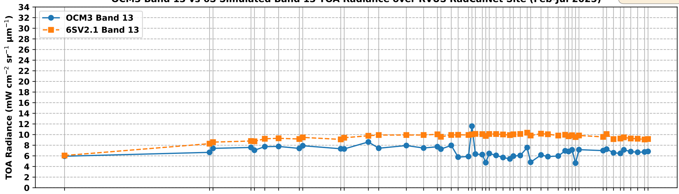
OCM3 Band 13 vs 6S Simulated Band 13 TOA Radiance over RVUS RadCalNet Site (Feb-Jul 2025)
