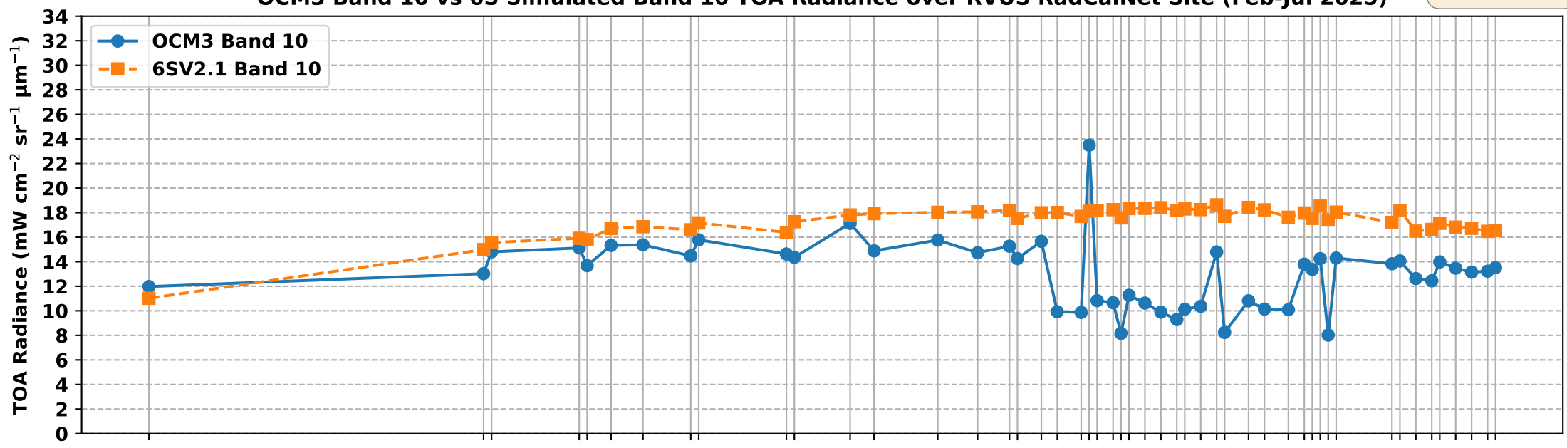
OCM3 Band 10 vs 6S Simulated Band 10 TOA Radiance over RVUS RadCalNet Site (Feb-Jul 2025)
