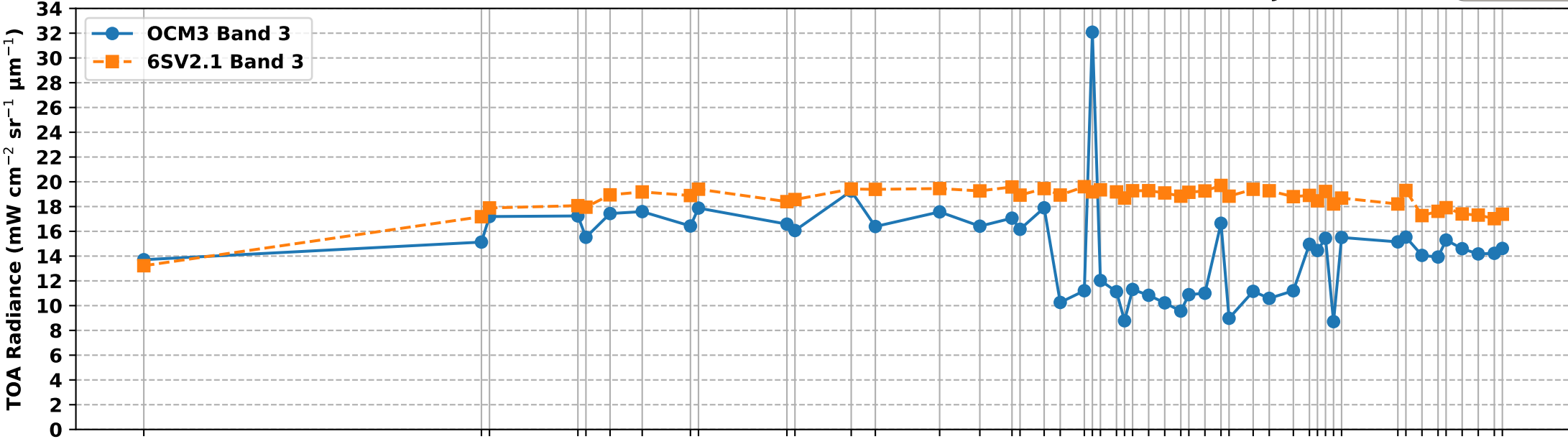
OCM3 Band 3 vs 6S Simulated Band 3 TOA Radiance over RVUS RadCalNet Site (Feb-Jul 2025)
