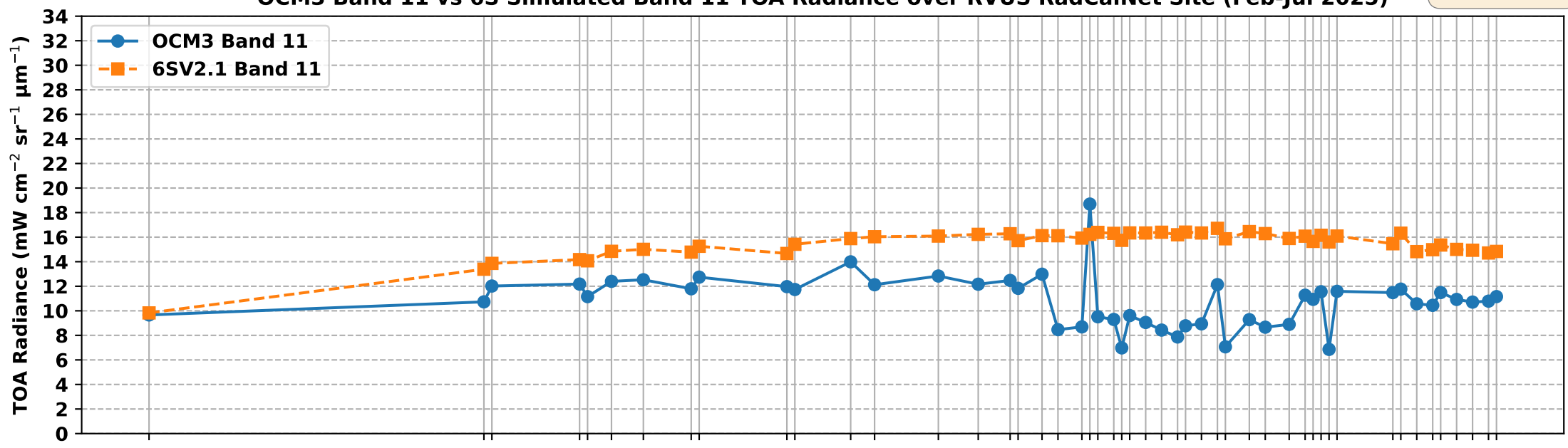
OCM3 Band 11 vs 6S Simulated Band 11 TOA Radiance over RVUS RadCalNet Site (Feb-Jul 2025)
