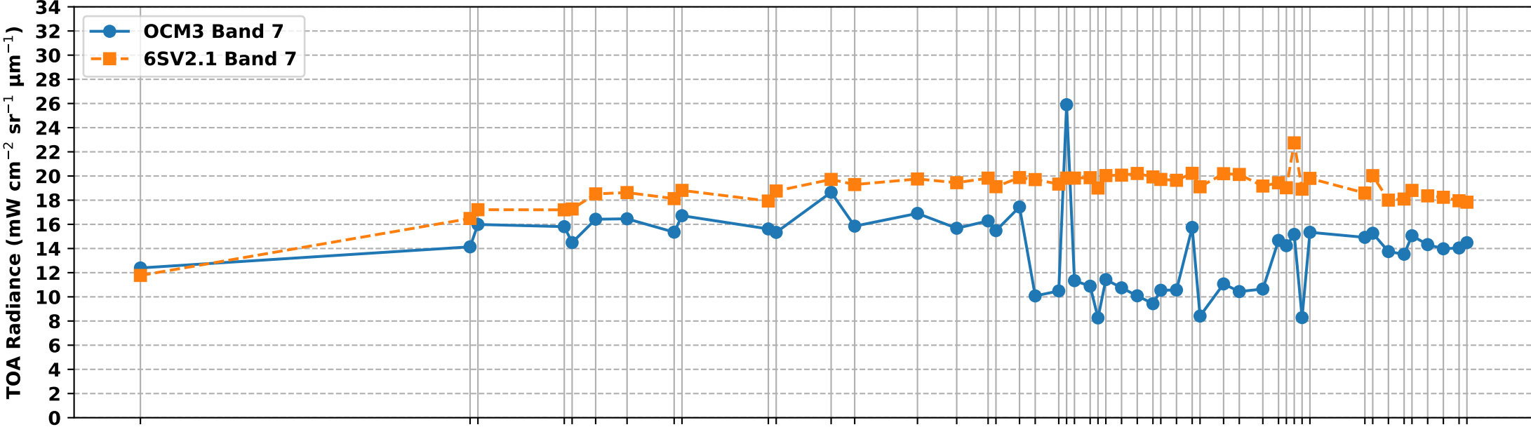
OCM3 Band 7 vs 6S Simulated Band 7 TOA Radiance over RVUS RadCalNet Site (Feb-Jul 2025)
