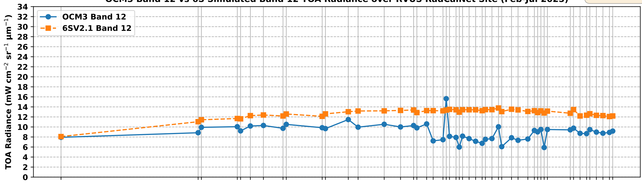
OCM3 Band 12 vs 6S Simulated Band 12 TOA Radiance over RVUS RadCalNet Site (Feb-Jul 2025)
