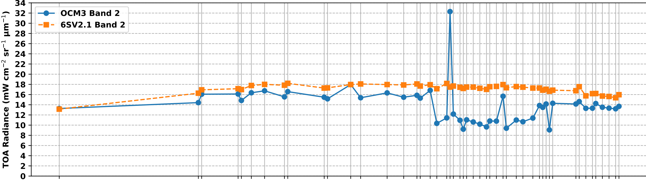
OCM3 Band 2 vs 6S Simulated Band 2 TOA Radiance over RVUS RadCalNet Site (Feb-Jul 2025)
