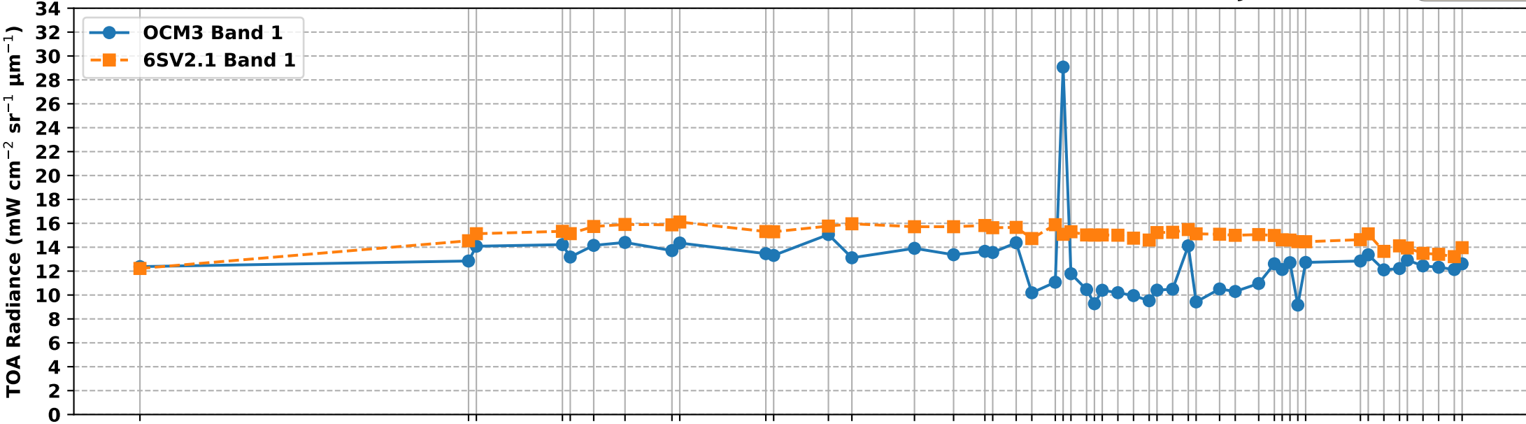
OCM3 Band 1 vs 6S Simulated Band 1 TOA Radiance over RVUS RadCalNet Site (Feb-Jul 2025)
