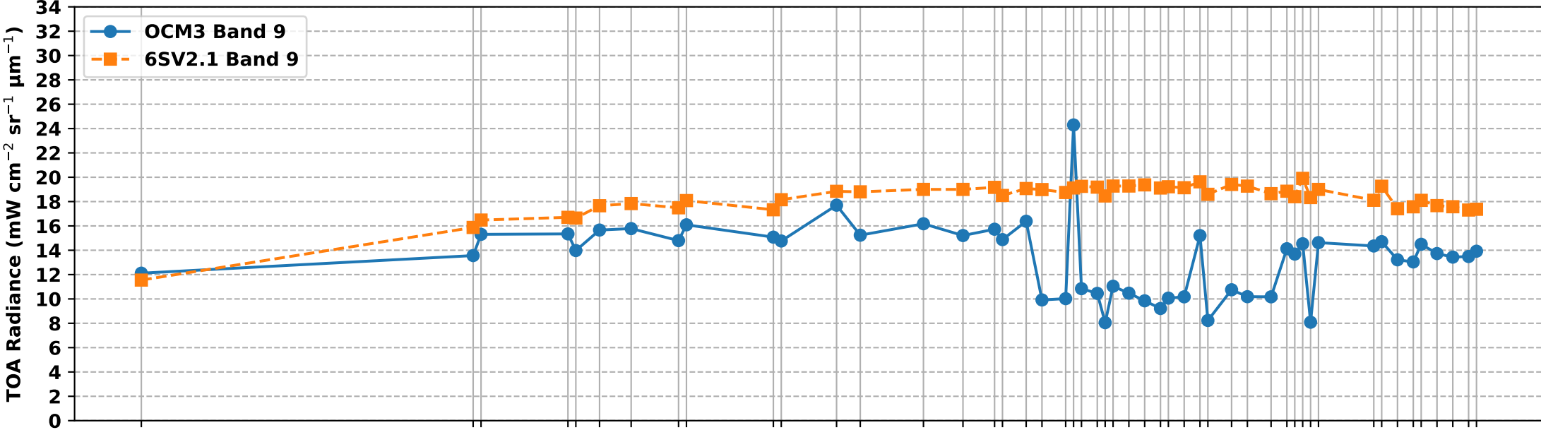
OCM3 Band 9 vs 6S Simulated Band 9 TOA Radiance over RVUS RadCalNet Site (Feb-Jul 2025)
