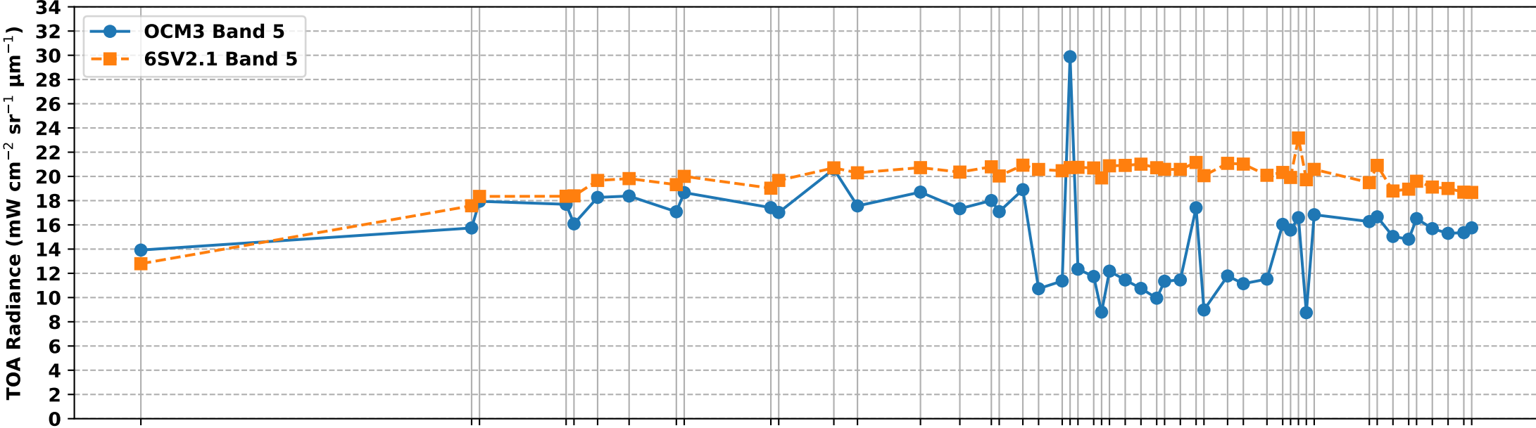
OCM3 Band 5 vs 6S Simulated Band 5 TOA Radiance over RVUS RadCalNet Site (Feb-Jul 2025)
