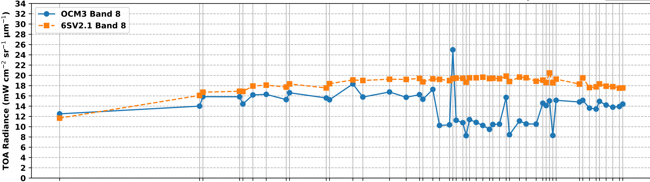
OCM3 Band 8 vs 6S Simulated Band 8 TOA Radiance over RVUS RadCalNet Site (Feb-Jul 2025)
