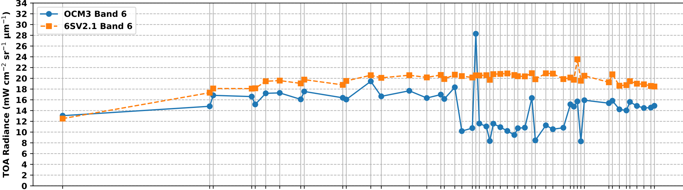
OCM3 Band 6 vs 6S Simulated Band 6 TOA Radiance over RVUS RadCalNet Site (Feb-Jul 2025)
