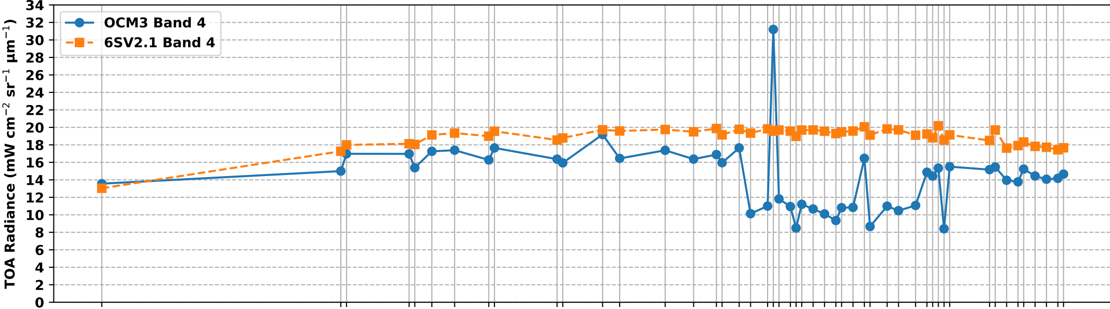
OCM3 Band 4 vs 6S Simulated Band 4 TOA Radiance over RVUS RadCalNet Site (Feb-Jul 2025)
