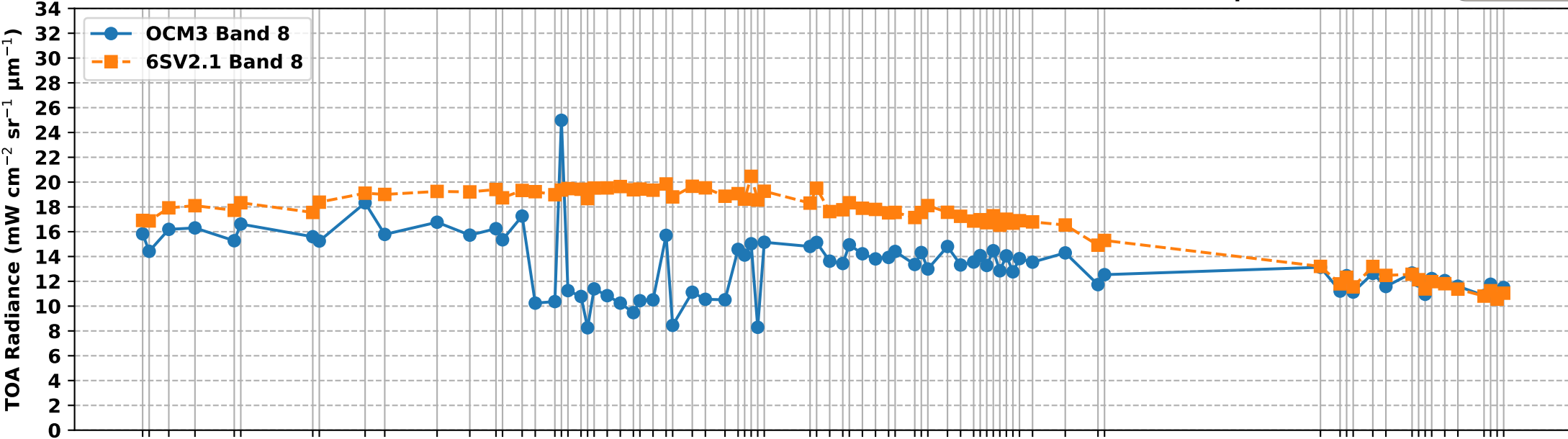
OCM3 Band 8 vs 6S Simulated Band 8 TOA Radiance over RVUS RadCalNet Site (Apr-Oct 2025)
