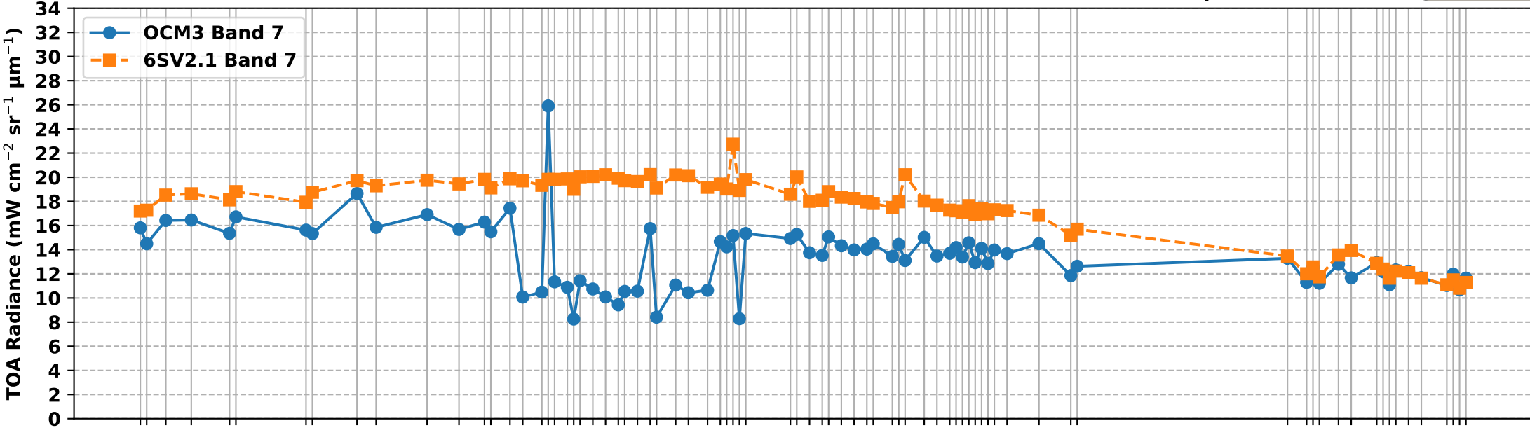
OCM3 Band 7 vs 6S Simulated Band 7 TOA Radiance over RVUS RadCalNet Site (Apr-Oct 2025)
