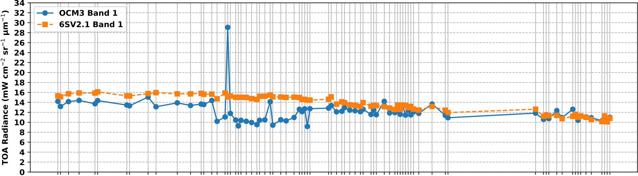
OCM3 Band 1 vs 6S Simulated Band 1 TOA Radiance over RVUS RadCalNet Site (Apr-Oct 2025)
