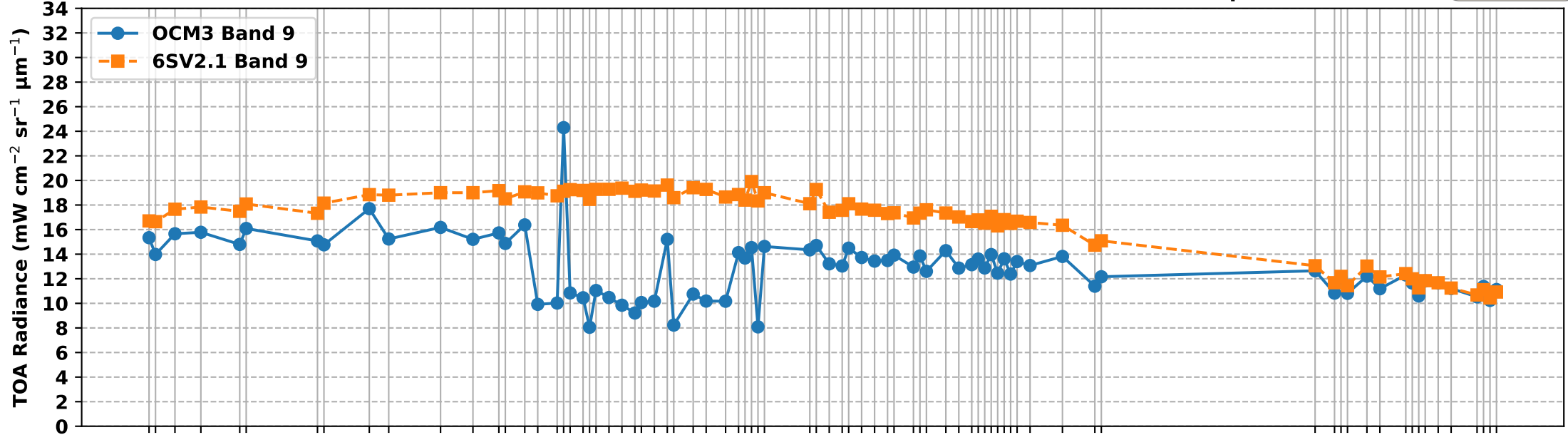
OCM3 Band 9 vs 6S Simulated Band 9 TOA Radiance over RVUS RadCalNet Site (Apr-Oct 2025)
