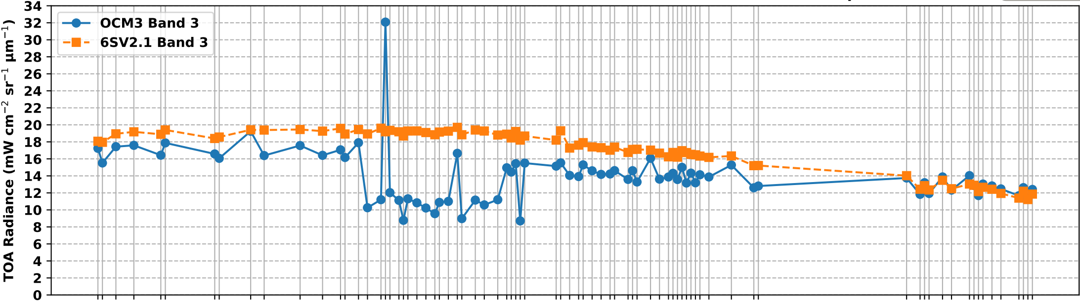
OCM3 Band 3 vs 6S Simulated Band 3 TOA Radiance over RVUS RadCalNet Site (Apr-Oct 2025)
