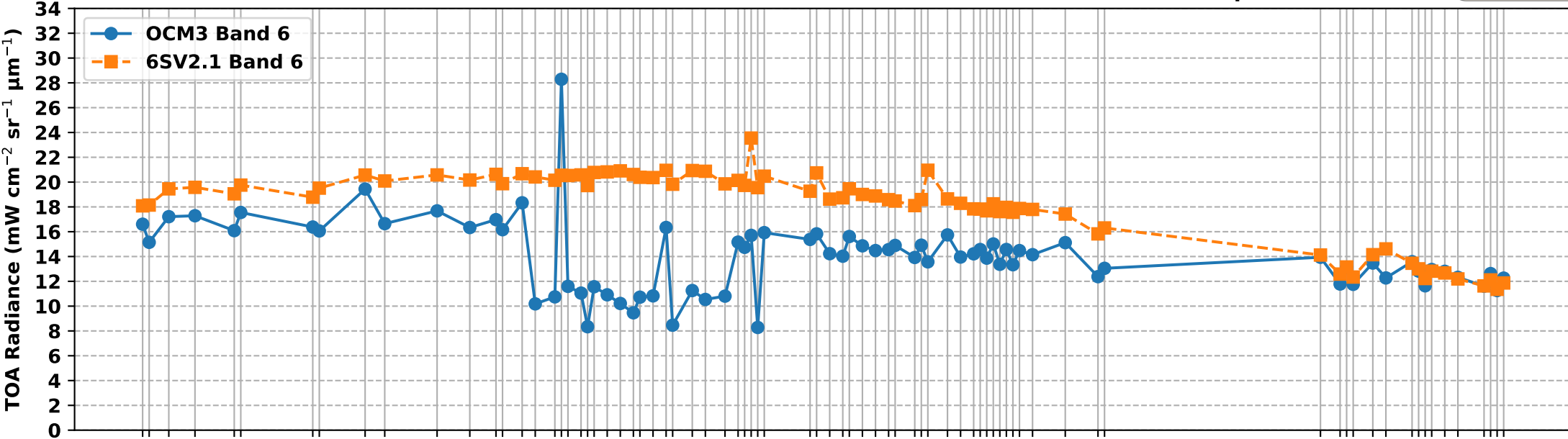
OCM3 Band 6 vs 6S Simulated Band 6 TOA Radiance over RVUS RadCalNet Site (Apr-Oct 2025)
