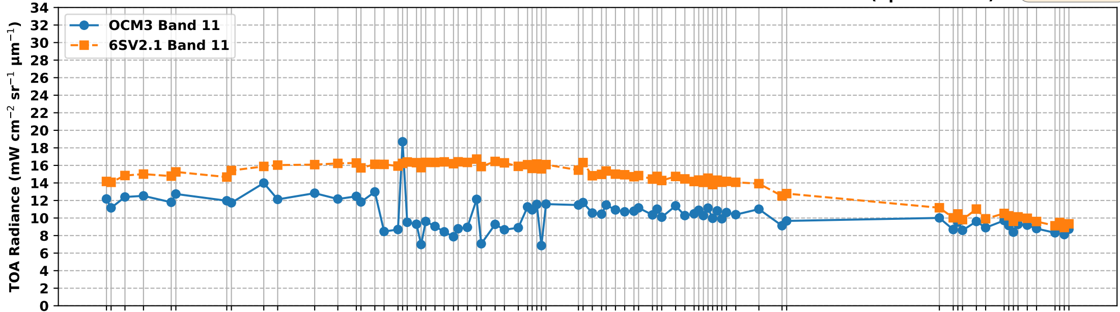
OCM3 Band 11 vs 6S Simulated Band 11 TOA Radiance over RVUS RadCalNet Site (Apr-Oct 2025)
