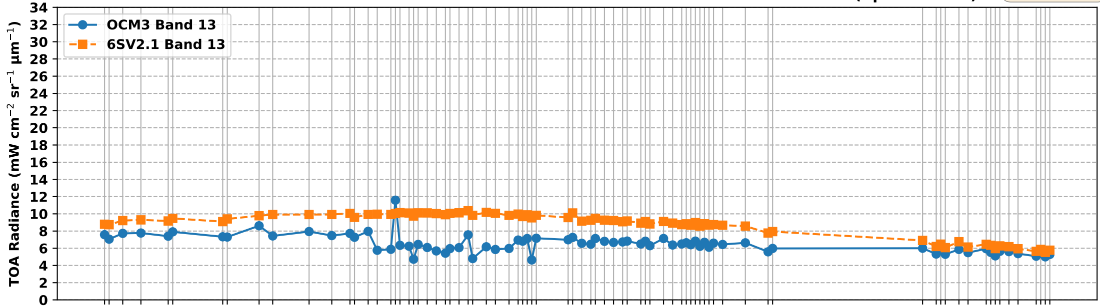
OCM3 Band 13 vs 6S Simulated Band 13 TOA Radiance over RVUS RadCalNet Site (Apr-Oct 2025)
