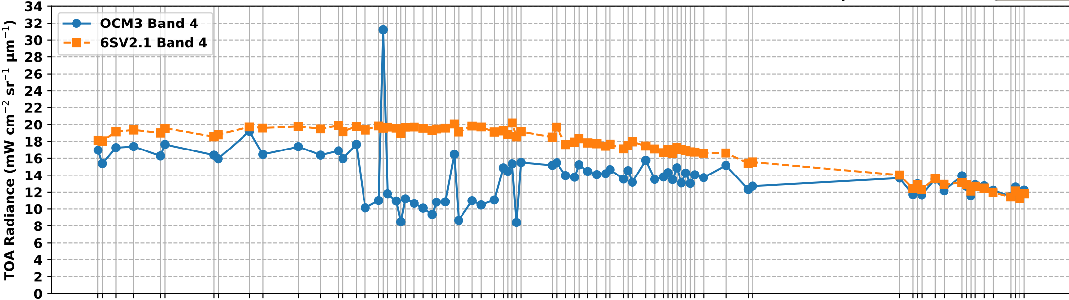
OCM3 Band 4 vs 6S Simulated Band 4 TOA Radiance over RVUS RadCalNet Site (Apr-Oct 2025)
