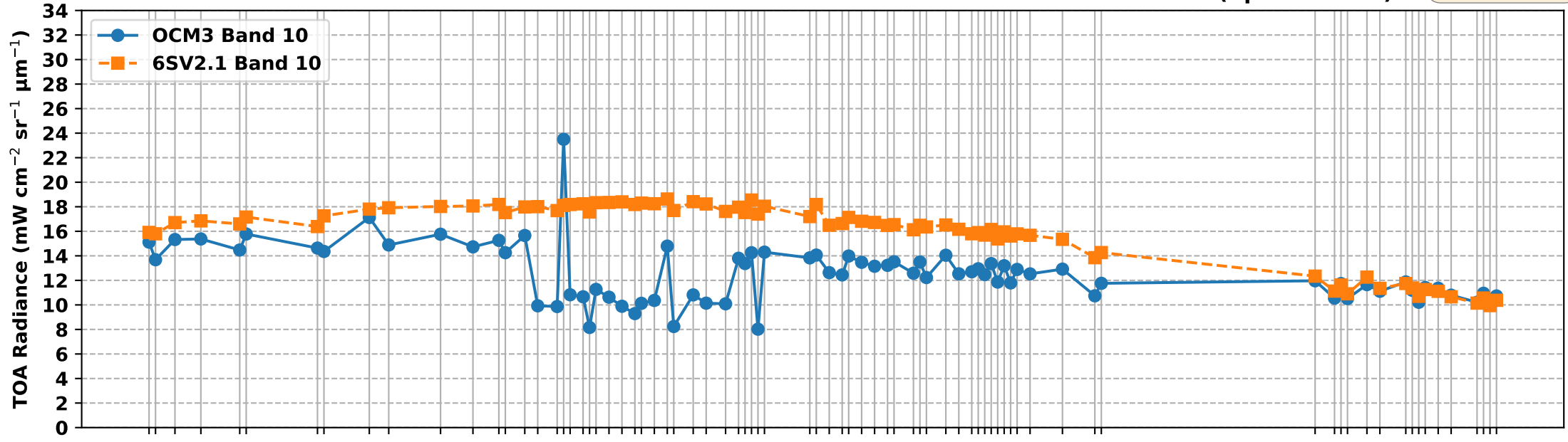
OCM3 Band 10 vs 6S Simulated Band 10 TOA Radiance over RVUS RadCalNet Site (Apr-Oct 2025)
