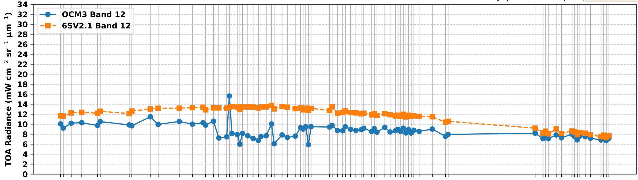
OCM3 Band 12 vs 6S Simulated Band 12 TOA Radiance over RVUS RadCalNet Site (Apr-Oct 2025)
