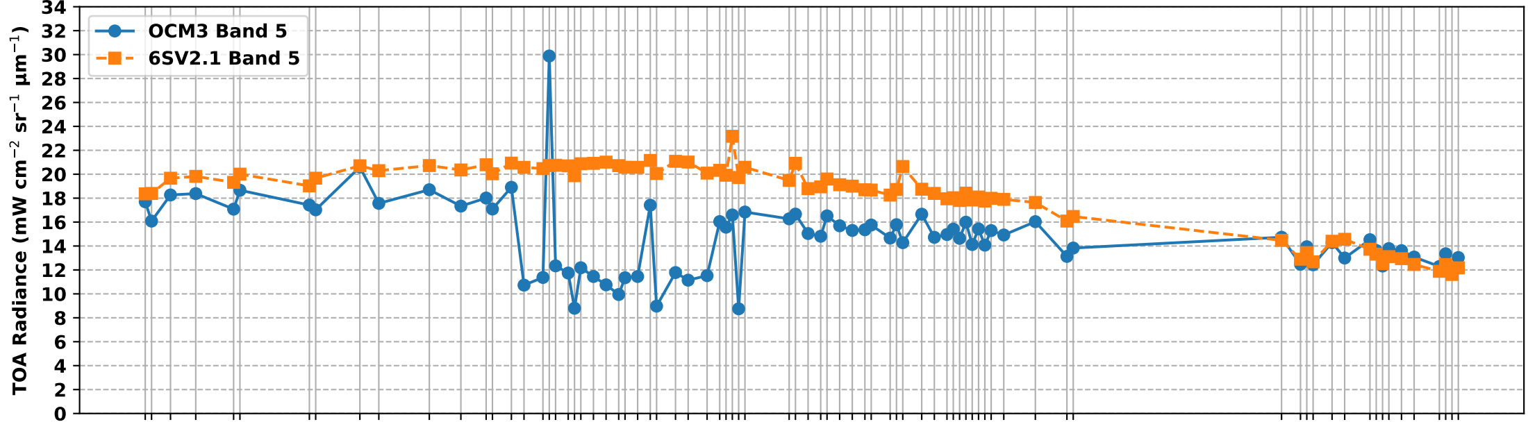
OCM3 Band 5 vs 6S Simulated Band 5 TOA Radiance over RVUS RadCalNet Site (Apr-Oct 2025)
