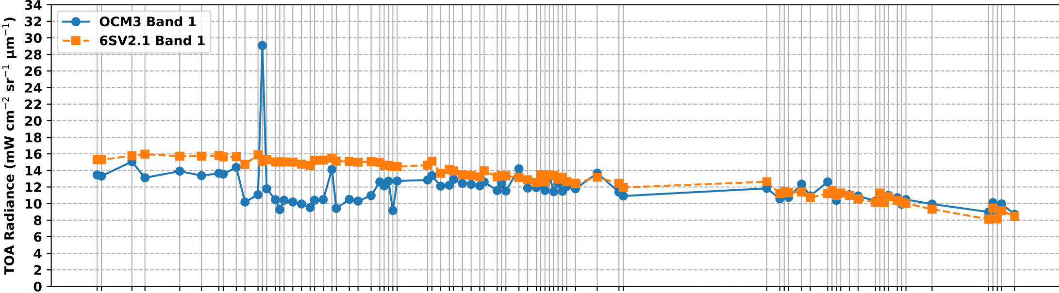
OCM3 Band 1 vs 6S Simulated Band 1 TOA Radiance over RVUS RadCalNet Site (May-Nov 2025)
