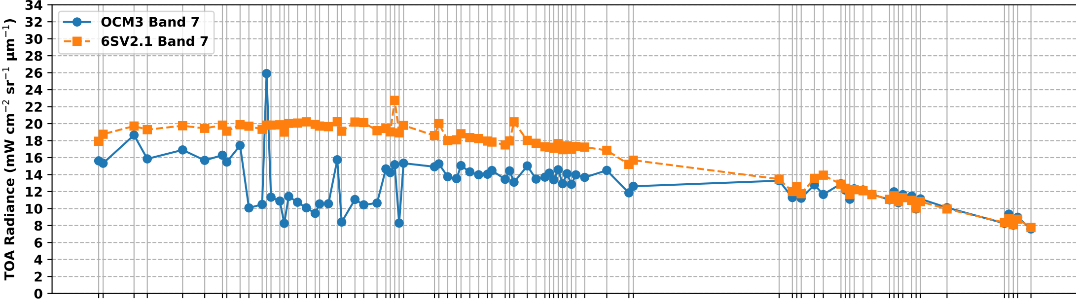
OCM3 Band 7 vs 6S Simulated Band 7 TOA Radiance over RVUS RadCalNet Site (May-Nov 2025)
