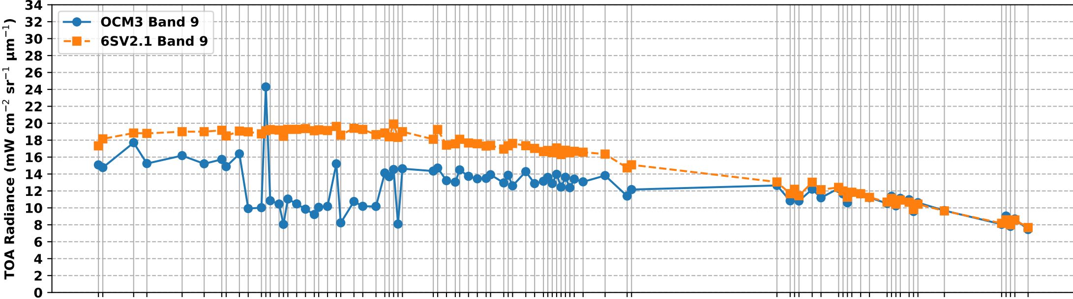
OCM3 Band 9 vs 6S Simulated Band 9 TOA Radiance over RVUS RadCalNet Site (May-Nov 2025)
