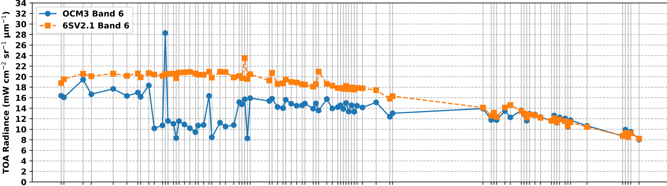
OCM3 Band 6 vs 6S Simulated Band 6 TOA Radiance over RVUS RadCalNet Site (May-Nov 2025)
