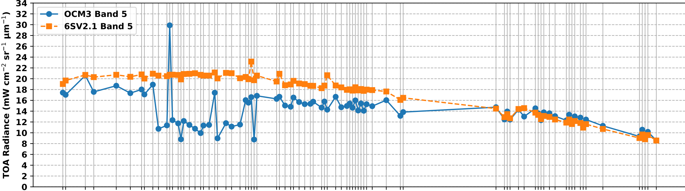
OCM3 Band 5 vs 6S Simulated Band 5 TOA Radiance over RVUS RadCalNet Site (May-Nov 2025)
