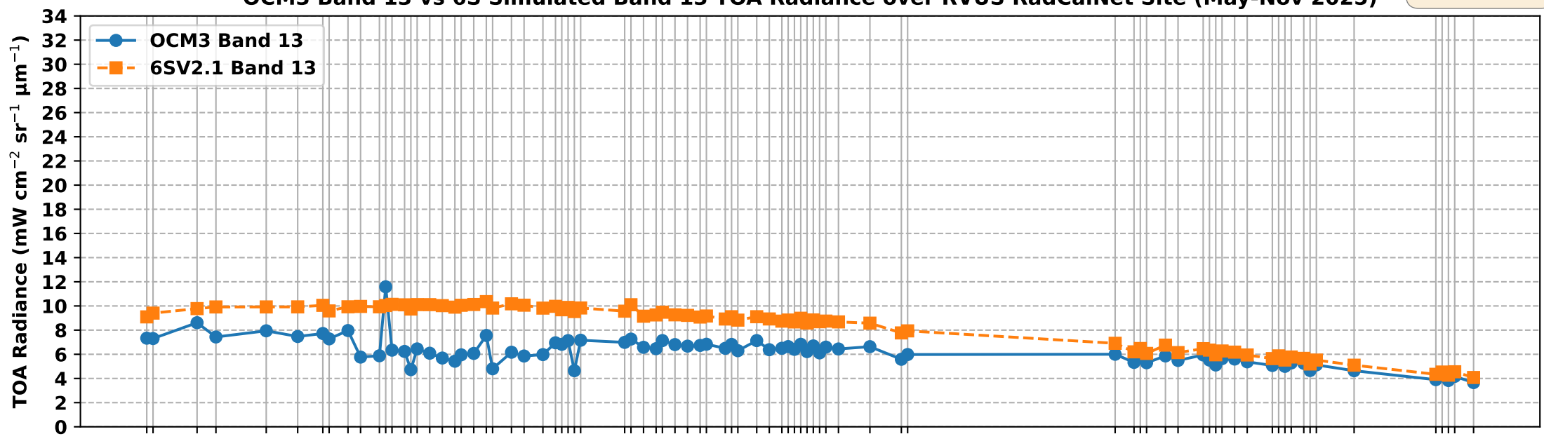
OCM3 Band 13 vs 6S Simulated Band 13 TOA Radiance over RVUS RadCalNet Site (May-Nov 2025)
