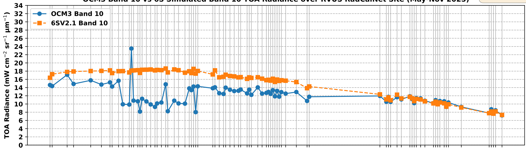
OCM3 Band 10 vs 6S Simulated Band 10 TOA Radiance over RVUS RadCalNet Site (May-Nov 2025)
