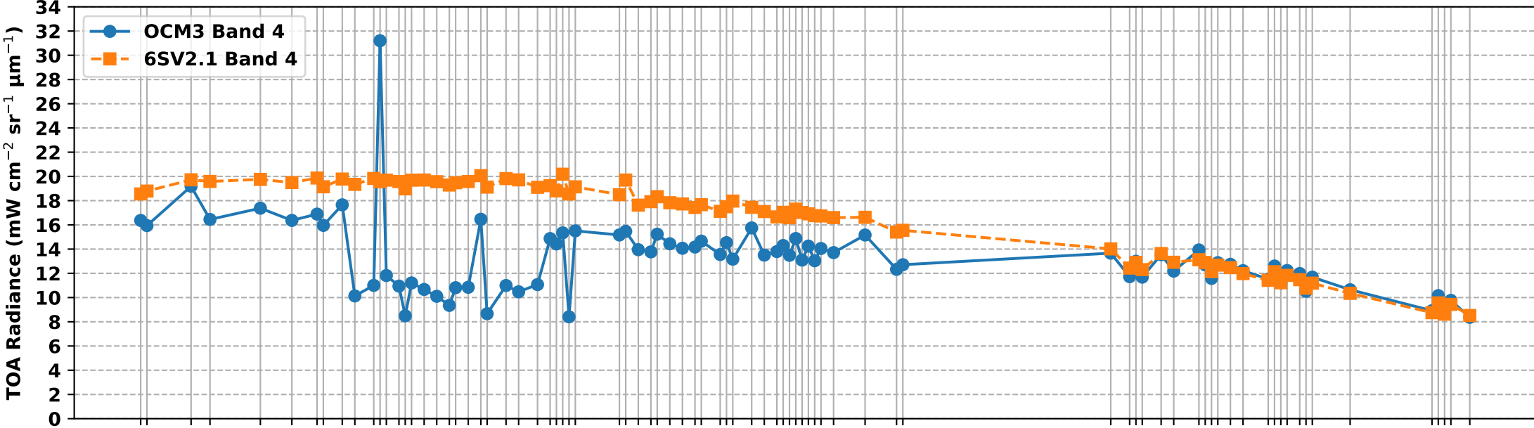
OCM3 Band 4 vs 6S Simulated Band 4 TOA Radiance over RVUS RadCalNet Site (May-Nov 2025)
