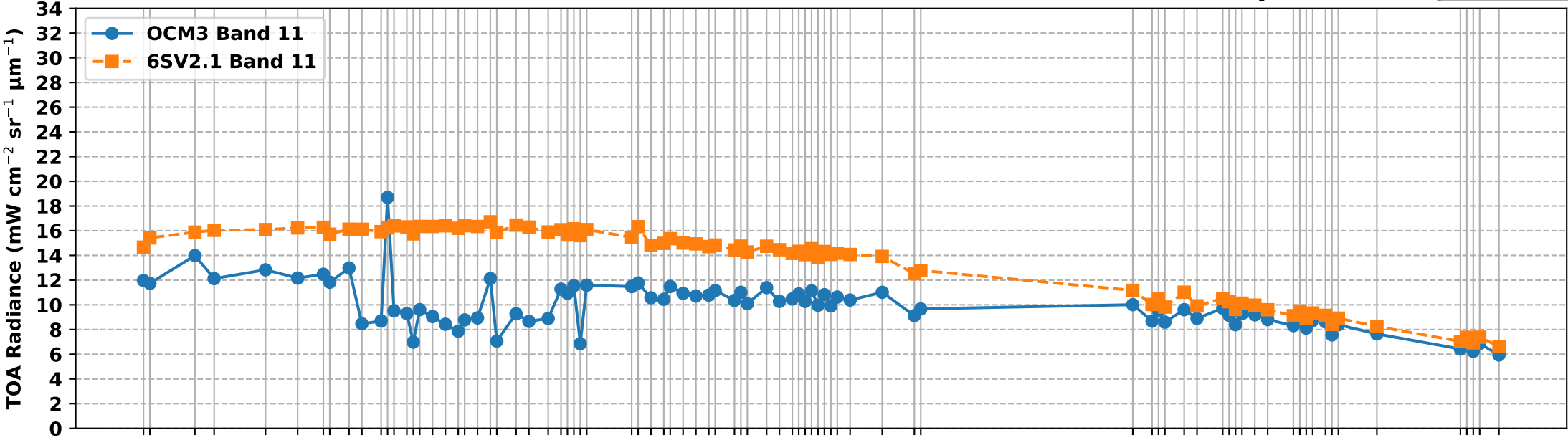
OCM3 Band 11 vs 6S Simulated Band 11 TOA Radiance over RVUS RadCalNet Site (May-Nov 2025)
