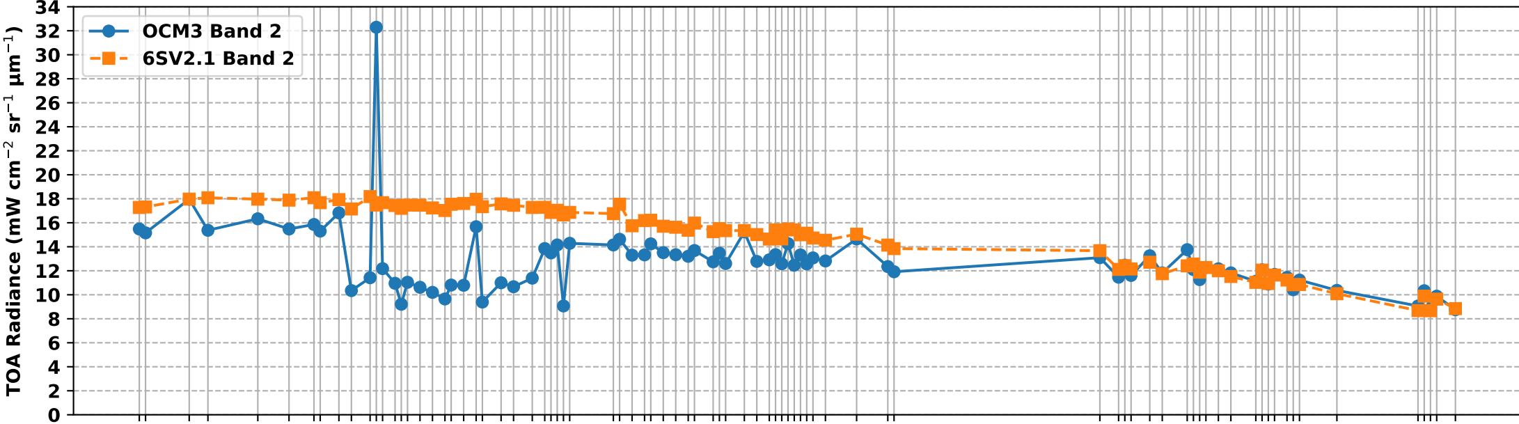
OCM3 Band 2 vs 6S Simulated Band 2 TOA Radiance over RVUS RadCalNet Site (May-Nov 2025)
