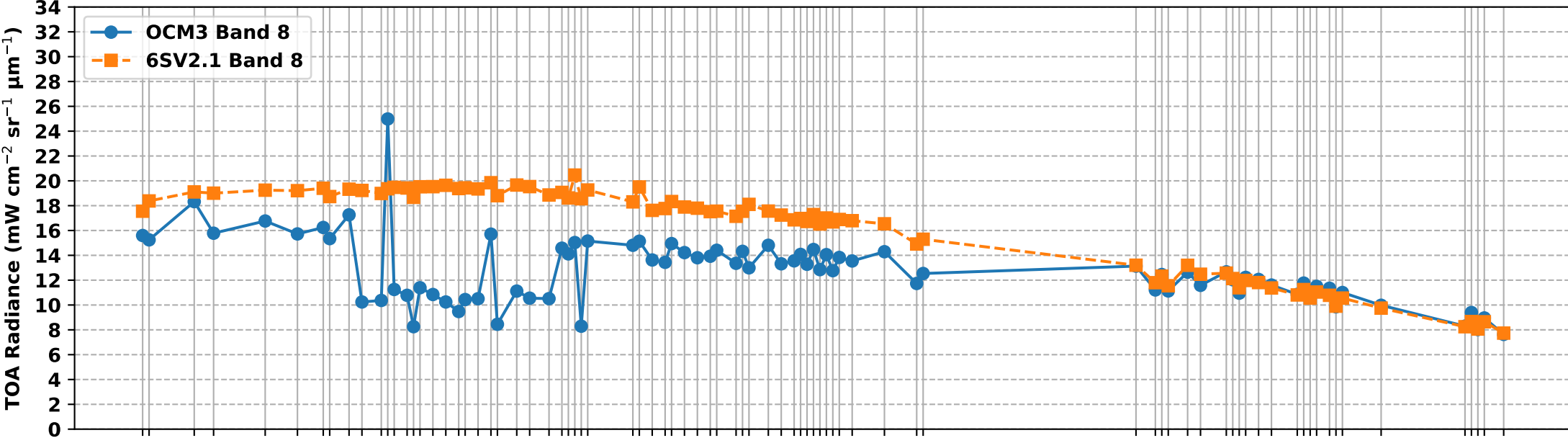
OCM3 Band 8 vs 6S Simulated Band 8 TOA Radiance over RVUS RadCalNet Site (May-Nov 2025)
