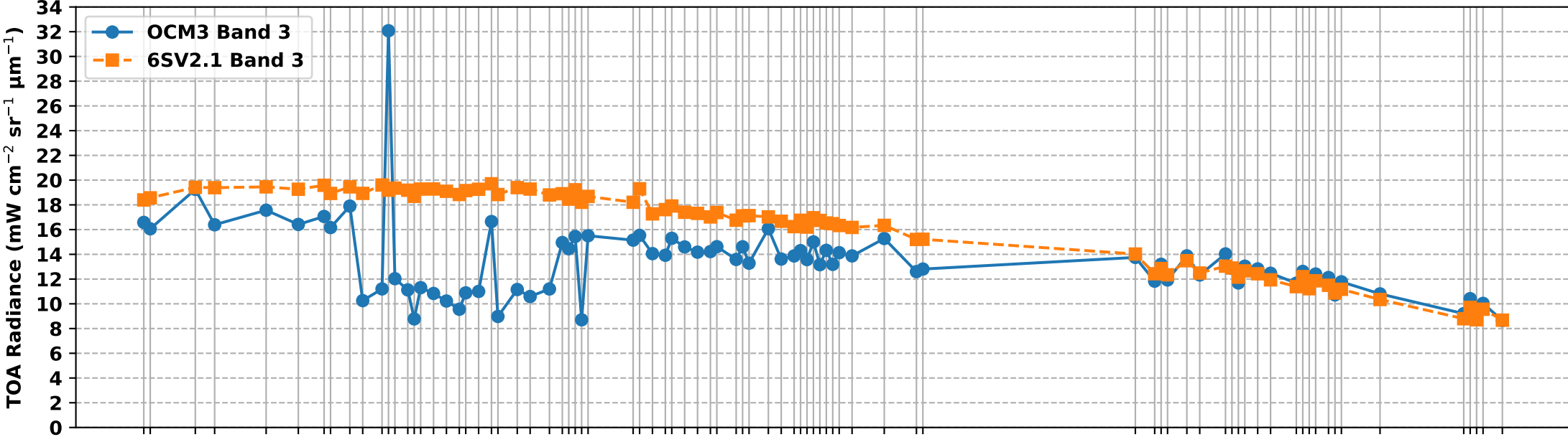
OCM3 Band 3 vs 6S Simulated Band 3 TOA Radiance over RVUS RadCalNet Site (May-Nov 2025)
