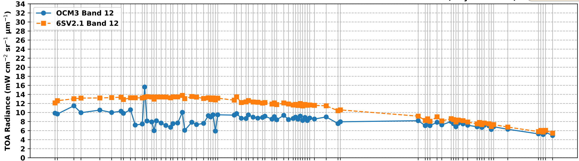
OCM3 Band 12 vs 6S Simulated Band 12 TOA Radiance over RVUS RadCalNet Site (May-Nov 2025)
