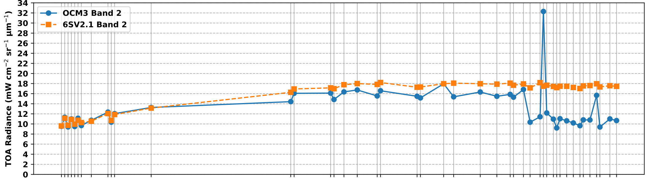
OCM3 Band 2 vs 6S Simulated Band 2 TOA Radiance over RVUS RadCalNet Site (Jan-Jun 2025)
