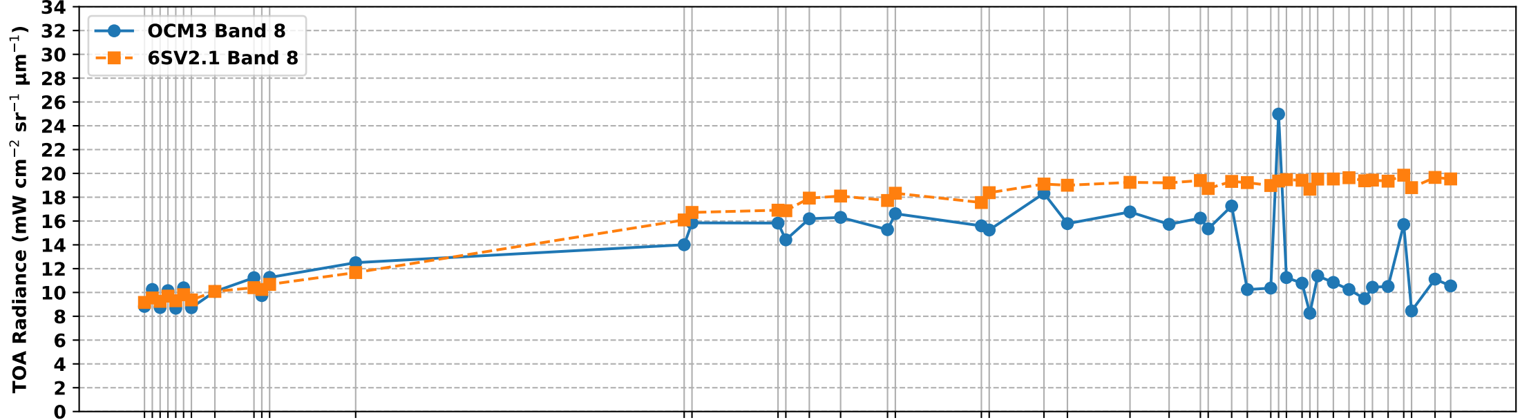
OCM3 Band 8 vs 6S Simulated Band 8 TOA Radiance over RVUS RadCalNet Site (Jan-Jun 2025)
