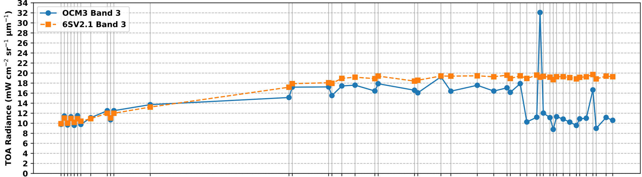
OCM3 Band 3 vs 6S Simulated Band 3 TOA Radiance over RVUS RadCalNet Site (Jan-Jun 2025)
