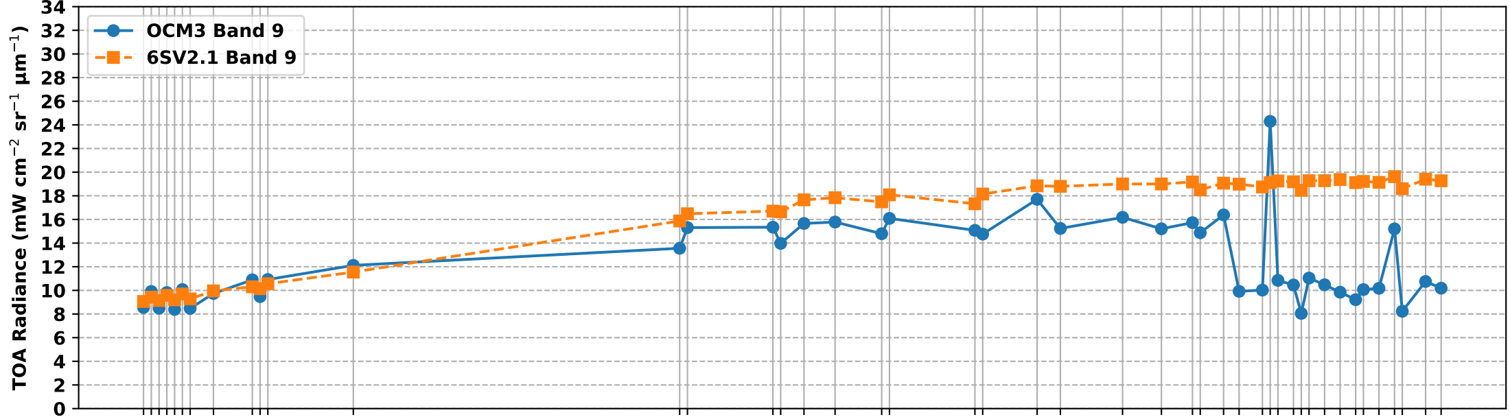
OCM3 Band 9 vs 6S Simulated Band 9 TOA Radiance over RVUS RadCalNet Site (Jan-Jun 2025)
