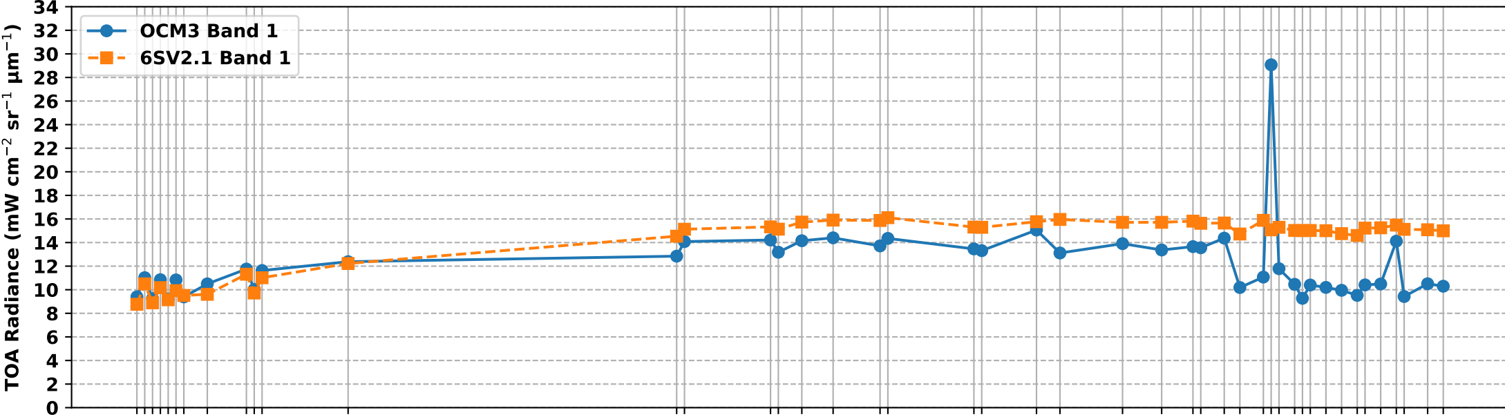
OCM3 Band 1 vs 6S Simulated Band 1 TOA Radiance over RVUS RadCalNet Site (Jan-Jun 2025)
