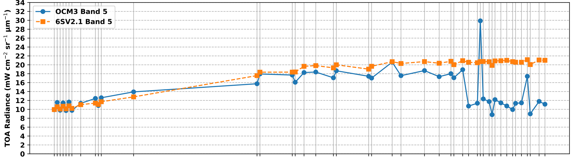
OCM3 Band 5 vs 6S Simulated Band 5 TOA Radiance over RVUS RadCalNet Site (Jan-Jun 2025)
