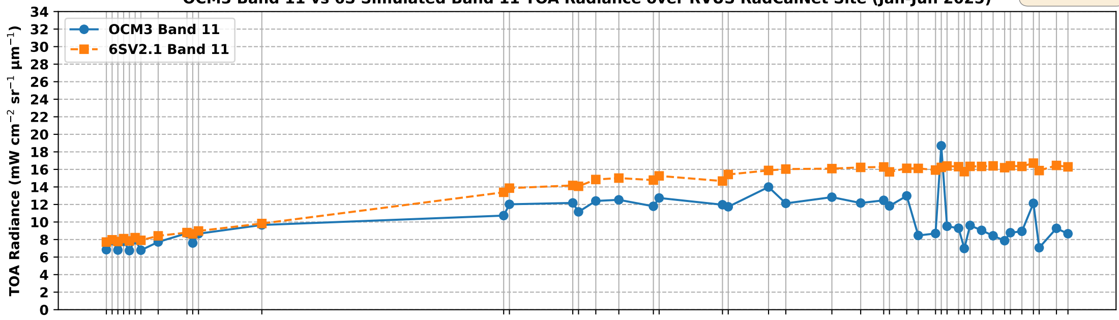
OCM3 Band 11 vs 6S Simulated Band 11 TOA Radiance over RVUS RadCalNet Site (Jan-Jun 2025)
