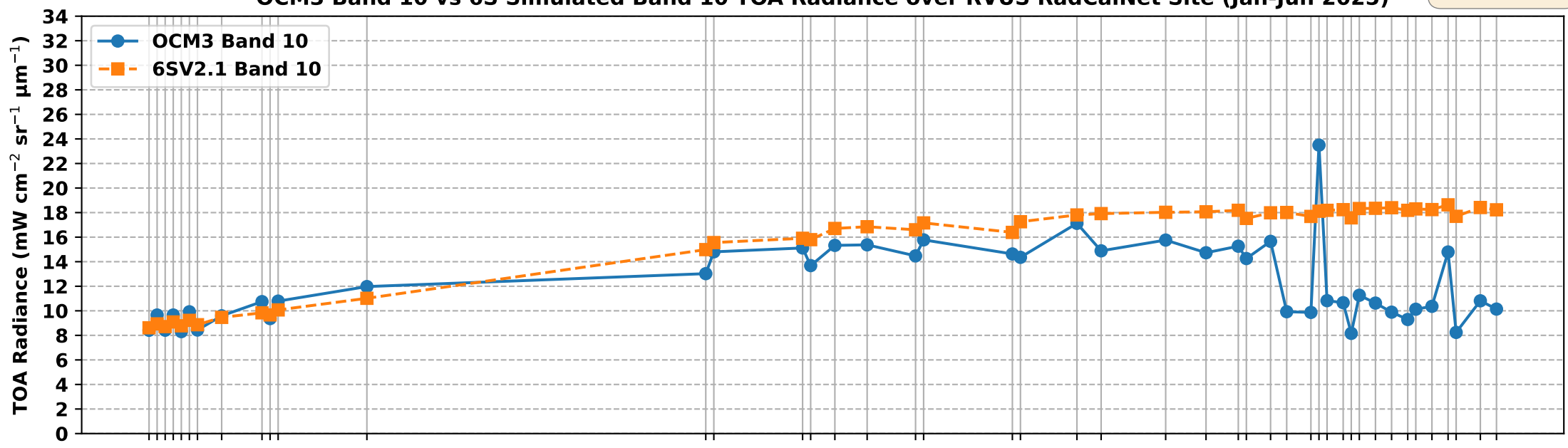
OCM3 Band 10 vs 6S Simulated Band 10 TOA Radiance over RVUS RadCalNet Site (Jan-Jun 2025)
