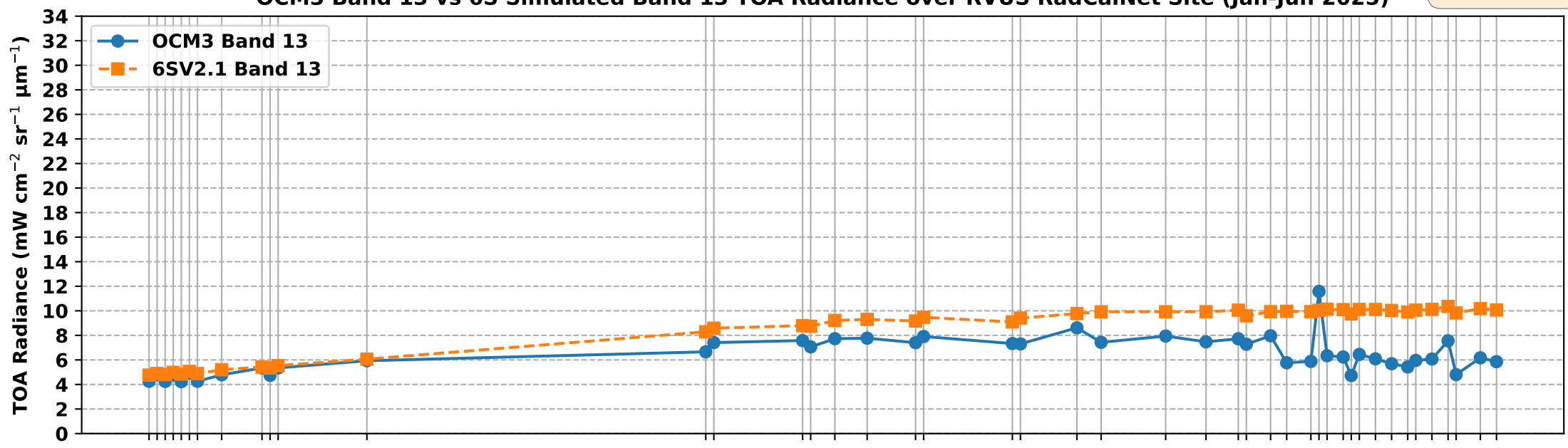
OCM3 Band 13 vs 6S Simulated Band 13 TOA Radiance over RVUS RadCalNet Site (Jan-Jun 2025)
