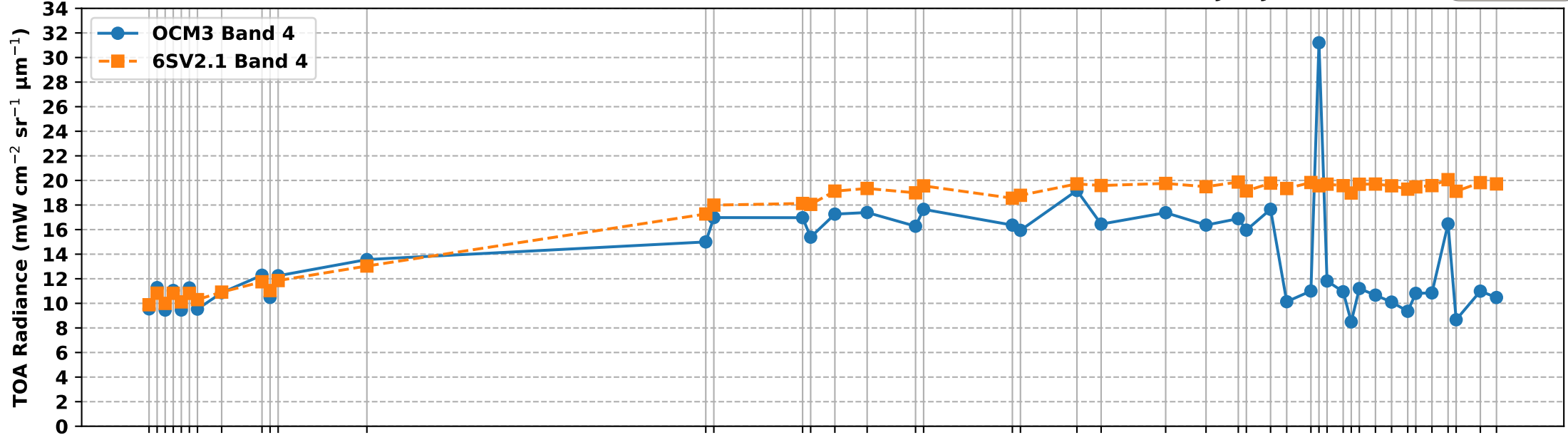
OCM3 Band 4 vs 6S Simulated Band 4 TOA Radiance over RVUS RadCalNet Site (Jan-Jun 2025)
