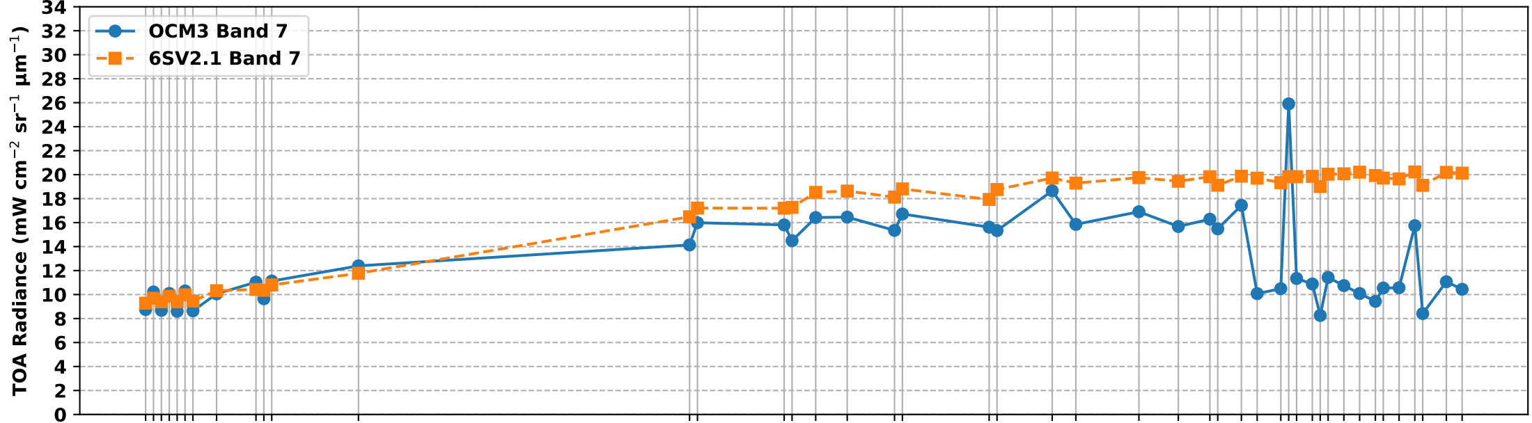
OCM3 Band 7 vs 6S Simulated Band 7 TOA Radiance over RVUS RadCalNet Site (Jan-Jun 2025)
