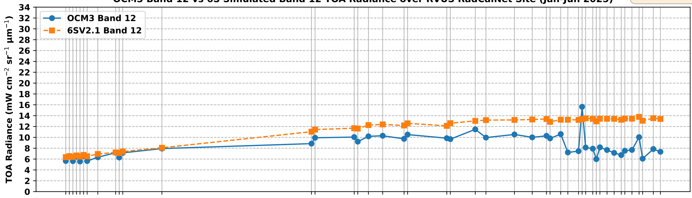
OCM3 Band 12 vs 6S Simulated Band 12 TOA Radiance over RVUS RadCalNet Site (Jan-Jun 2025)
