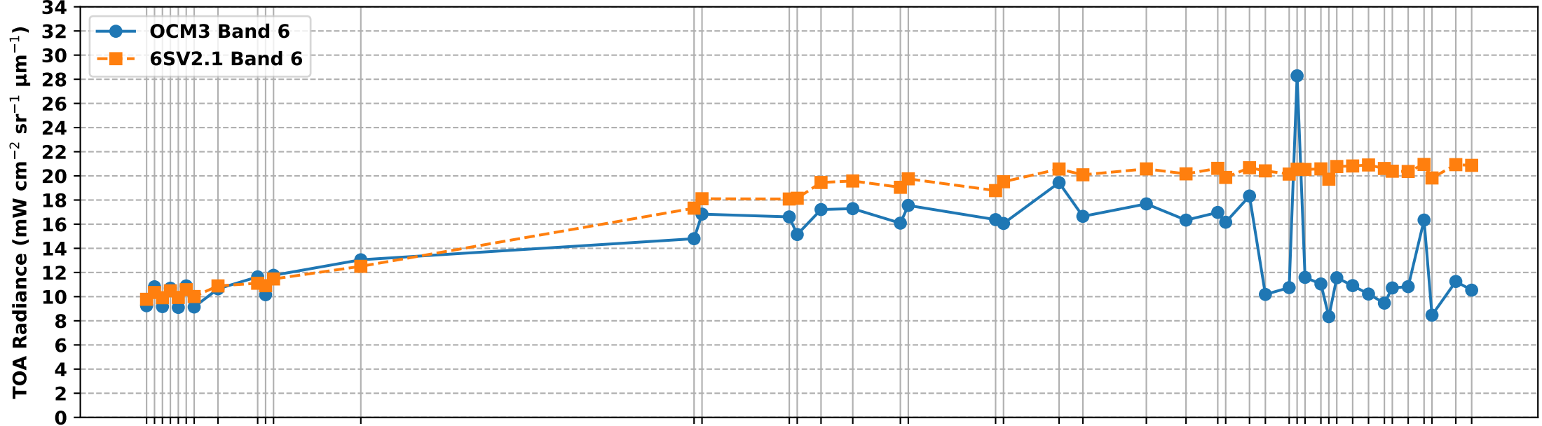
OCM3 Band 6 vs 6S Simulated Band 6 TOA Radiance over RVUS RadCalNet Site (Jan-Jun 2025)
