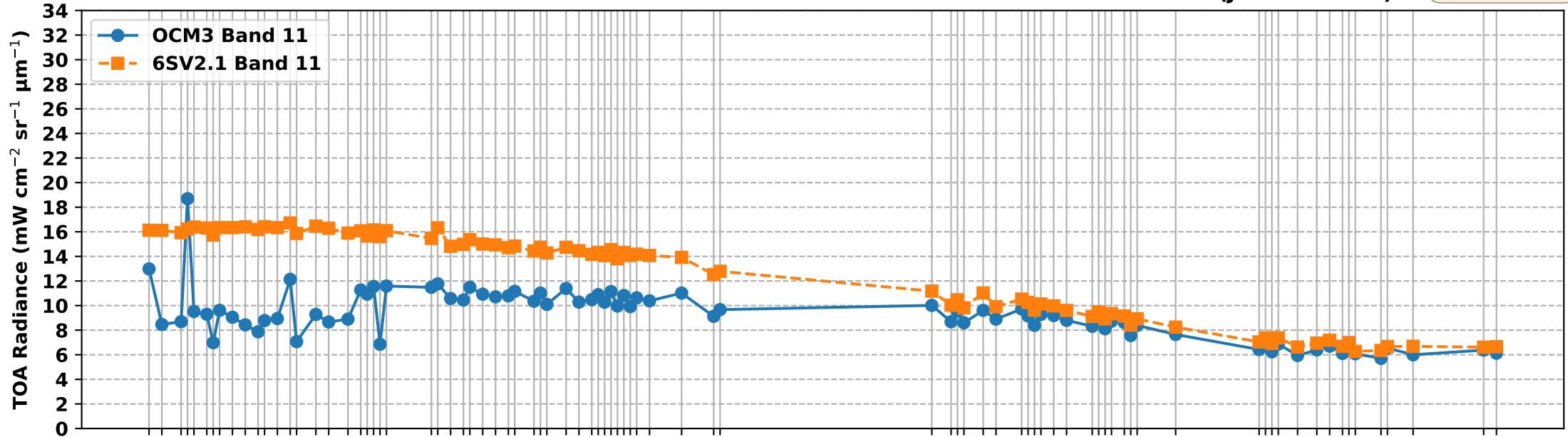
OCM3 Band 11 vs 6S Simulated Band 11 TOA Radiance over RVUS RadCalNet Site (Jun-Dec 2025)
