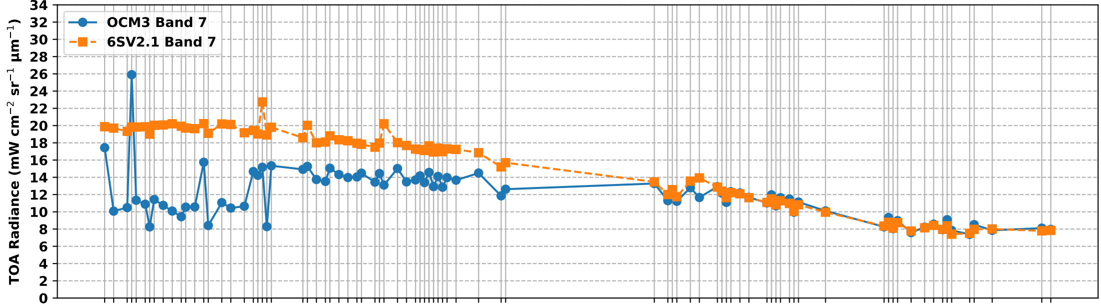
OCM3 Band 7 vs 6S Simulated Band 7 TOA Radiance over RVUS RadCalNet Site (Jun-Dec 2025)
