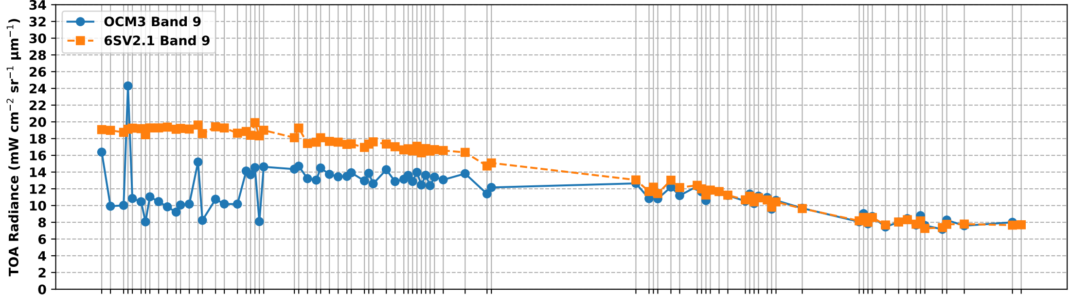
OCM3 Band 9 vs 6S Simulated Band 9 TOA Radiance over RVUS RadCalNet Site (Jun-Dec 2025)
