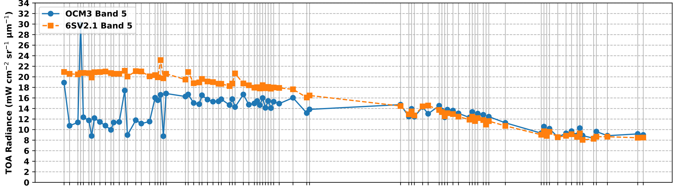
OCM3 Band 5 vs 6S Simulated Band 5 TOA Radiance over RVUS RadCalNet Site (Jun-Dec 2025)
