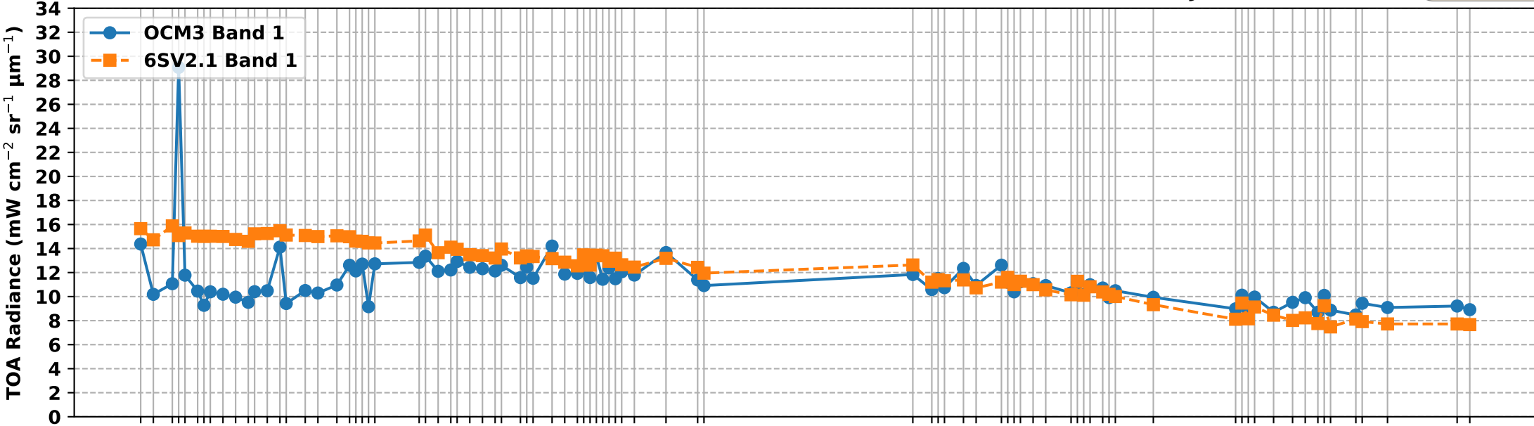
OCM3 Band 1 vs 6S Simulated Band 1 TOA Radiance over RVUS RadCalNet Site (Jun-Dec 2025)
