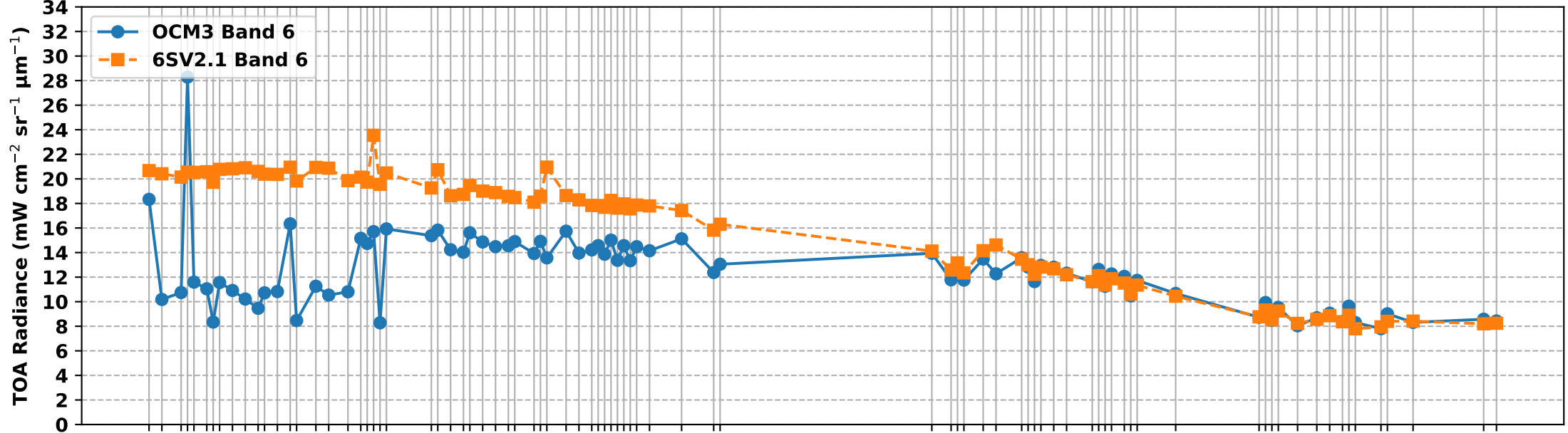
OCM3 Band 6 vs 6S Simulated Band 6 TOA Radiance over RVUS RadCalNet Site (Jun-Dec 2025)
