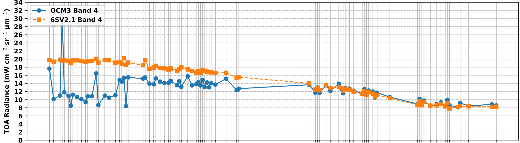
OCM3 Band 4 vs 6S Simulated Band 4 TOA Radiance over RVUS RadCalNet Site (Jun-Dec 2025)
