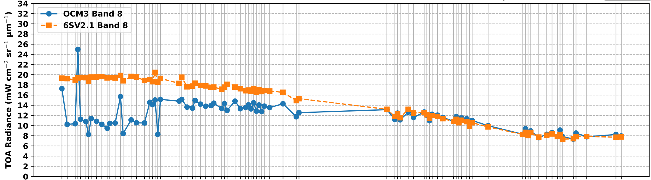
OCM3 Band 8 vs 6S Simulated Band 8 TOA Radiance over RVUS RadCalNet Site (Jun-Dec 2025)
