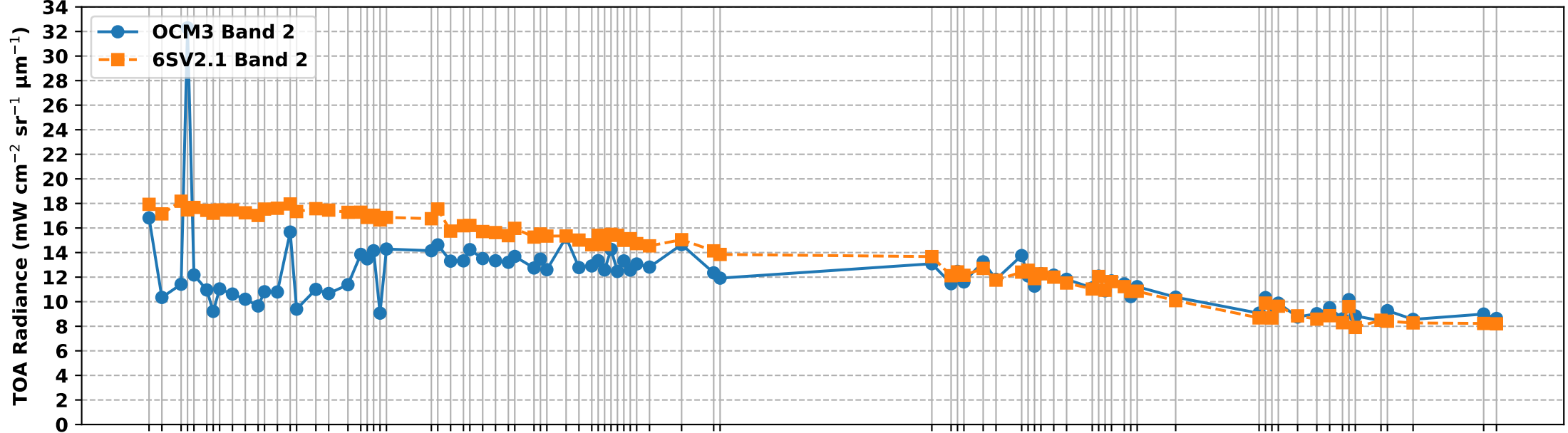
OCM3 Band 2 vs 6S Simulated Band 2 TOA Radiance over RVUS RadCalNet Site (Jun-Dec 2025)
