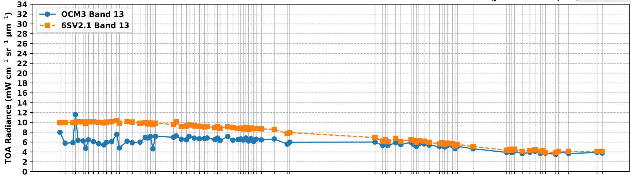
OCM3 Band 13 vs 6S Simulated Band 13 TOA Radiance over RVUS RadCalNet Site (Jun-Dec 2025)
