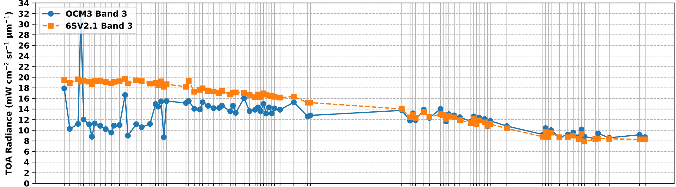
OCM3 Band 3 vs 6S Simulated Band 3 TOA Radiance over RVUS RadCalNet Site (Jun-Dec 2025)
