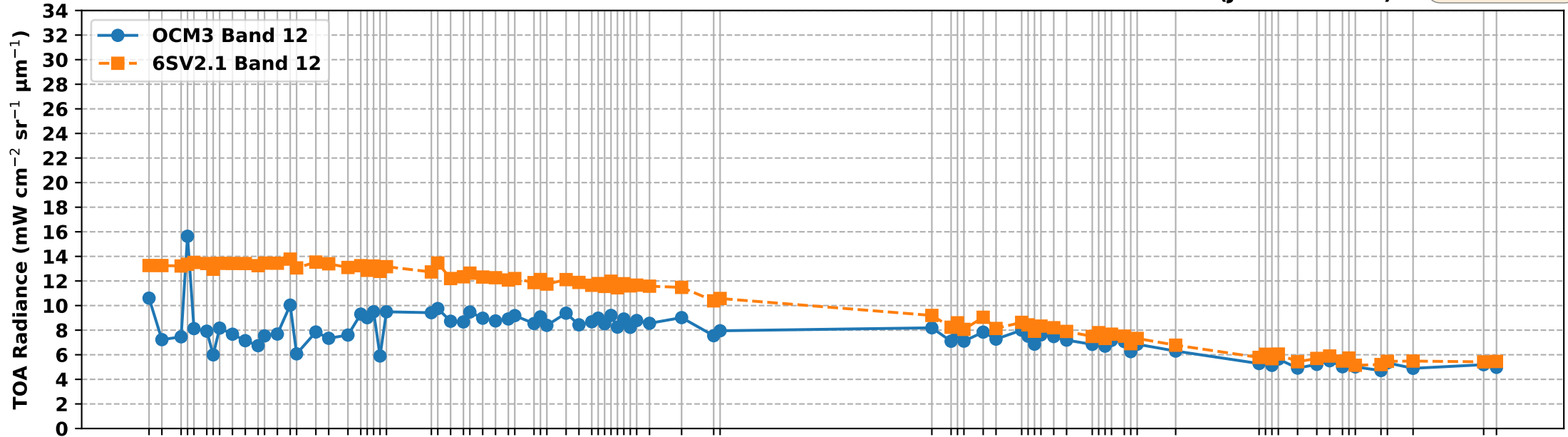
OCM3 Band 12 vs 6S Simulated Band 12 TOA Radiance over RVUS RadCalNet Site (Jun-Dec 2025)
