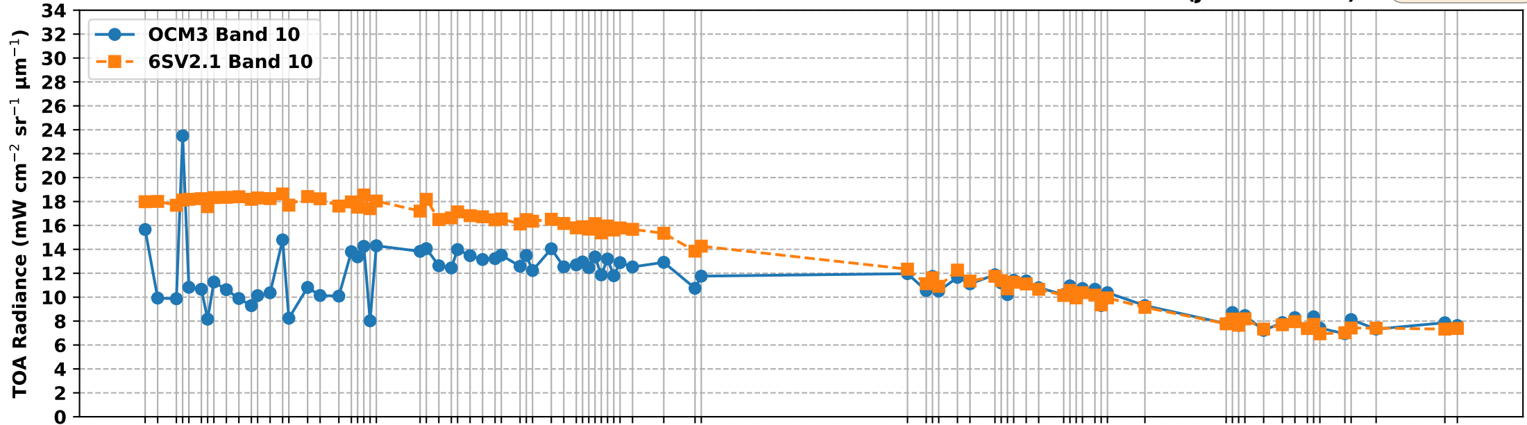
OCM3 Band 10 vs 6S Simulated Band 10 TOA Radiance over RVUS RadCalNet Site (Jun-Dec 2025)
