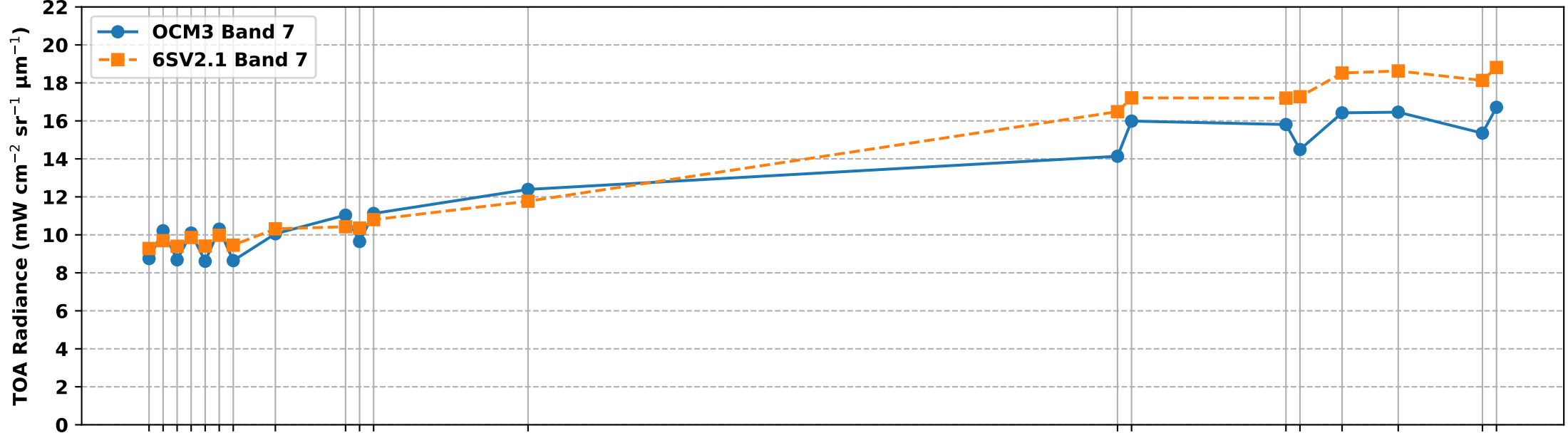
OCM3 Band 7 vs 6S Simulated Band 7 TOA Radiance over RVUS RadCalNet Site (Jan-Apr 2025)
