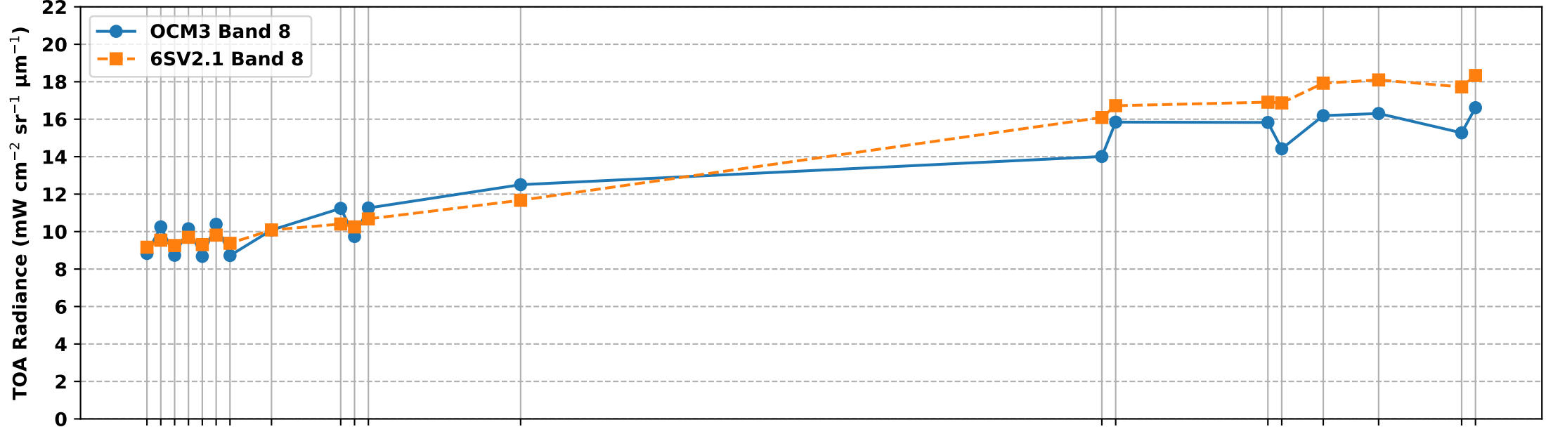
OCM3 Band 8 vs 6S Simulated Band 8 TOA Radiance over RVUS RadCalNet Site (Jan-Apr 2025)
