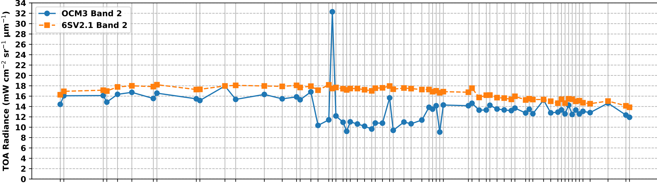
OCM3 Band 2 vs 6S Simulated Band 2 TOA Radiance over RVUS RadCalNet Site (Mar-Aug 2025)
