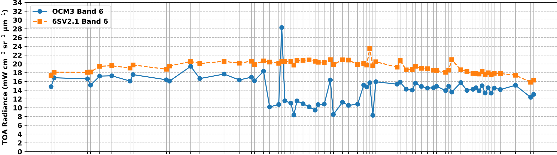
OCM3 Band 6 vs 6S Simulated Band 6 TOA Radiance over RVUS RadCalNet Site (Mar-Aug 2025)
