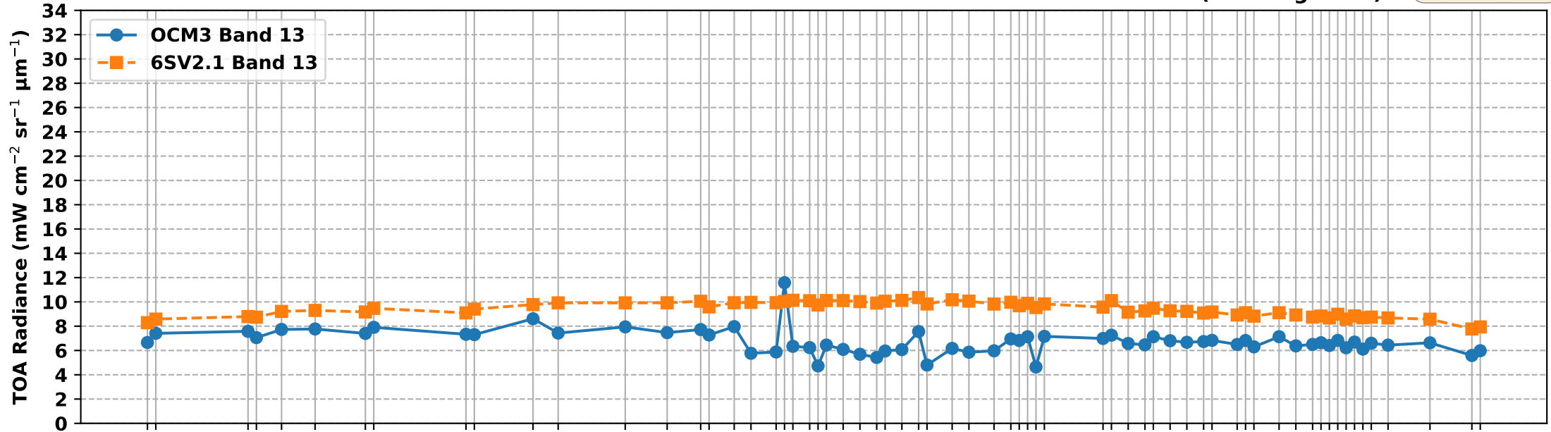
OCM3 Band 13 vs 6S Simulated Band 13 TOA Radiance over RVUS RadCalNet Site (Mar-Aug 2025)
