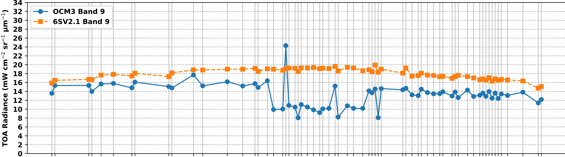
OCM3 Band 9 vs 6S Simulated Band 9 TOA Radiance over RVUS RadCalNet Site (Mar-Aug 2025)
