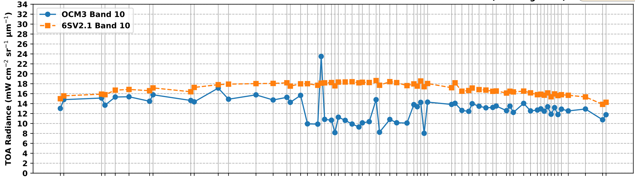
OCM3 Band 10 vs 6S Simulated Band 10 TOA Radiance over RVUS RadCalNet Site (Mar-Aug 2025)
