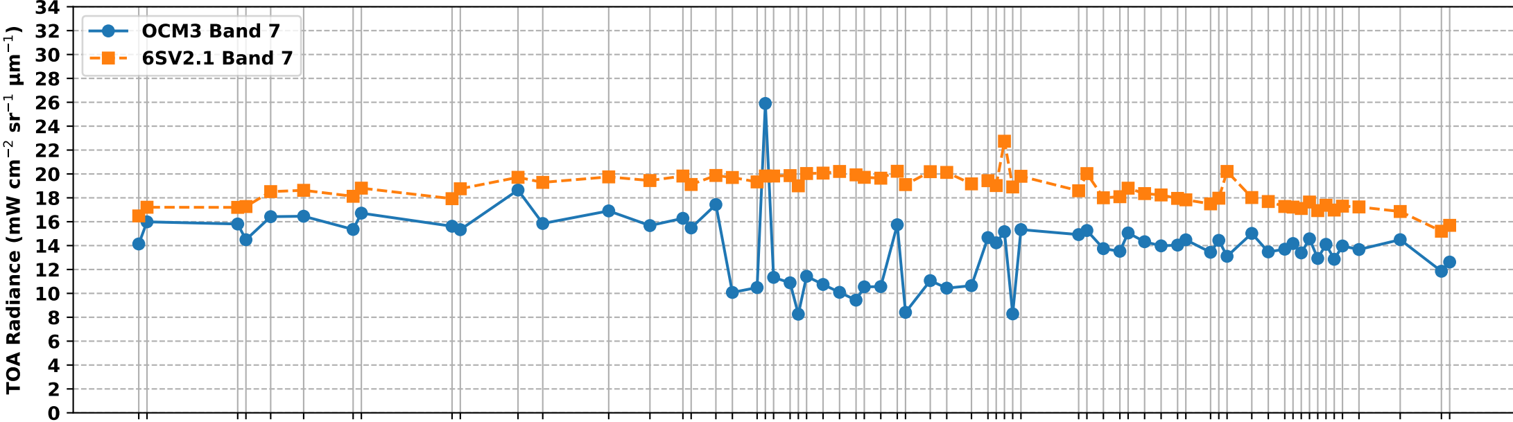
OCM3 Band 7 vs 6S Simulated Band 7 TOA Radiance over RVUS RadCalNet Site (Mar-Aug 2025)
