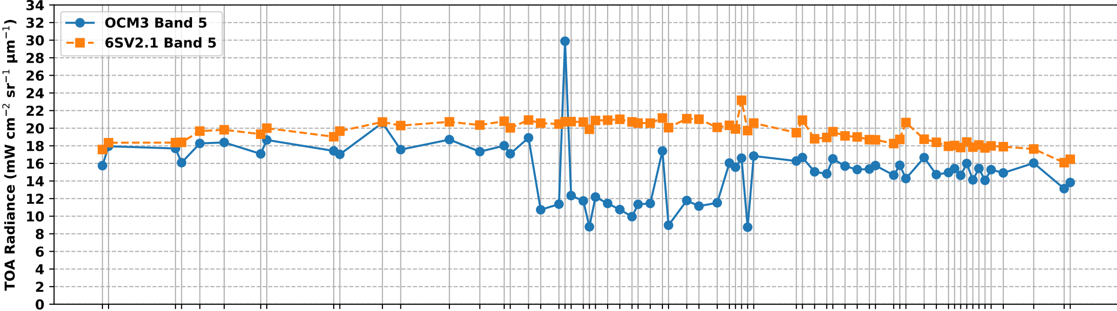
OCM3 Band 5 vs 6S Simulated Band 5 TOA Radiance over RVUS RadCalNet Site (Mar-Aug 2025)
