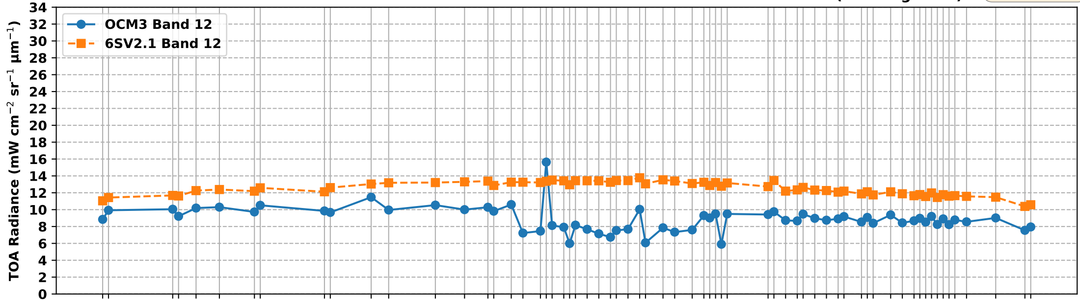
OCM3 Band 12 vs 6S Simulated Band 12 TOA Radiance over RVUS RadCalNet Site (Mar-Aug 2025)
