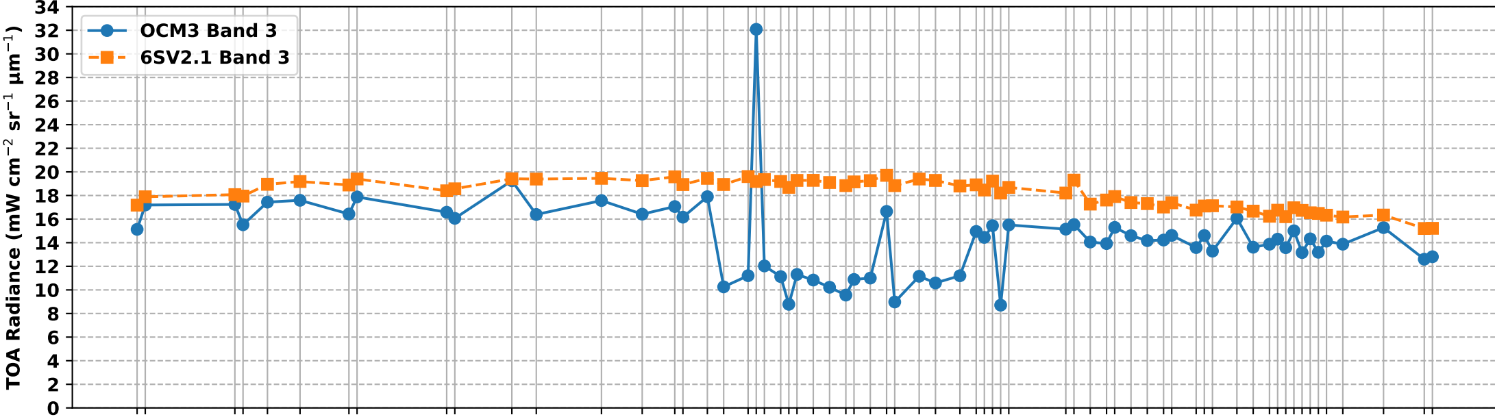
OCM3 Band 3 vs 6S Simulated Band 3 TOA Radiance over RVUS RadCalNet Site (Mar-Aug 2025)
