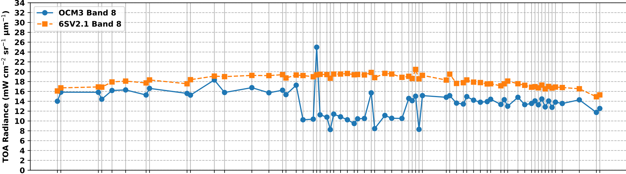
OCM3 Band 8 vs 6S Simulated Band 8 TOA Radiance over RVUS RadCalNet Site (Mar-Aug 2025)
