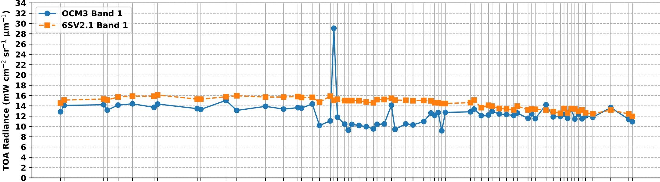
OCM3 Band 1 vs 6S Simulated Band 1 TOA Radiance over RVUS RadCalNet Site (Mar-Aug 2025)
