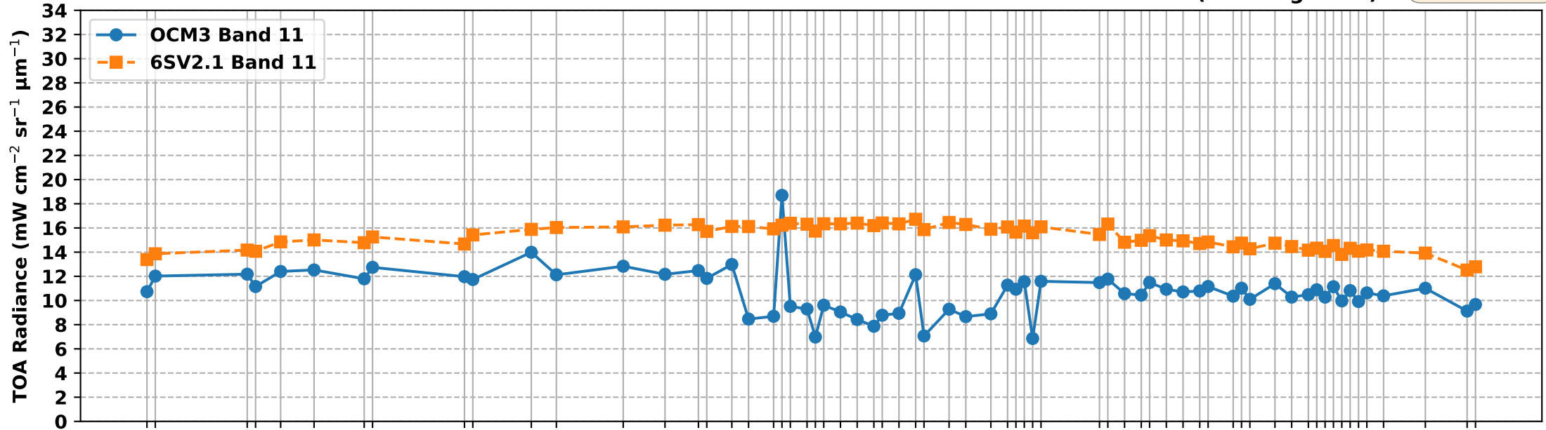
OCM3 Band 11 vs 6S Simulated Band 11 TOA Radiance over RVUS RadCalNet Site (Mar-Aug 2025)
