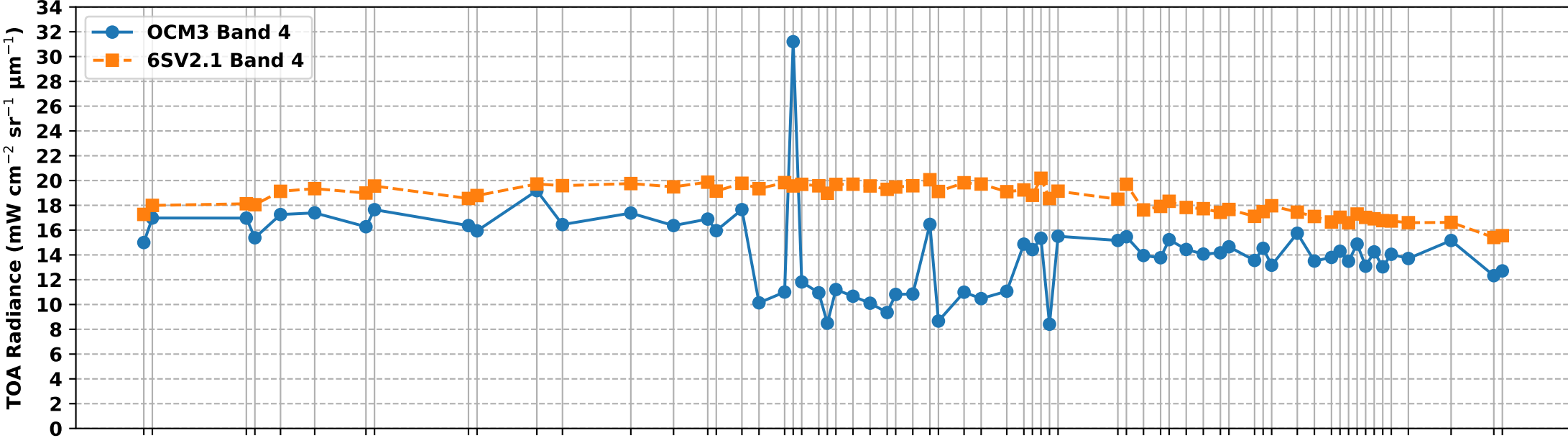
OCM3 Band 4 vs 6S Simulated Band 4 TOA Radiance over RVUS RadCalNet Site (Mar-Aug 2025)
