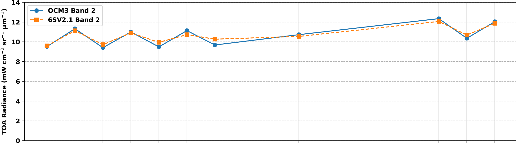
OCM3 Band 2 vs 6S Simulated Band 2 TOA Radiance over RVUS RadCalNet Site (Jan-Jan 2025)
