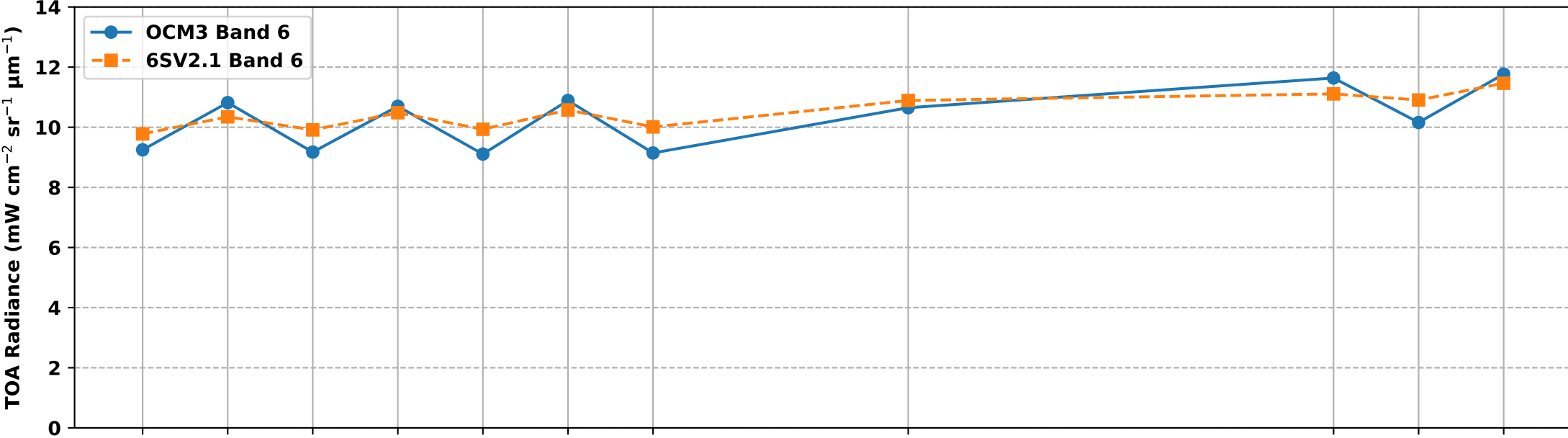
OCM3 Band 6 vs 6S Simulated Band 6 TOA Radiance over RVUS RadCalNet Site (Jan-Jan 2025)
