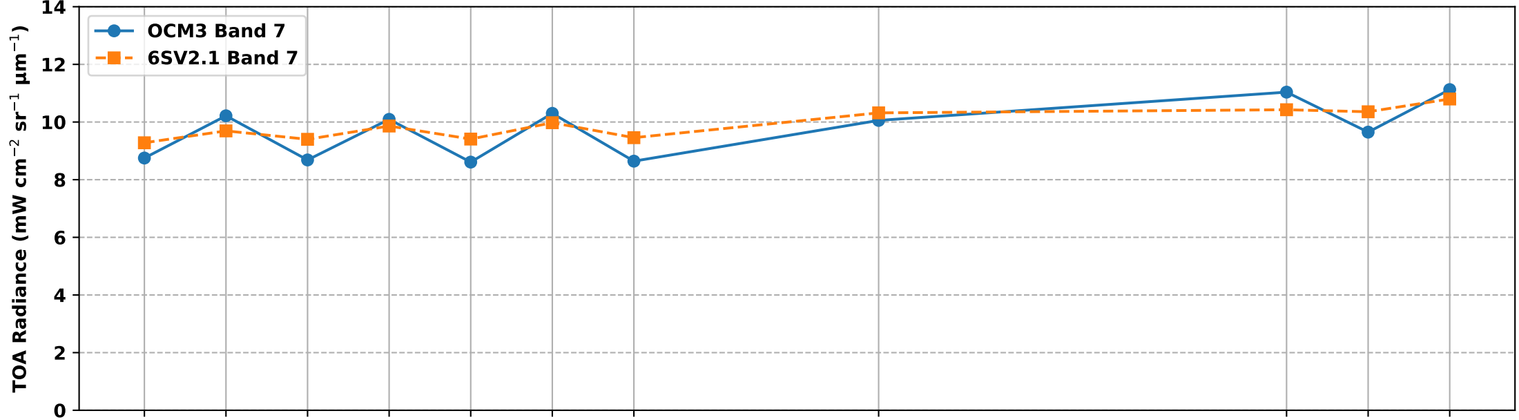
OCM3 Band 7 vs 6S Simulated Band 7 TOA Radiance over RVUS RadCalNet Site (Jan-Jan 2025)
