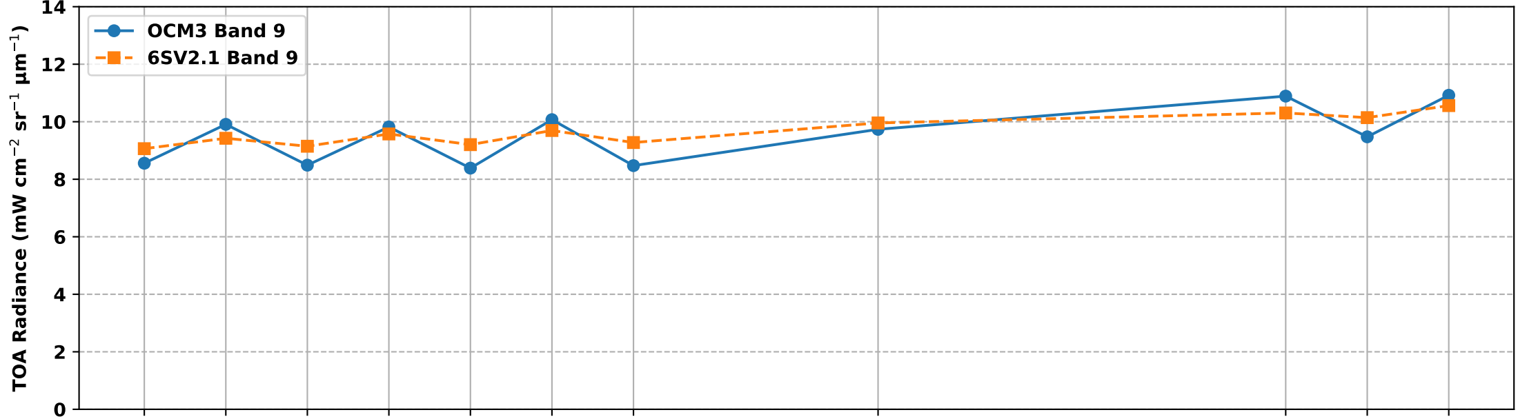
OCM3 Band 9 vs 6S Simulated Band 9 TOA Radiance over RVUS RadCalNet Site (Jan-Jan 2025)
