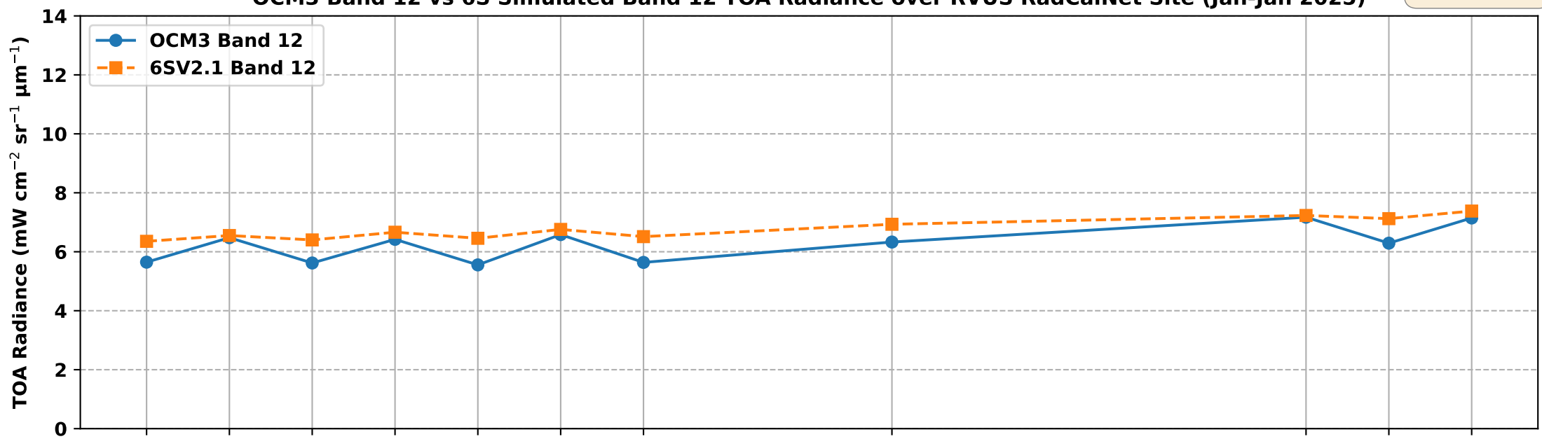
OCM3 Band 12 vs 6S Simulated Band 12 TOA Radiance over RVUS RadCalNet Site (Jan-Jan 2025)
