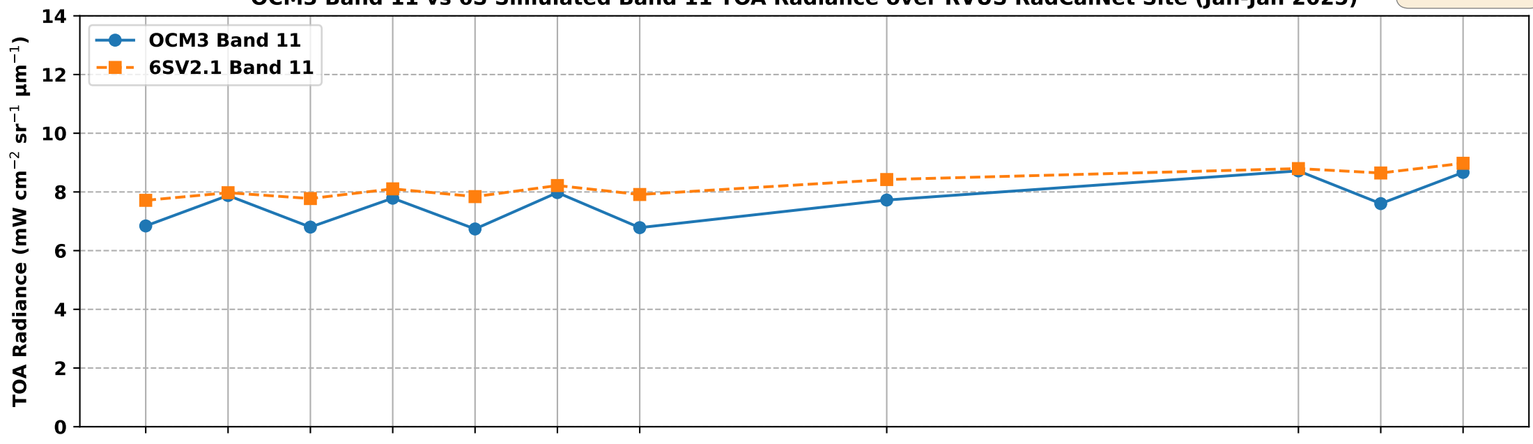
OCM3 Band 11 vs 6S Simulated Band 11 TOA Radiance over RVUS RadCalNet Site (Jan-Jan 2025)
