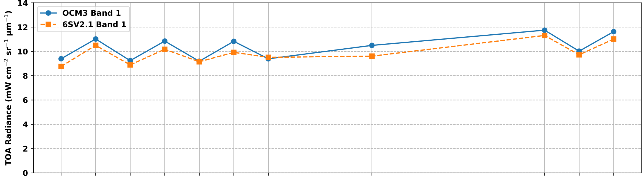
OCM3 Band 1 vs 6S Simulated Band 1 TOA Radiance over RVUS RadCalNet Site (Jan-Jan 2025)
