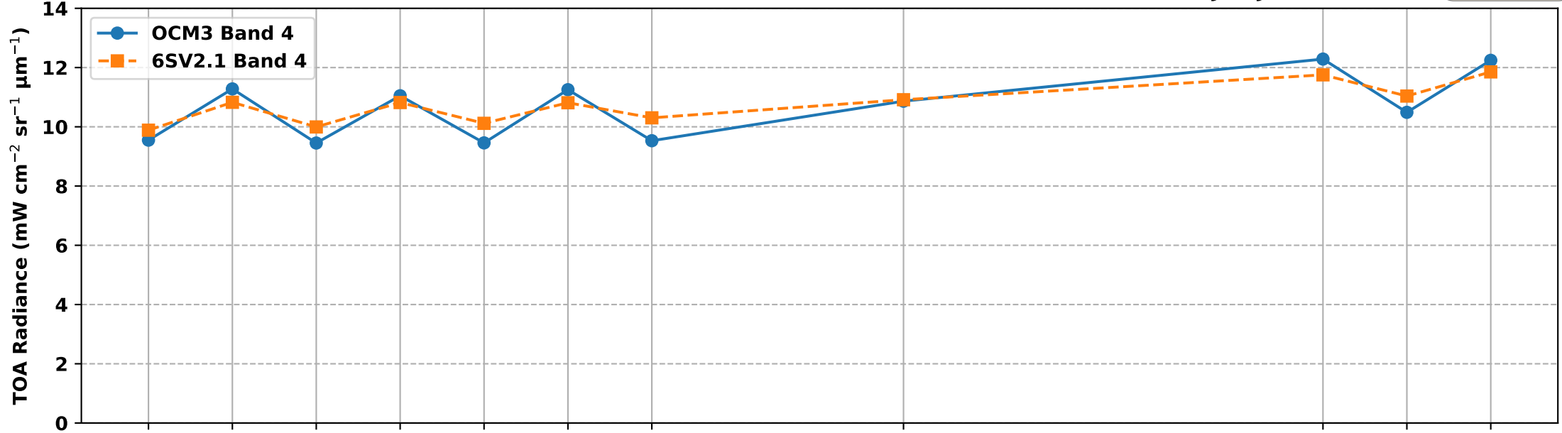
OCM3 Band 4 vs 6S Simulated Band 4 TOA Radiance over RVUS RadCalNet Site (Jan-Jan 2025)
