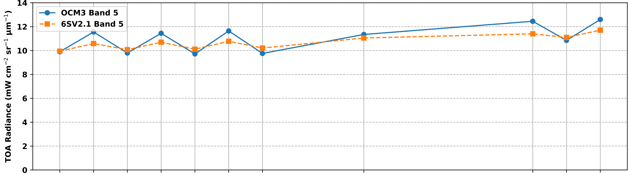
OCM3 Band 5 vs 6S Simulated Band 5 TOA Radiance over RVUS RadCalNet Site (Jan-Jan 2025)
