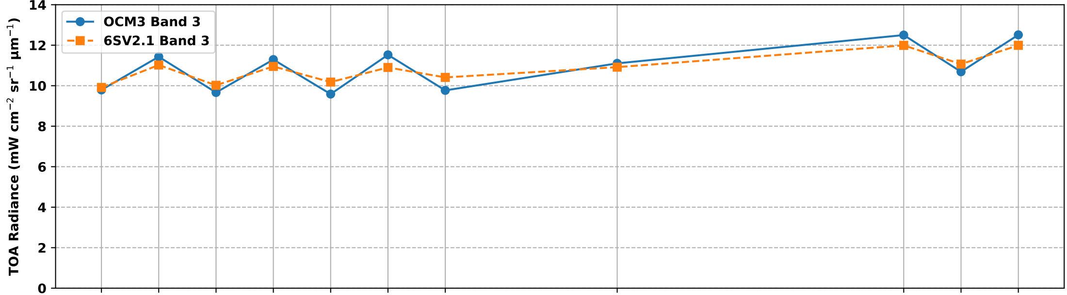
OCM3 Band 3 vs 6S Simulated Band 3 TOA Radiance over RVUS RadCalNet Site (Jan-Jan 2025)
