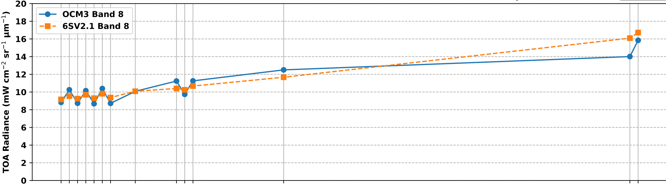
OCM3 Band 8 vs 6S Simulated Band 8 TOA Radiance over RVUS RadCalNet Site (Jan-Mar 2025)
