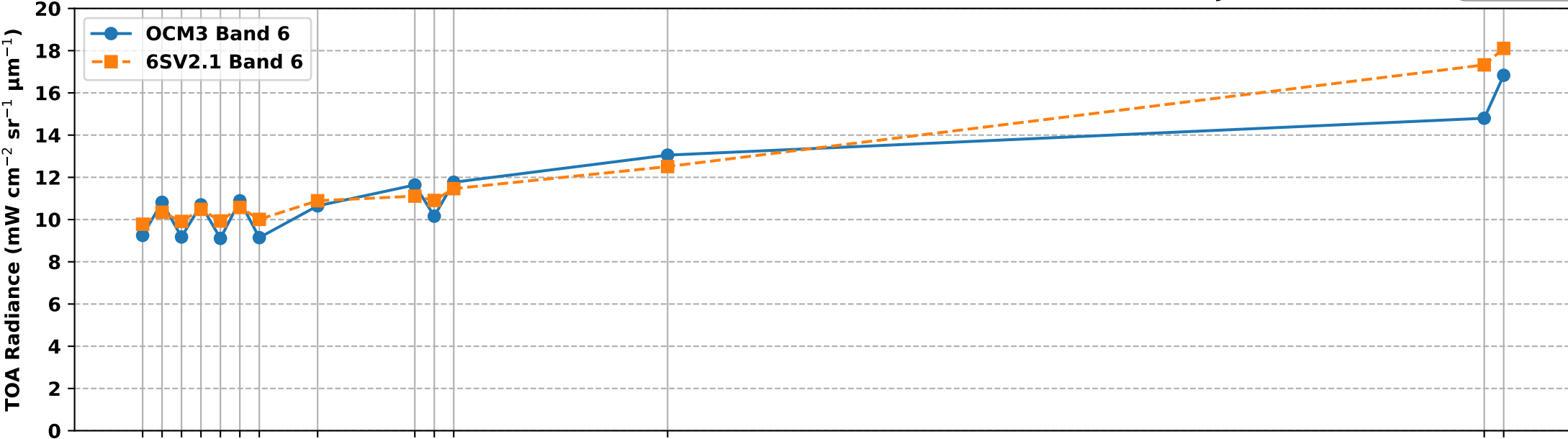
OCM3 Band 6 vs 6S Simulated Band 6 TOA Radiance over RVUS RadCalNet Site (Jan-Mar 2025)
