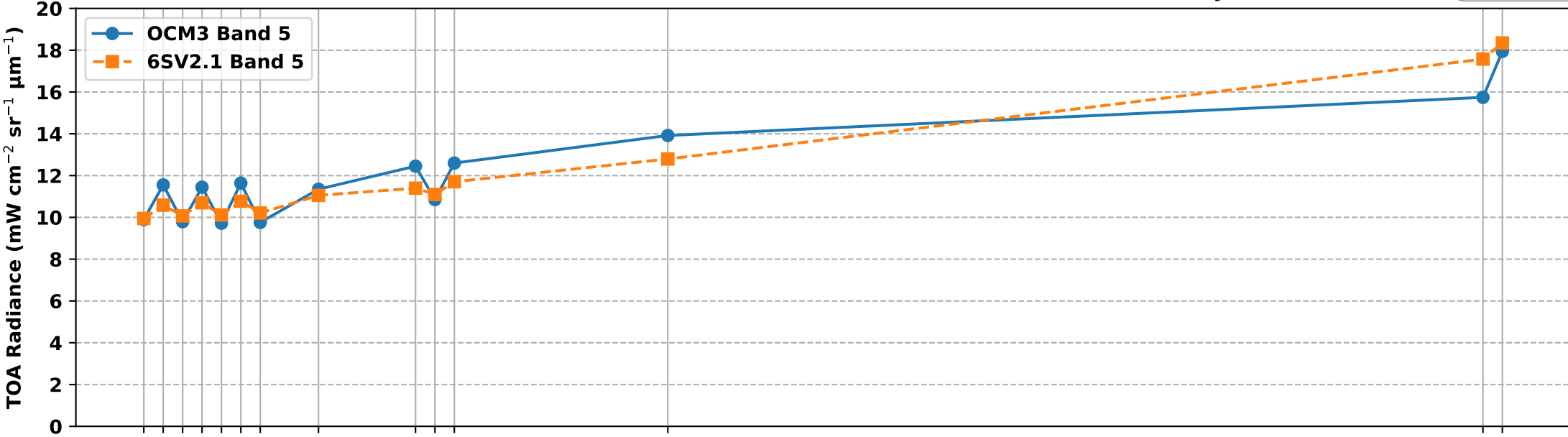
OCM3 Band 5 vs 6S Simulated Band 5 TOA Radiance over RVUS RadCalNet Site (Jan-Mar 2025)
