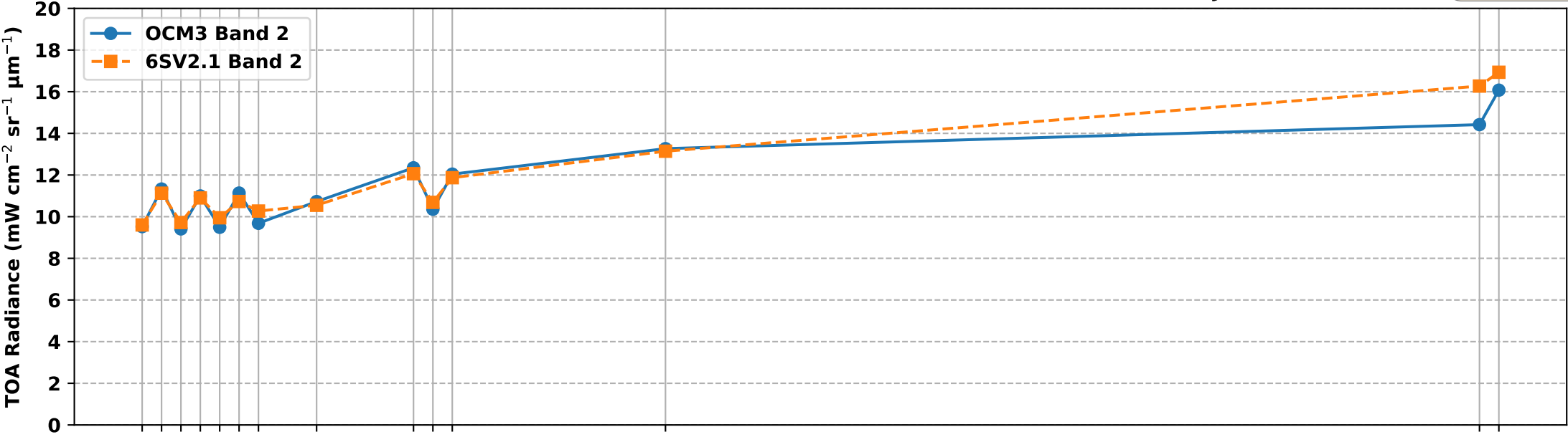
OCM3 Band 2 vs 6S Simulated Band 2 TOA Radiance over RVUS RadCalNet Site (Jan-Mar 2025)
