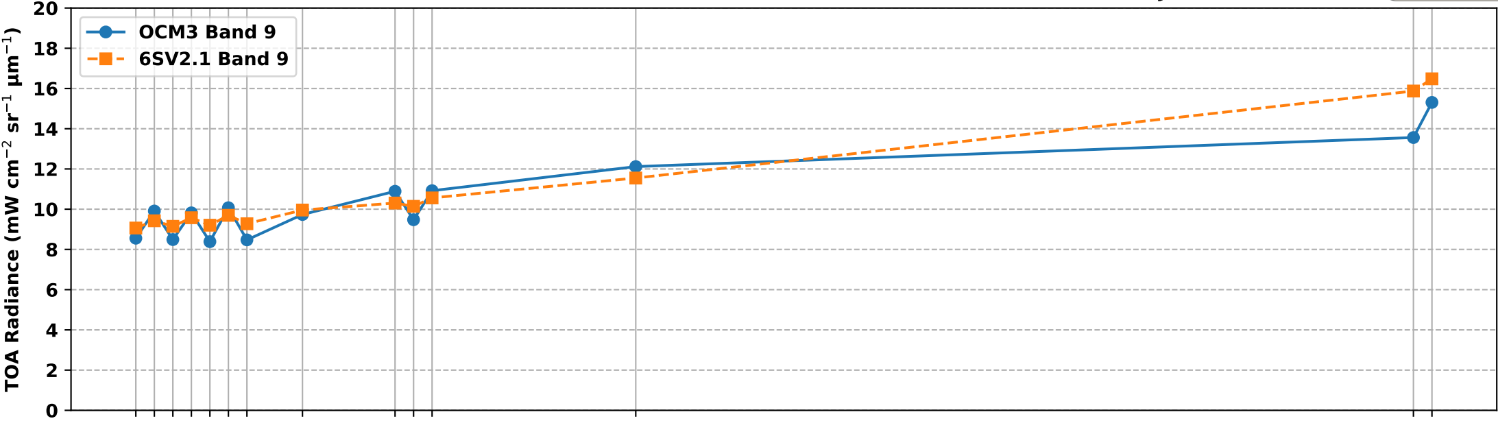
OCM3 Band 9 vs 6S Simulated Band 9 TOA Radiance over RVUS RadCalNet Site (Jan-Mar 2025)
