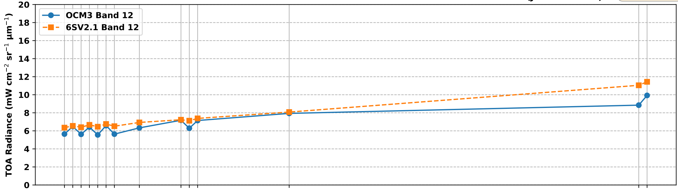
OCM3 Band 12 vs 6S Simulated Band 12 TOA Radiance over RVUS RadCalNet Site (Jan-Mar 2025)
