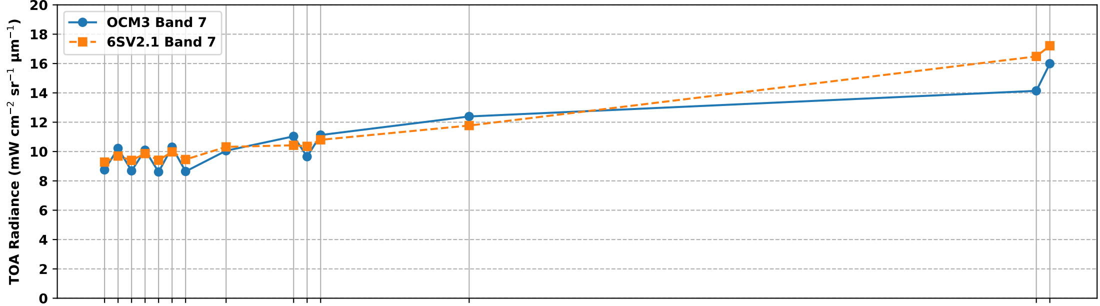
OCM3 Band 7 vs 6S Simulated Band 7 TOA Radiance over RVUS RadCalNet Site (Jan-Mar 2025)
