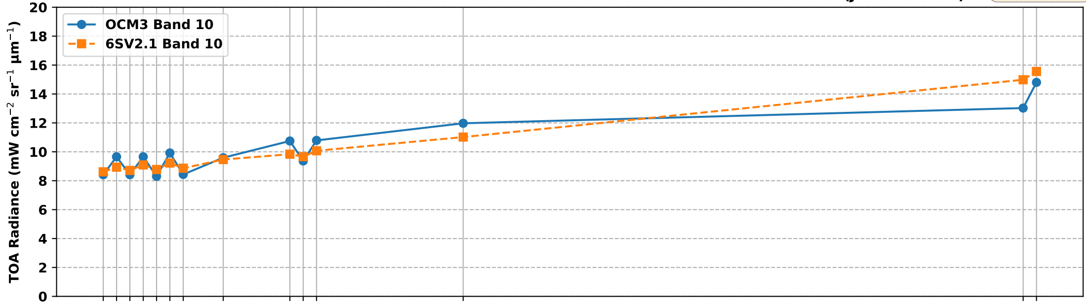
OCM3 Band 10 vs 6S Simulated Band 10 TOA Radiance over RVUS RadCalNet Site (Jan-Mar 2025)
