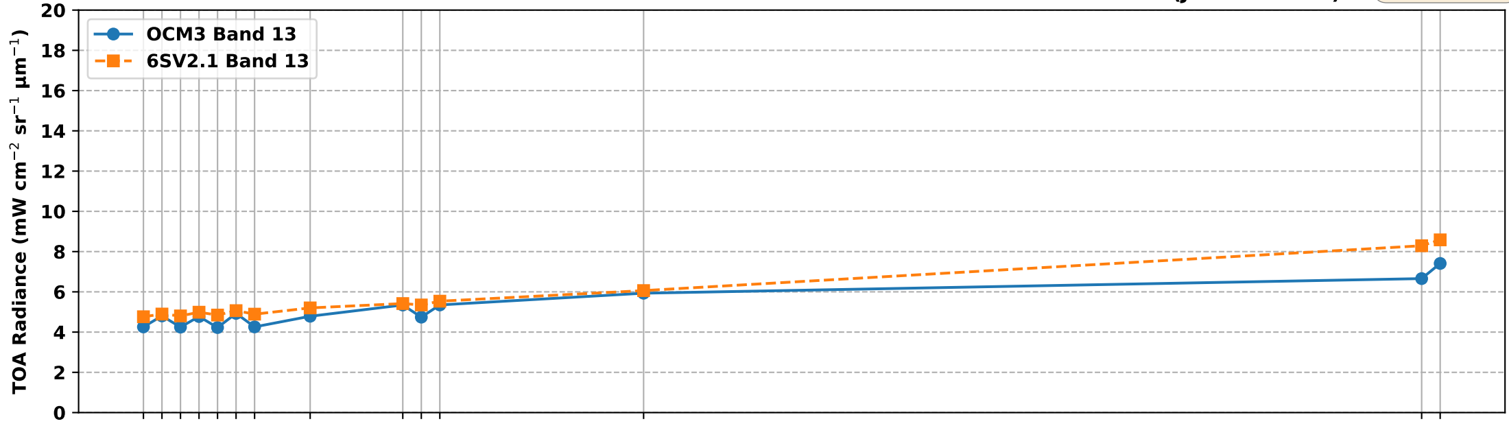
OCM3 Band 13 vs 6S Simulated Band 13 TOA Radiance over RVUS RadCalNet Site (Jan-Mar 2025)
