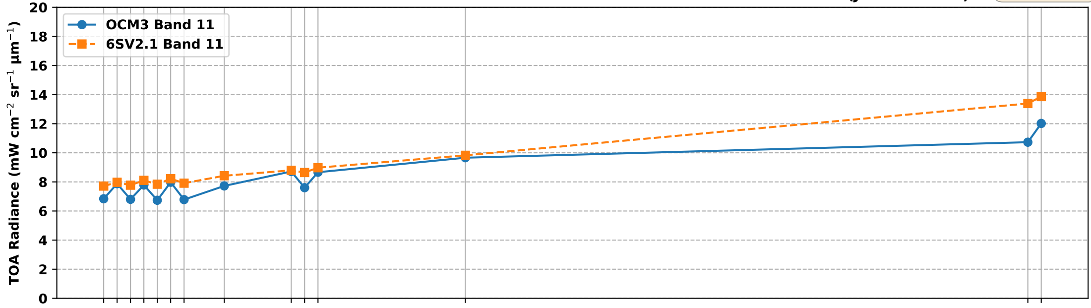
OCM3 Band 11 vs 6S Simulated Band 11 TOA Radiance over RVUS RadCalNet Site (Jan-Mar 2025)
