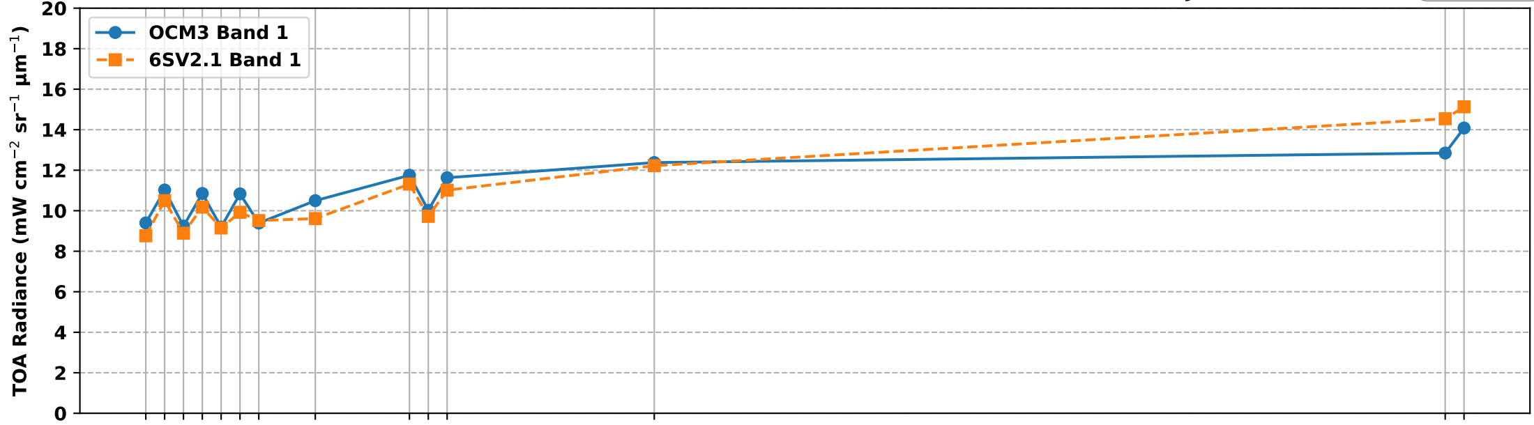
OCM3 Band 1 vs 6S Simulated Band 1 TOA Radiance over RVUS RadCalNet Site (Jan-Mar 2025)
