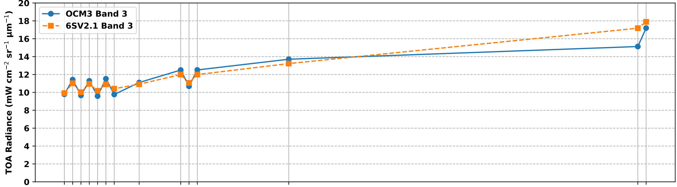
OCM3 Band 3 vs 6S Simulated Band 3 TOA Radiance over RVUS RadCalNet Site (Jan-Mar 2025)
