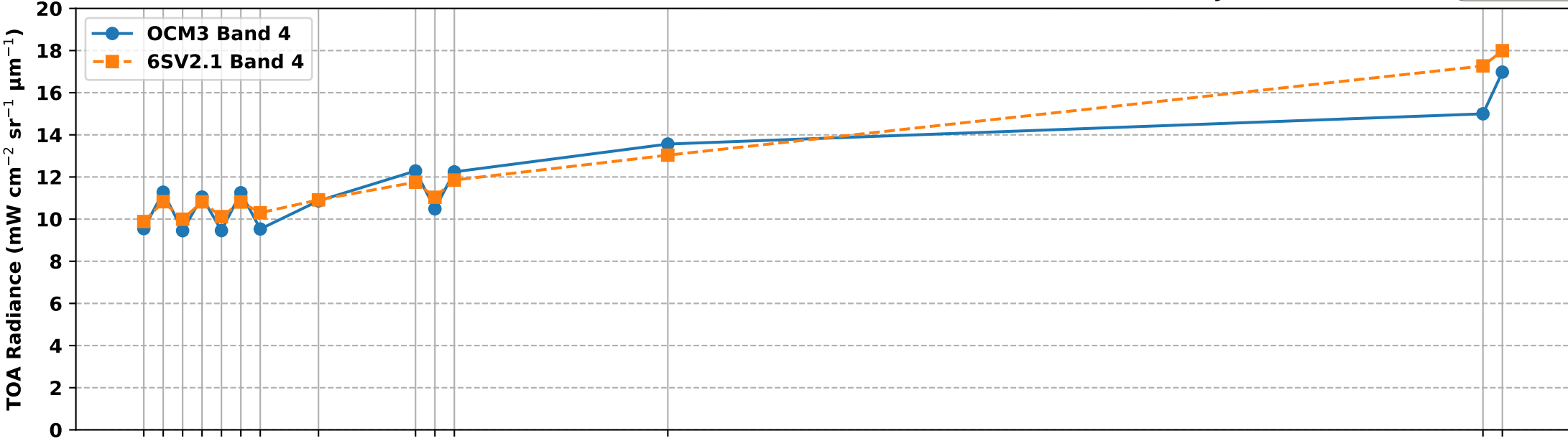
OCM3 Band 4 vs 6S Simulated Band 4 TOA Radiance over RVUS RadCalNet Site (Jan-Mar 2025)
