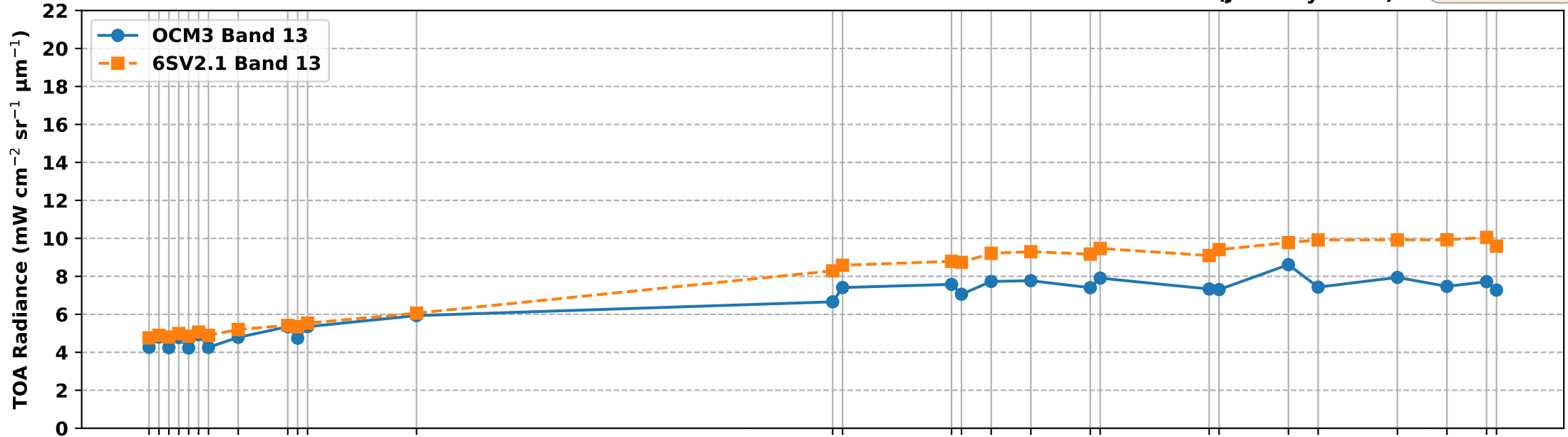
OCM3 Band 13 vs 6S Simulated Band 13 TOA Radiance over RVUS RadCalNet Site (Jan-May 2025)
