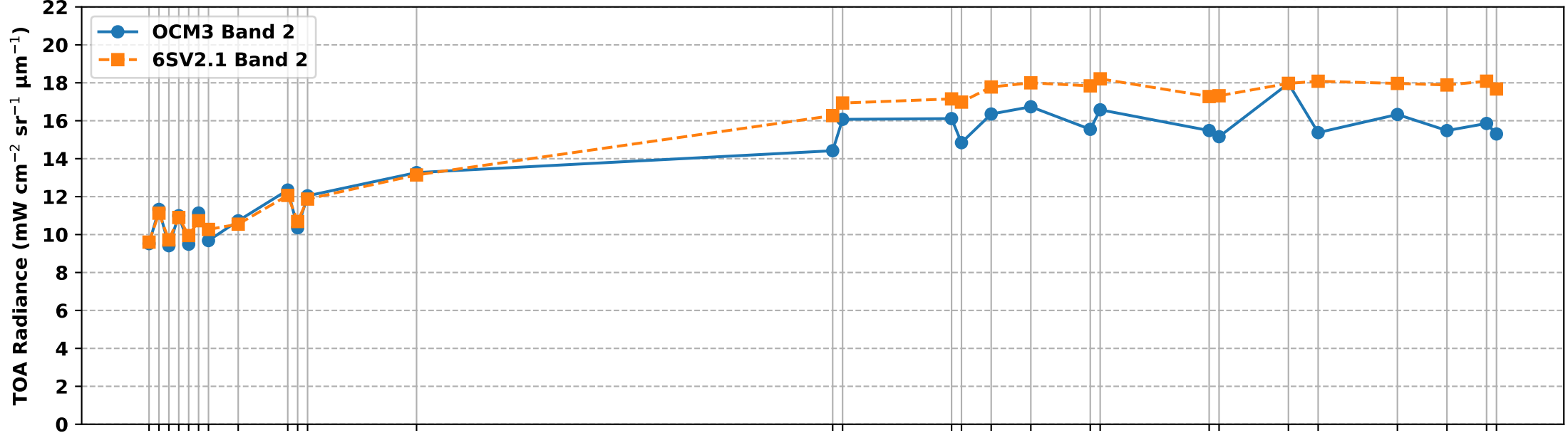
OCM3 Band 2 vs 6S Simulated Band 2 TOA Radiance over RVUS RadCalNet Site (Jan-May 2025)
