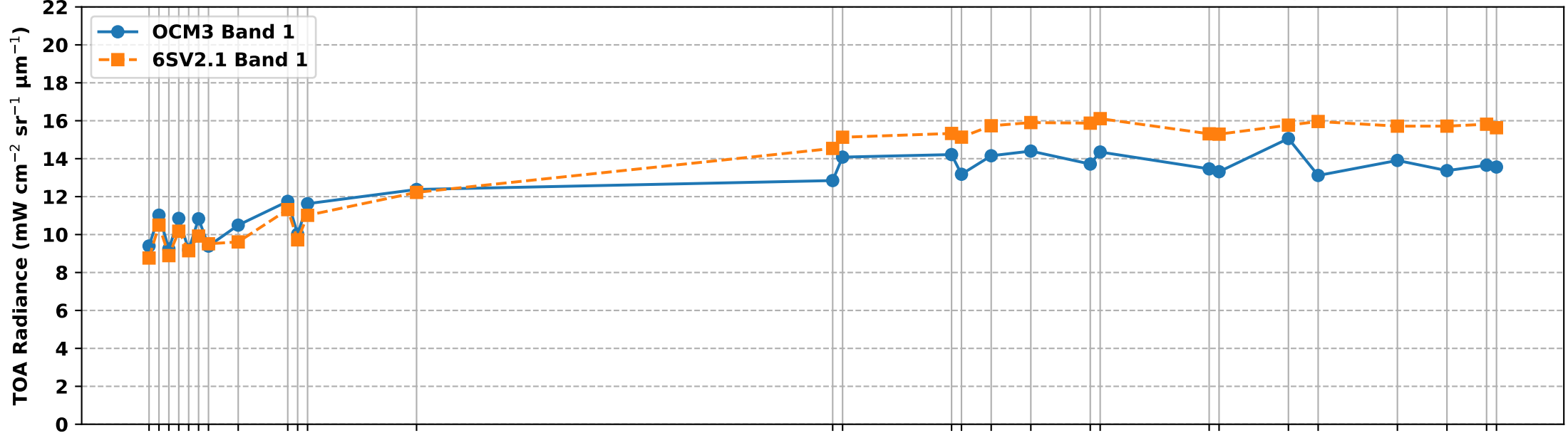
OCM3 Band 1 vs 6S Simulated Band 1 TOA Radiance over RVUS RadCalNet Site (Jan-May 2025)
