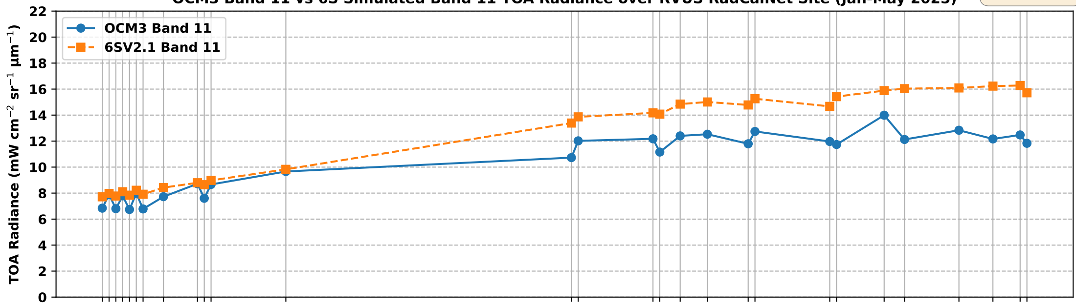
OCM3 Band 11 vs 6S Simulated Band 11 TOA Radiance over RVUS RadCalNet Site (Jan-May 2025)
