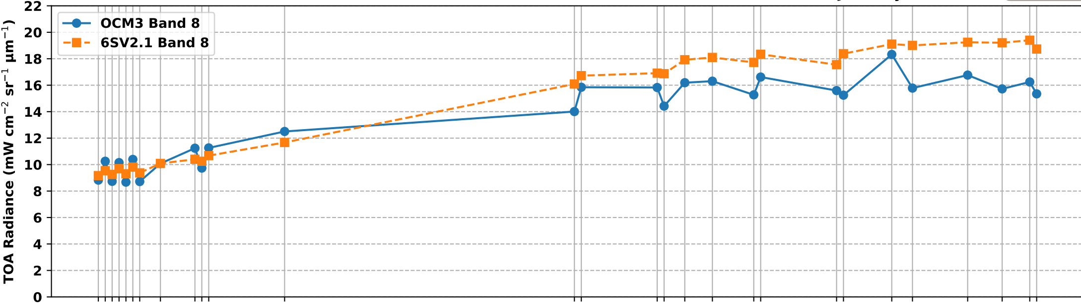
OCM3 Band 8 vs 6S Simulated Band 8 TOA Radiance over RVUS RadCalNet Site (Jan-May 2025)
