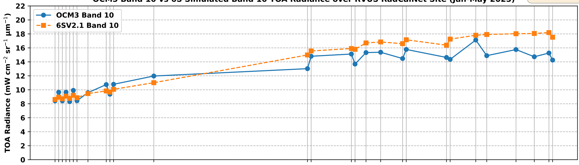
OCM3 Band 10 vs 6S Simulated Band 10 TOA Radiance over RVUS RadCalNet Site (Jan-May 2025)
