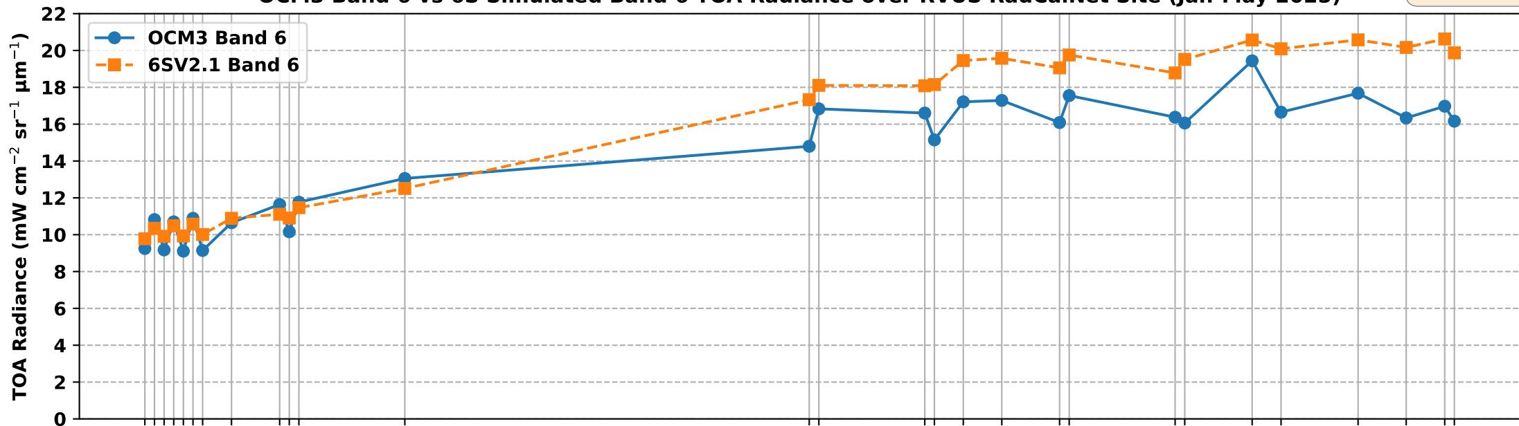
OCM3 Band 6 vs 6S Simulated Band 6 TOA Radiance over RVUS RadCalNet Site (Jan-May 2025)
