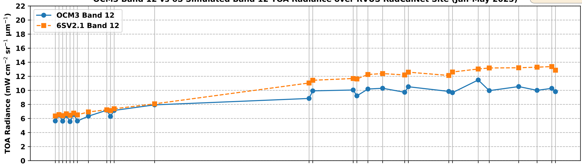
OCM3 Band 12 vs 6S Simulated Band 12 TOA Radiance over RVUS RadCalNet Site (Jan-May 2025)
