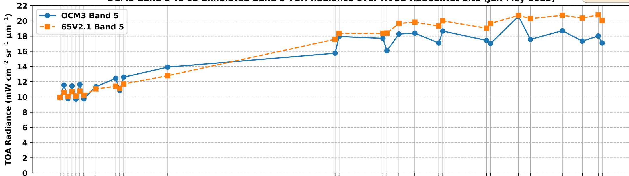
OCM3 Band 5 vs 6S Simulated Band 5 TOA Radiance over RVUS RadCalNet Site (Jan-May 2025)
