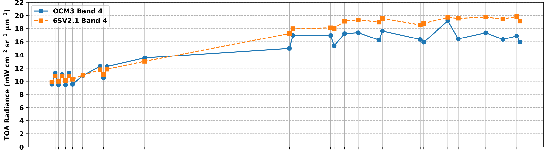
OCM3 Band 4 vs 6S Simulated Band 4 TOA Radiance over RVUS RadCalNet Site (Jan-May 2025)
