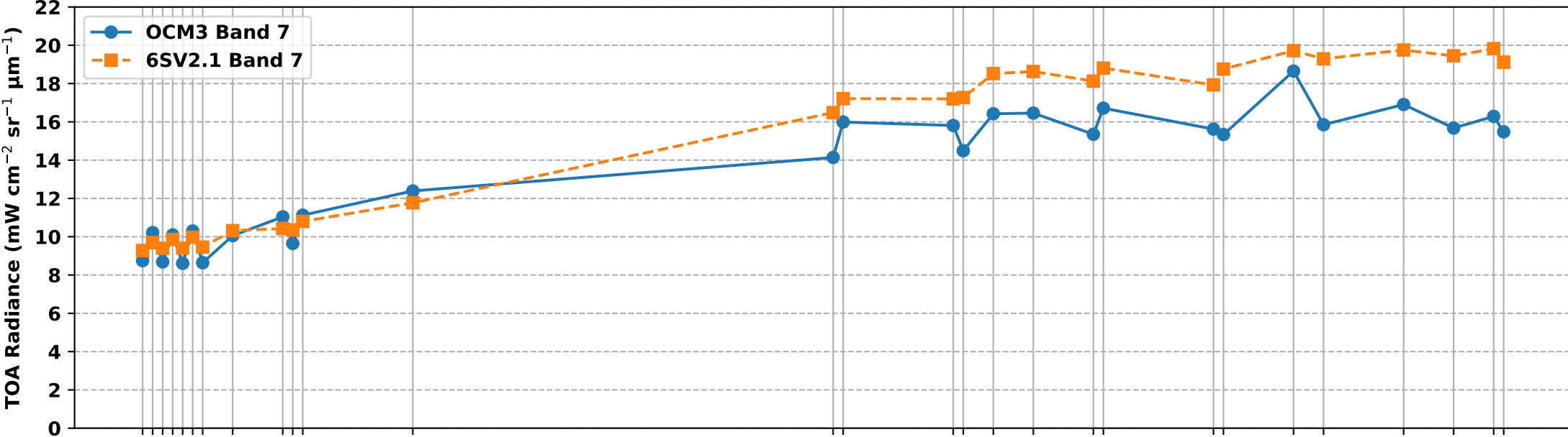
OCM3 Band 7 vs 6S Simulated Band 7 TOA Radiance over RVUS RadCalNet Site (Jan-May 2025)
