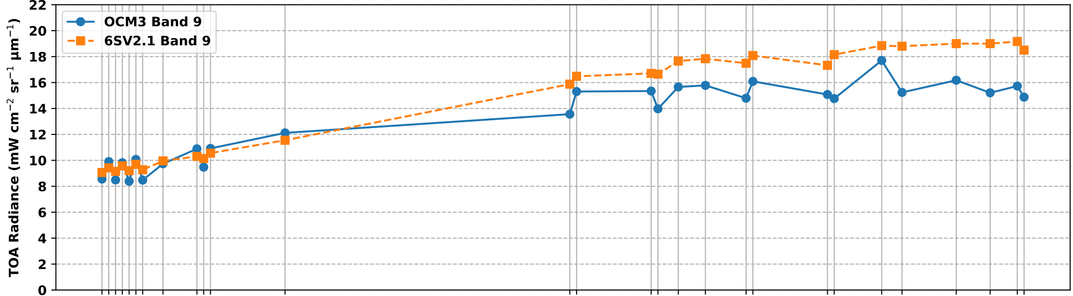
OCM3 Band 9 vs 6S Simulated Band 9 TOA Radiance over RVUS RadCalNet Site (Jan-May 2025)
