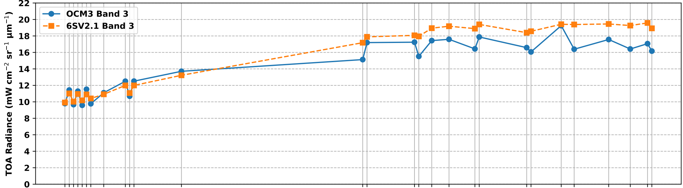
OCM3 Band 3 vs 6S Simulated Band 3 TOA Radiance over RVUS RadCalNet Site (Jan-May 2025)
