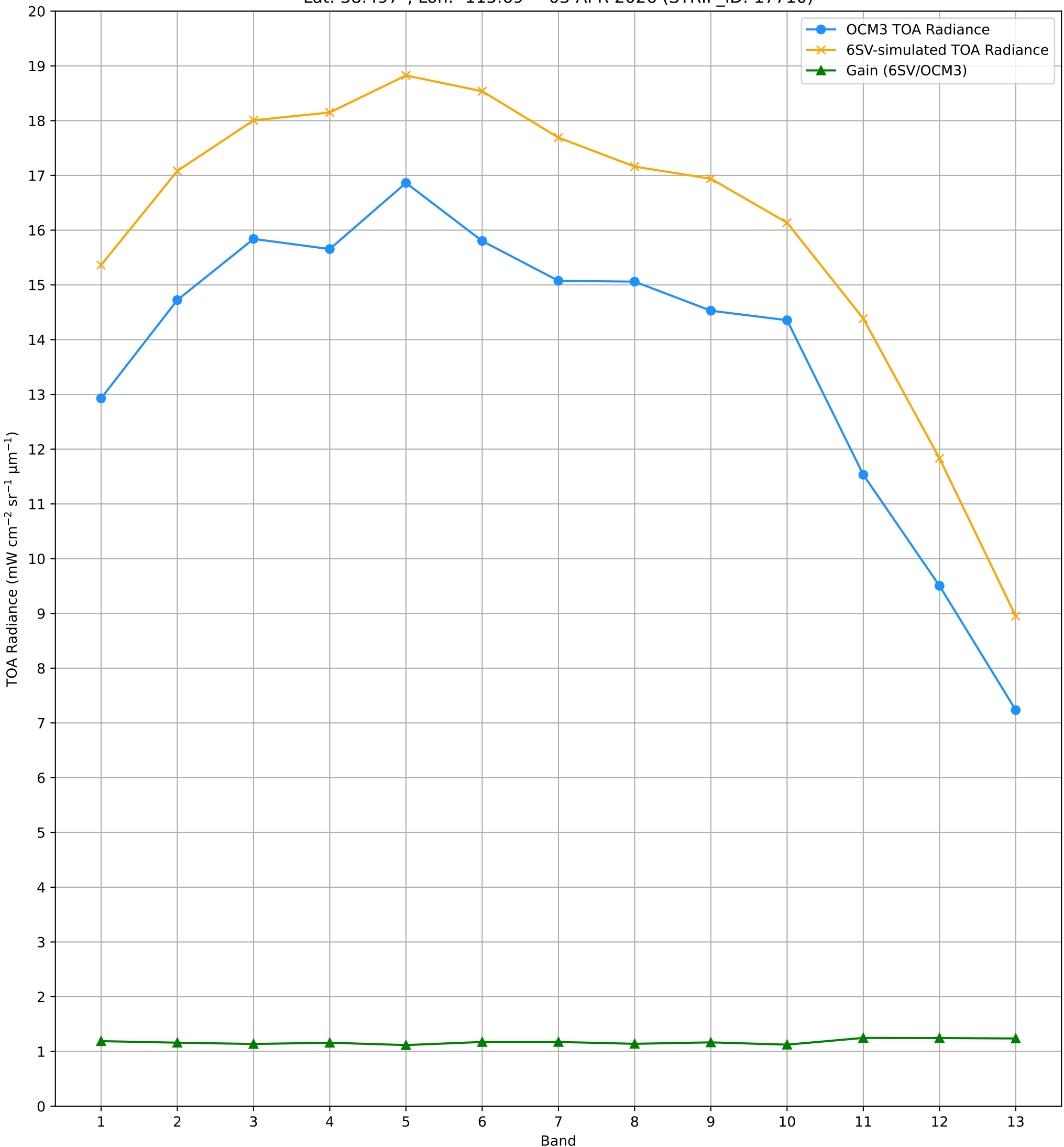
TOA Radiance (OCM3 vs. 6SV) over RVUS RadCalNet Site Lat: 38.497°, Lon: -115.69° - 03-APR-2026 (STRIP_ID: 17710)
