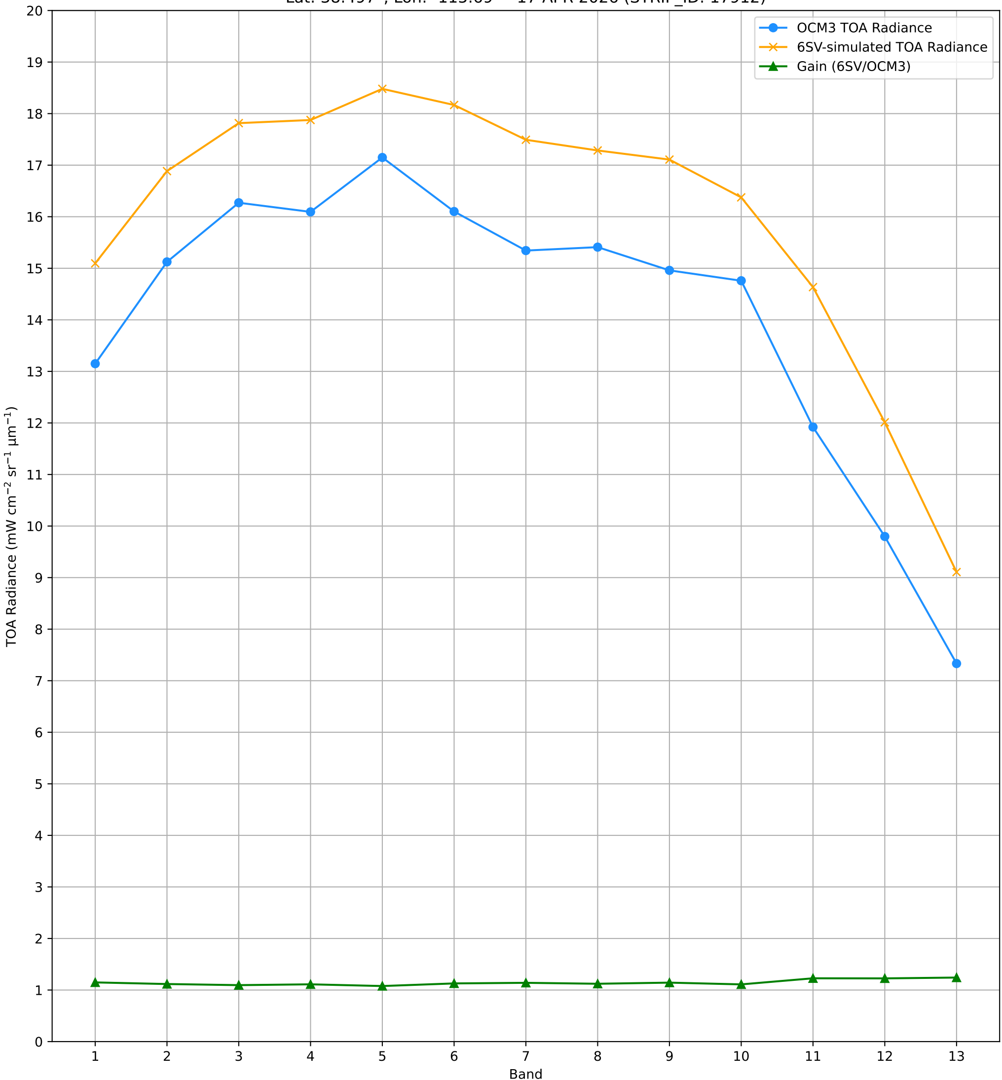
TOA Radiance (OCM3 vs. 6SV) over RVUS RadCalNet Site Lat: 38.497°, Lon: -115.69° - 17-APR-2026 (STRIP_ID: 17912)
