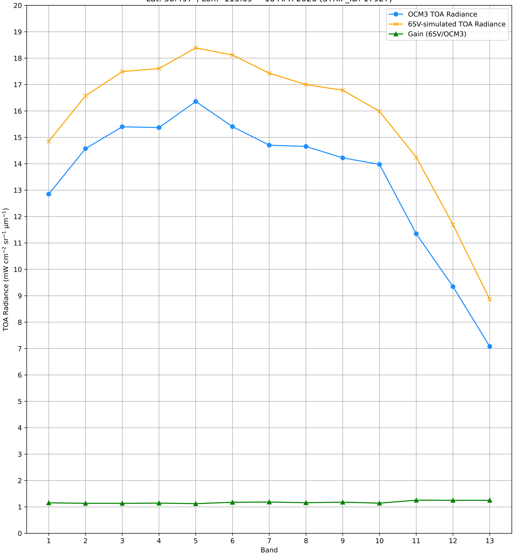
TOA Radiance (OCM3 vs. 6SV) over RVUS RadCalNet Site Lat: 38.497°, Lon: -115.69° - 18-APR-2026 (STRIP_ID: 17927)
