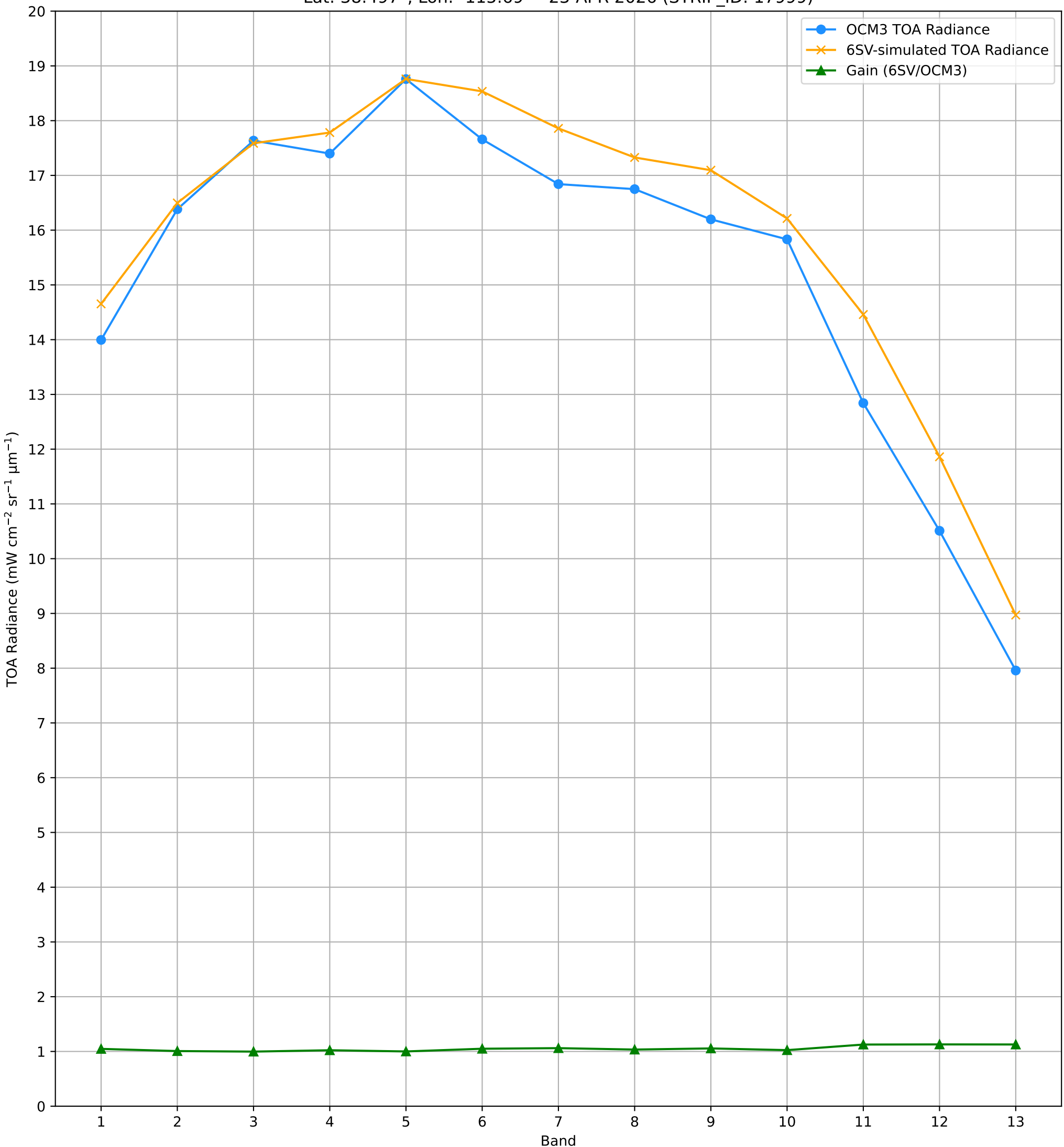
TOA Radiance (OCM3 vs. 6SV) over RVUS RadCalNet Site Lat: 38.497°, Lon: -115.69° - 23-APR-2026 (STRIP_ID: 17999)
