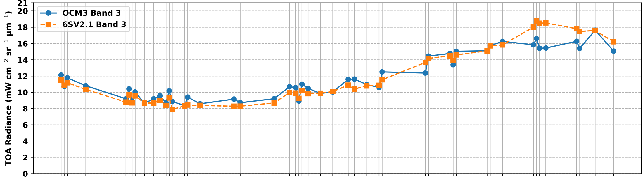
OCM3 Band 3 vs 6S Simulated Band 3 TOA Radiance over RVUS RadCalNet Site (Nov 2025 to Apr 2026)
