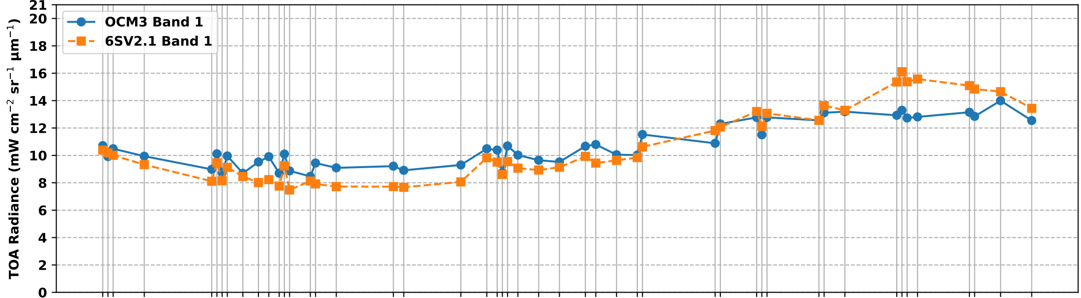
OCM3 Band 1 vs 6S Simulated Band 1 TOA Radiance over RVUS RadCalNet Site (Nov 2025 to Apr 2026)
