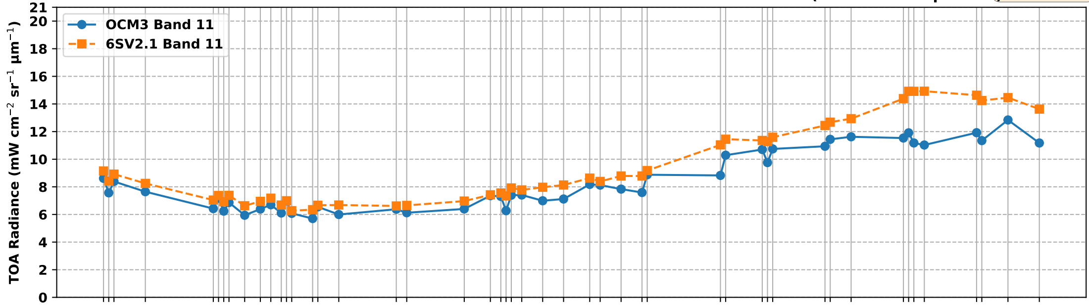
OCM3 Band 11 vs 6S Simulated Band 11 TOA Radiance over RVUS RadCalNet Site (Nov 2025 to Apr 2026)
