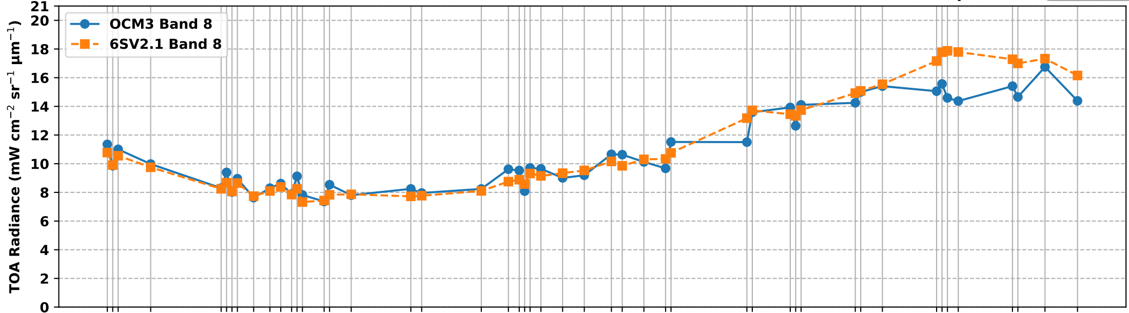
OCM3 Band 8 vs 6S Simulated Band 8 TOA Radiance over RVUS RadCalNet Site (Nov 2025 to Apr 2026)
