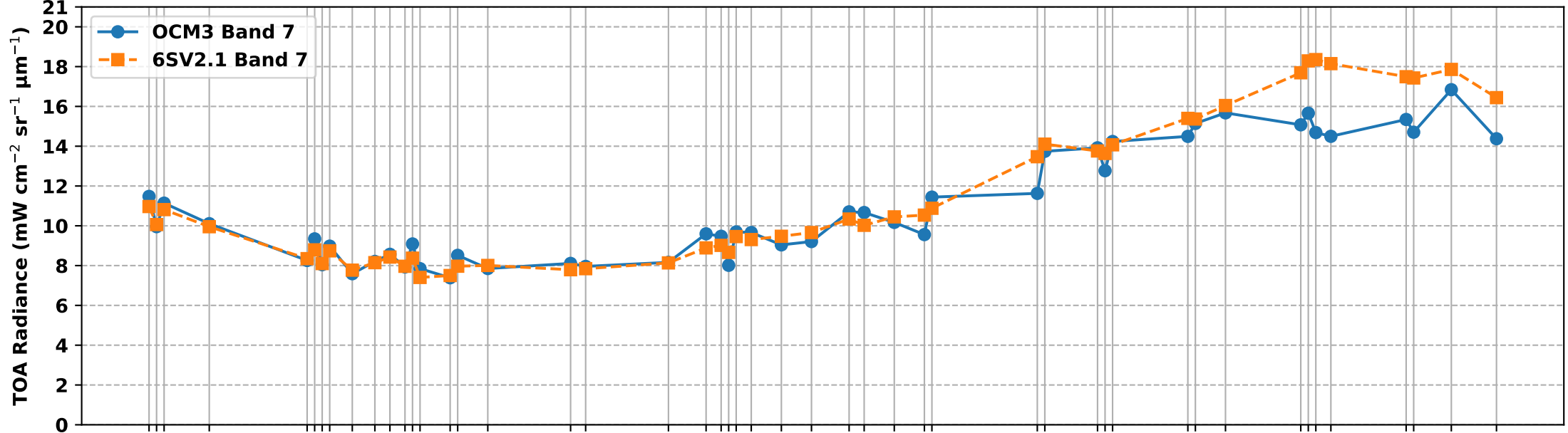
OCM3 Band 7 vs 6S Simulated Band 7 TOA Radiance over RVUS RadCalNet Site (Nov 2025 to Apr 2026)
