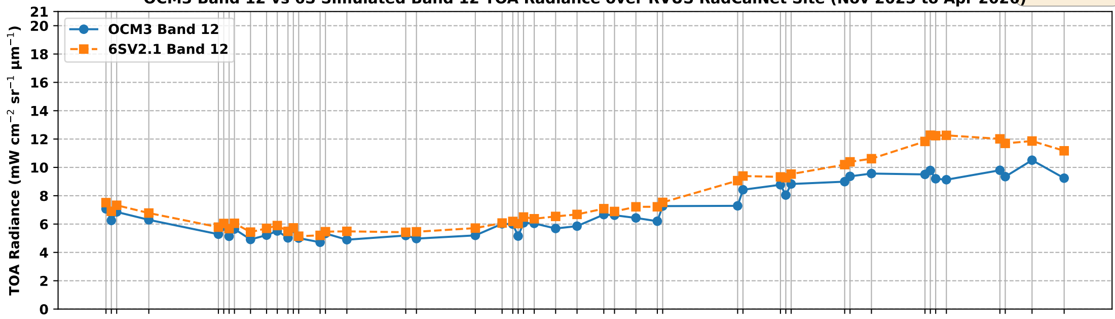
OCM3 Band 12 vs 6S Simulated Band 12 TOA Radiance over RVUS RadCalNet Site (Nov 2025 to Apr 2026)
