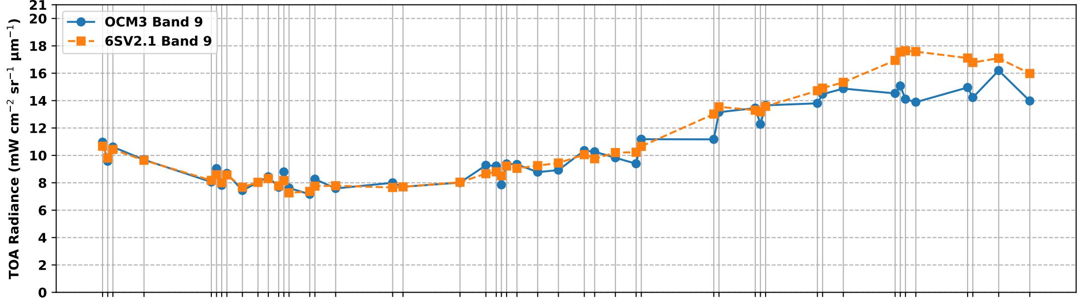
OCM3 Band 9 vs 6S Simulated Band 9 TOA Radiance over RVUS RadCalNet Site (Nov 2025 to Apr 2026)
