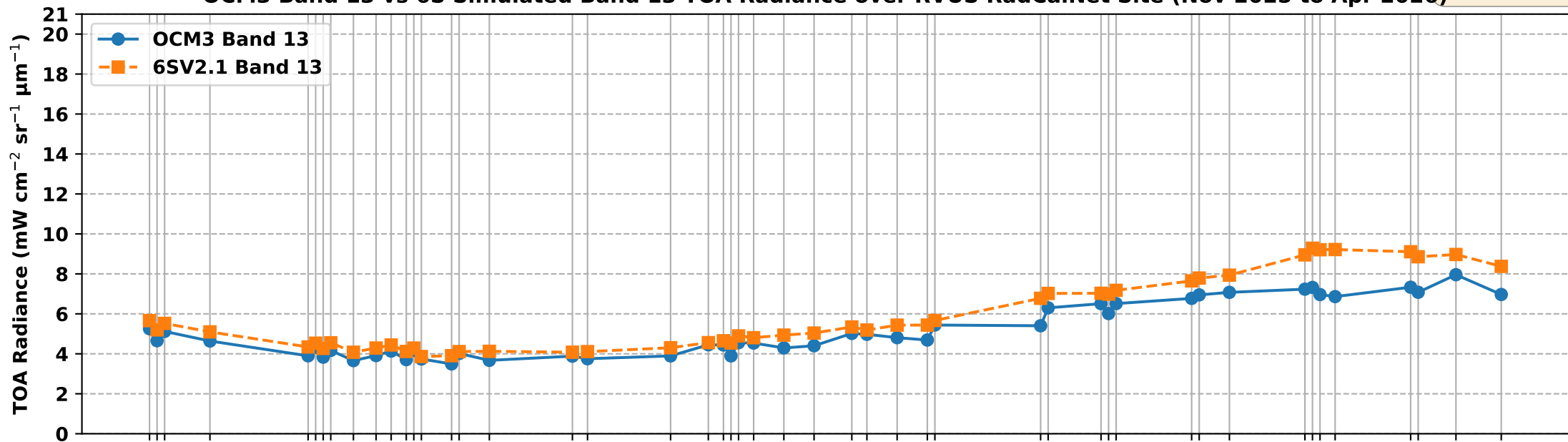
OCM3 Band 13 vs 6S Simulated Band 13 TOA Radiance over RVUS RadCalNet Site (Nov 2025 to Apr 2026)
