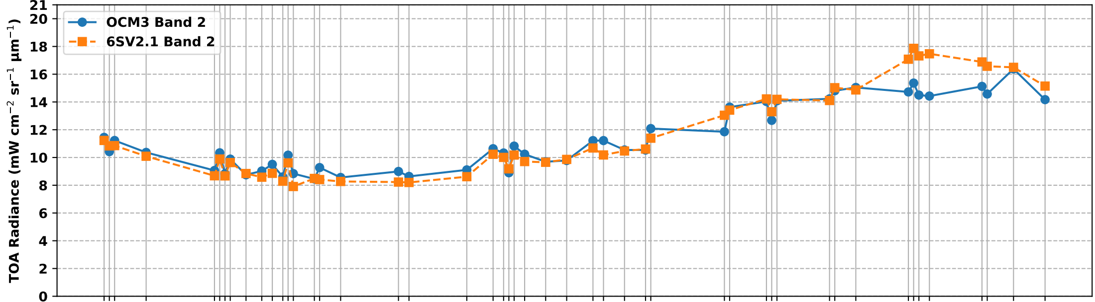
OCM3 Band 2 vs 6S Simulated Band 2 TOA Radiance over RVUS RadCalNet Site (Nov 2025 to Apr 2026)
