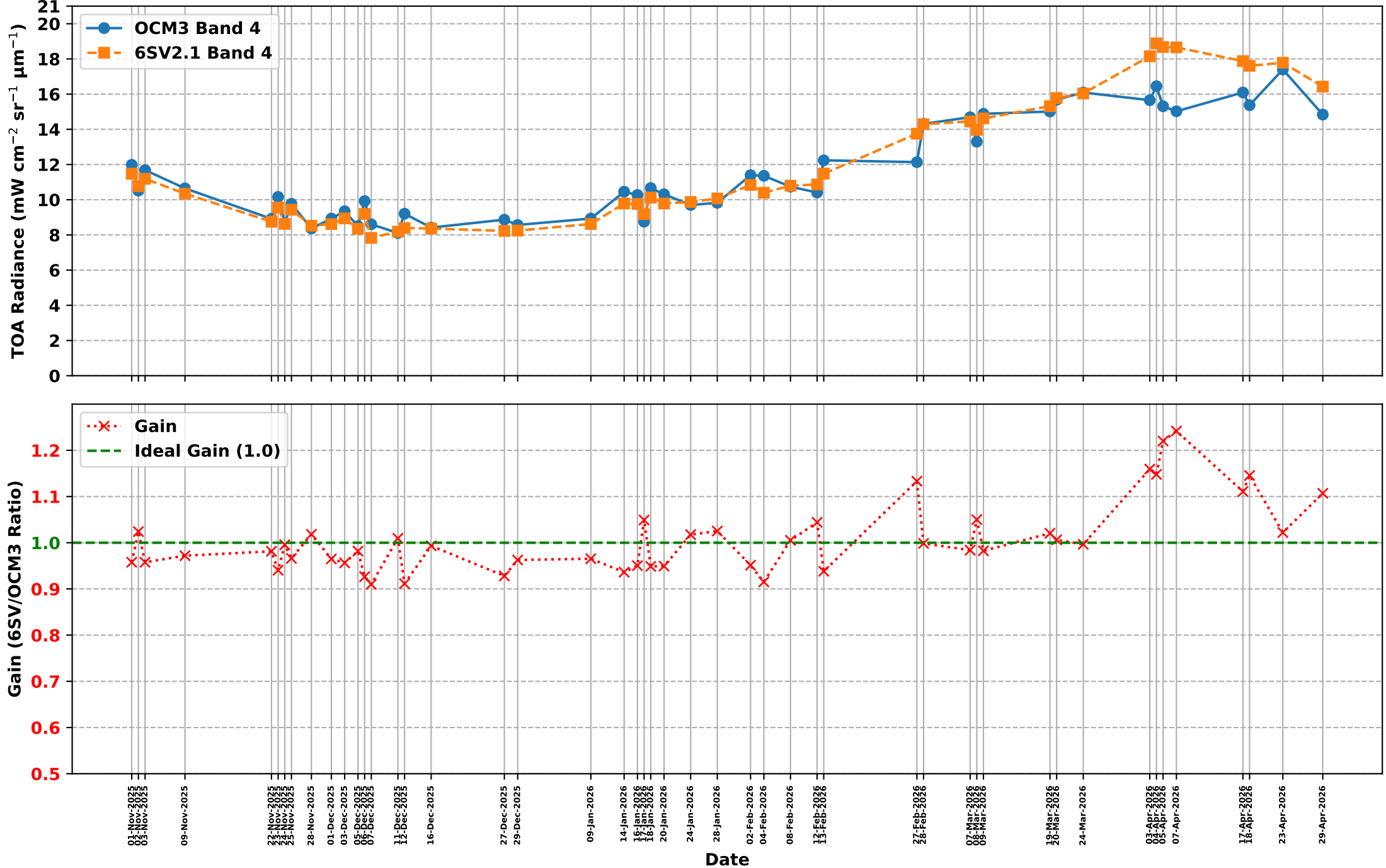
OCM3 Band 4 vs 6S Simulated Band 4 TOA Radiance over RVUS RadCalNet Site (Nov 2025 to Apr 2026)
