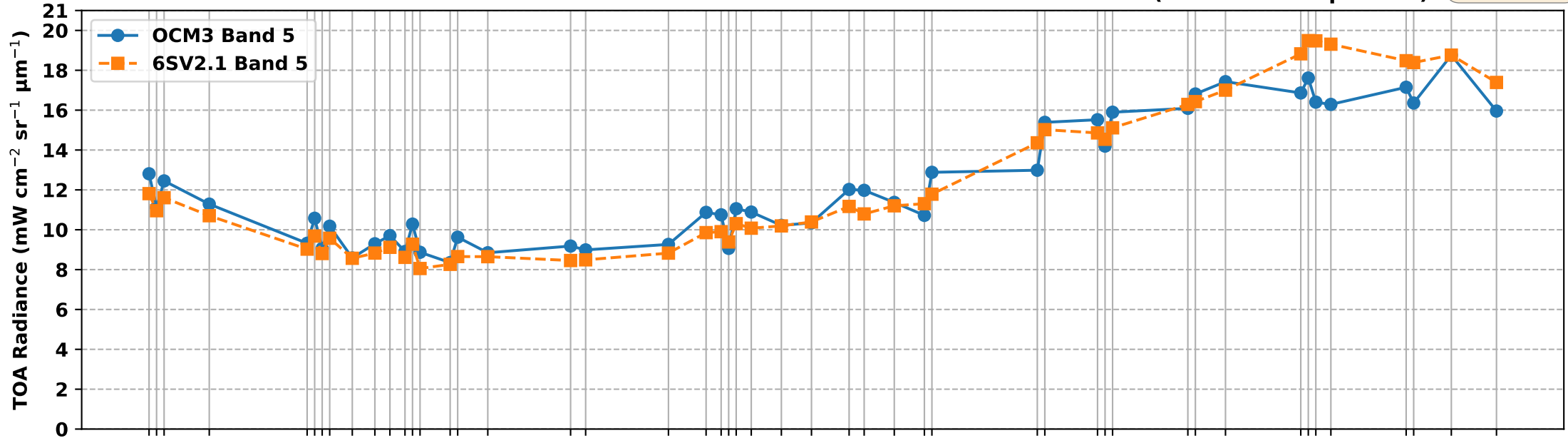
OCM3 Band 5 vs 6S Simulated Band 5 TOA Radiance over RVUS RadCalNet Site (Nov 2025 to Apr 2026)
