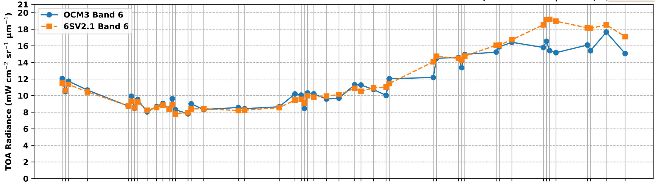
OCM3 Band 6 vs 6S Simulated Band 6 TOA Radiance over RVUS RadCalNet Site (Nov 2025 to Apr 2026)
