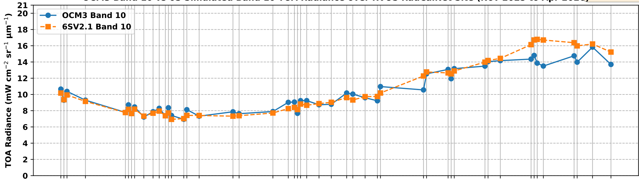
OCM3 Band 10 vs 6S Simulated Band 10 TOA Radiance over RVUS RadCalNet Site (Nov 2025 to Apr 2026)
