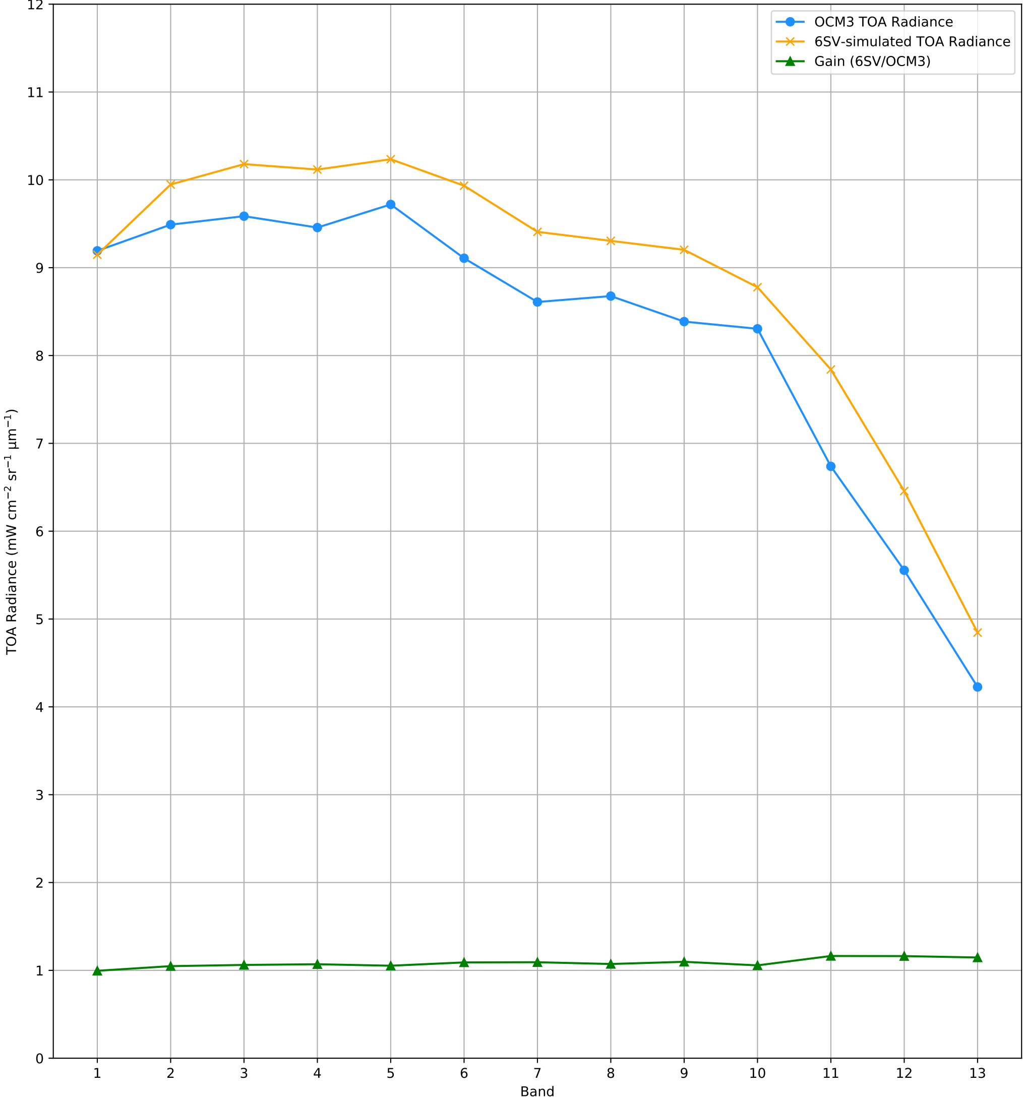
TOA Radiance (OCM3 vs. 6SV) over RVUS RadCalNet Site Lat: 38.497°, Lon: -115.69° - 18-JAN-2025 (STRIP_ID: 11347)
