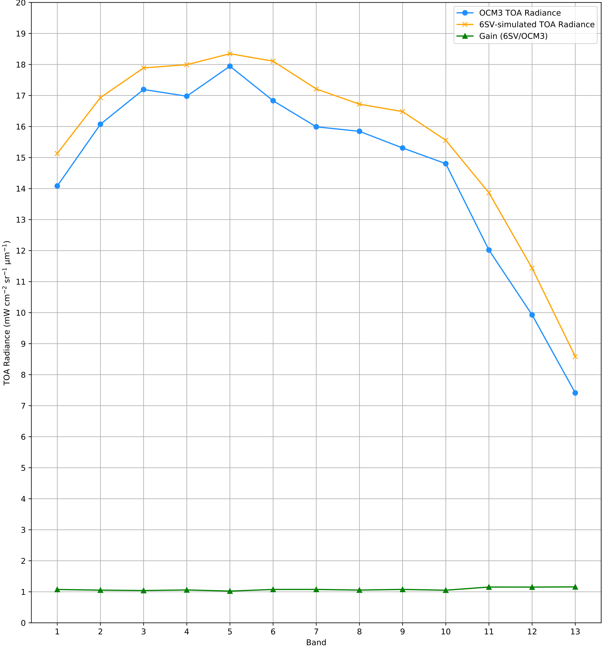
TOA Radiance (OCM3 vs. 6SV) over RVUS RadCalNet Site Lat: 38.497°, Lon: -115.69° - 25-MAR-2025 (STRIP_ID: 12301)
