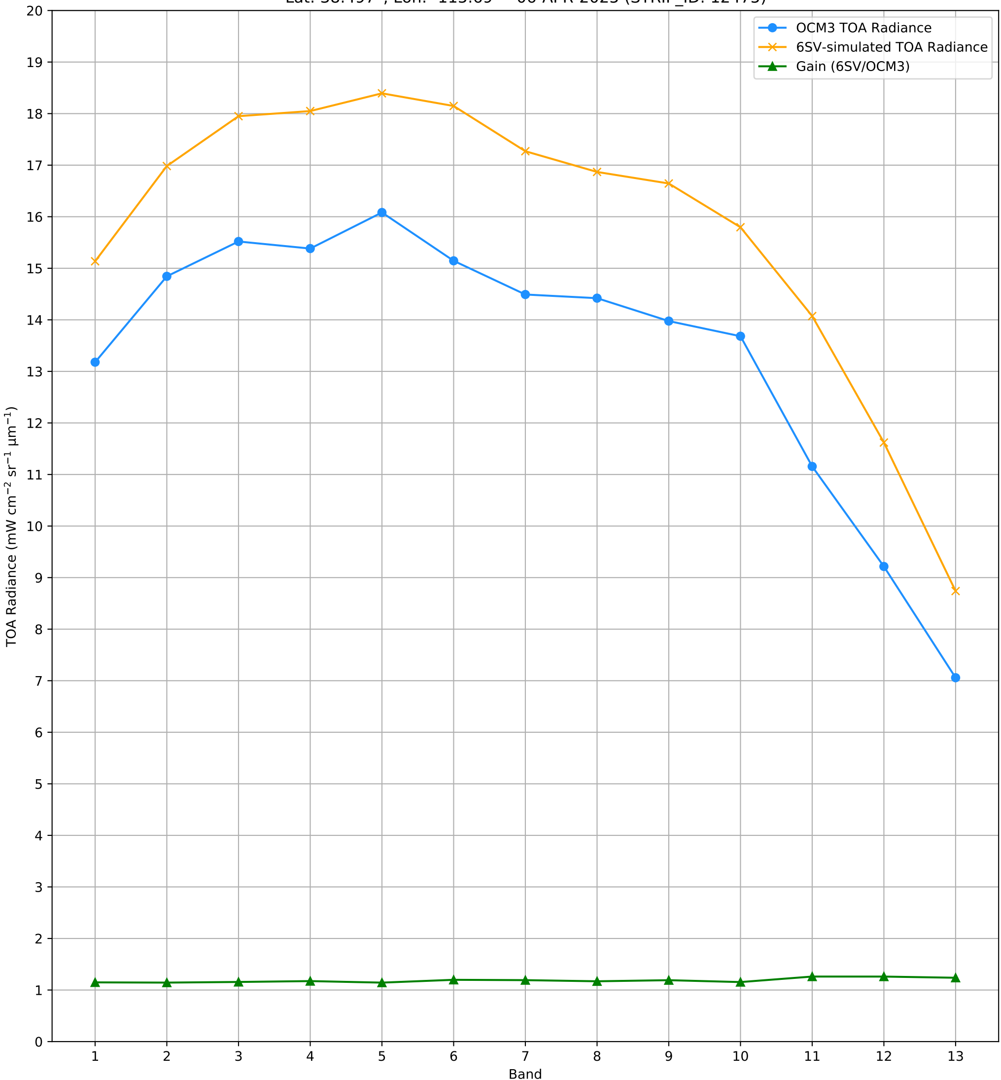
TOA Radiance (OCM3 vs. 6SV) over RVUS RadCalNet Site Lat: 38.497°, Lon: -115.69° - 06-APR-2025 (STRIP_ID: 12475)
