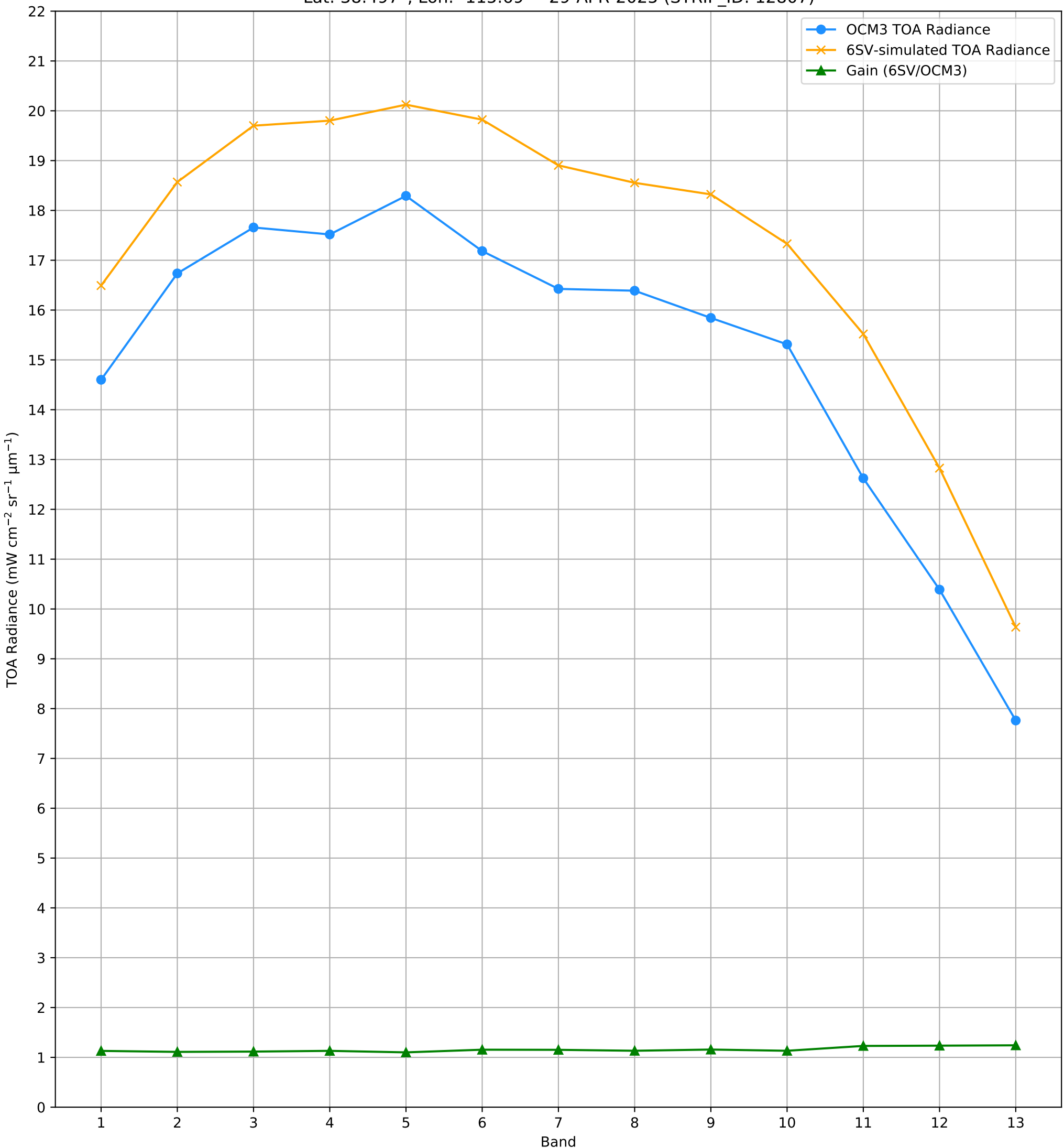
TOA Radiance (OCM3 vs. 6SV) over RVUS RadCalNet Site Lat: 38.497°, Lon: -115.69° - 29-APR-2025 (STRIP_ID:12807)
