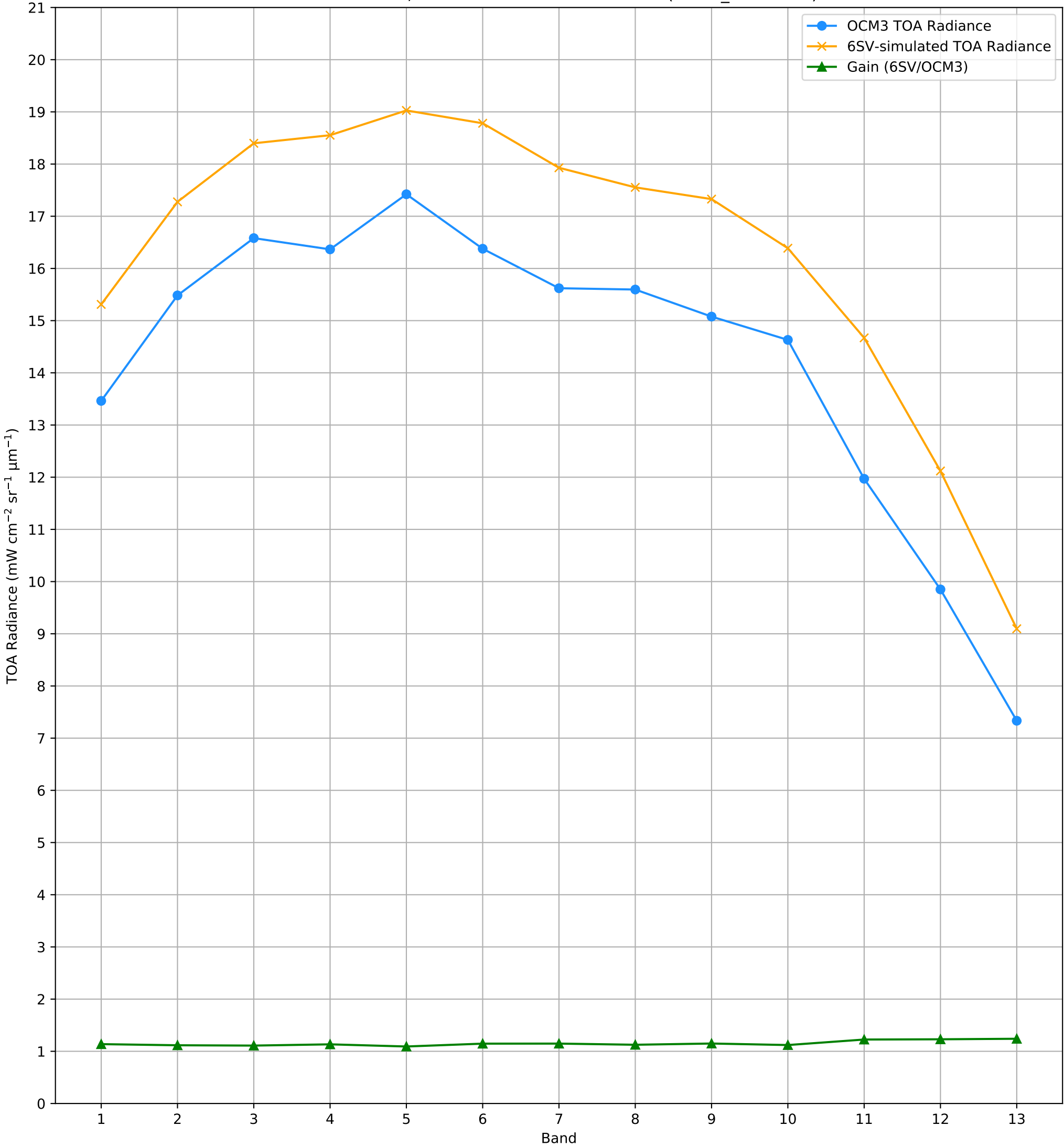
TOA Radiance (OCM3 vs. 6SV) over RVUS RadCalNet Site Lat: 38.497°, Lon: -115.69° - 01-MAY-2025 (STRIP_ID: 12836)
