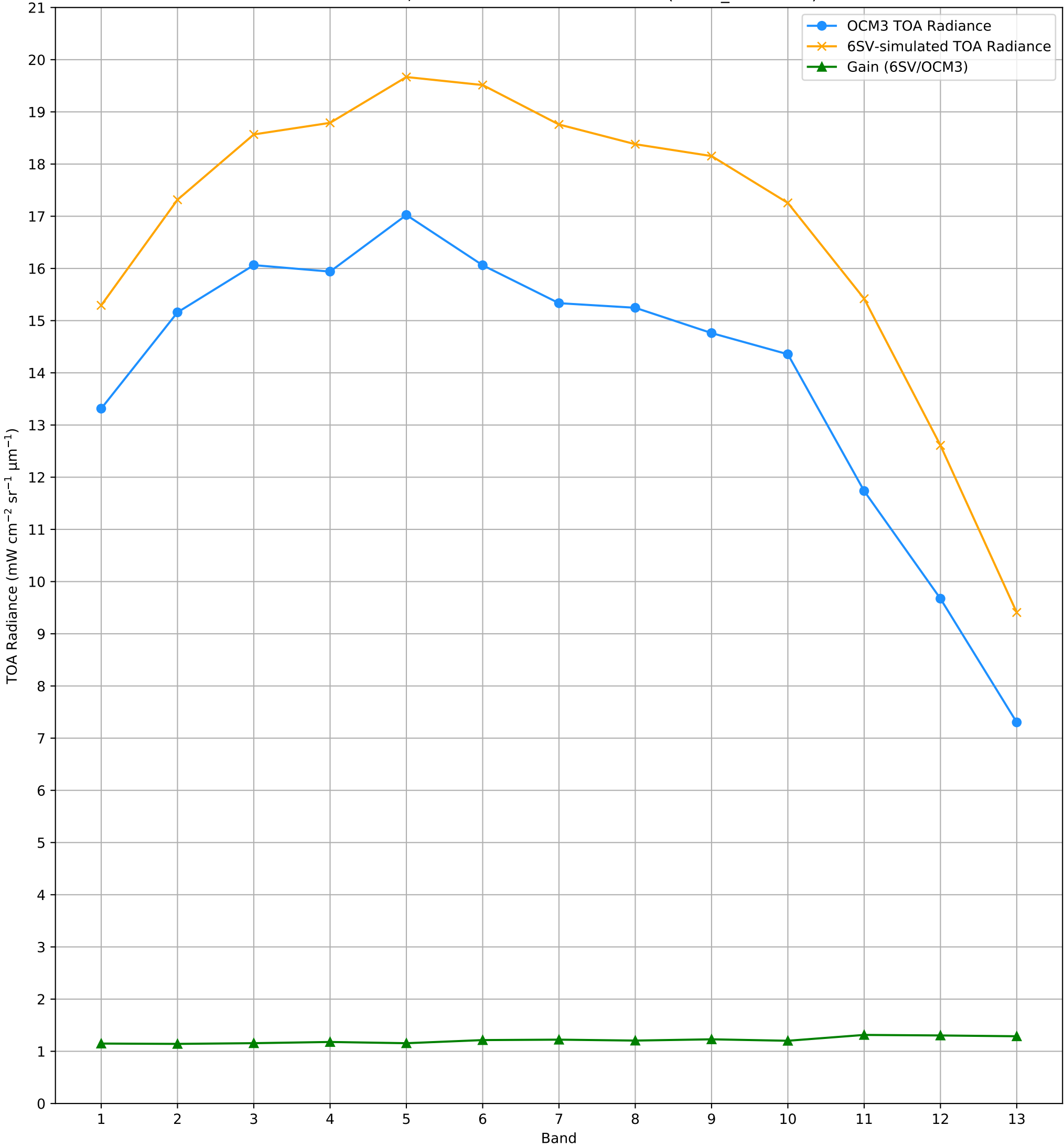
TOA Radiance (OCM3 vs. 6SV) over RVUS RadCalNet Site Lat: 38.497°, Lon: -115.69° - 02-MAY-2025 (STRIP_ID: 12851)
