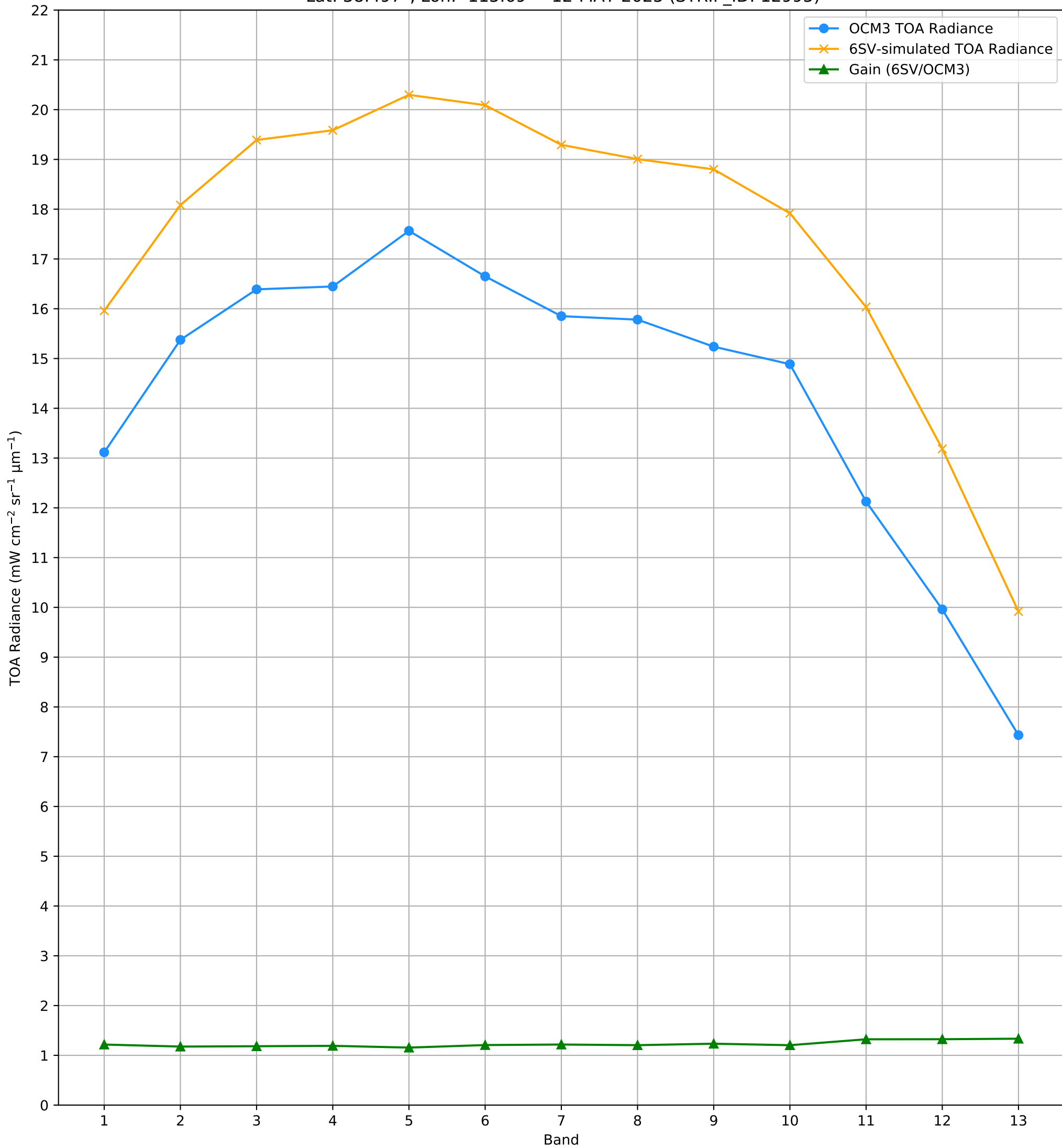
TOA Radiance (OCM3 vs. 6SV) over RVUS RadCalNet Site Lat: 38.497°, Lon: -115.69° - 12-MAY-2025 (STRIP_ID: 12995)
