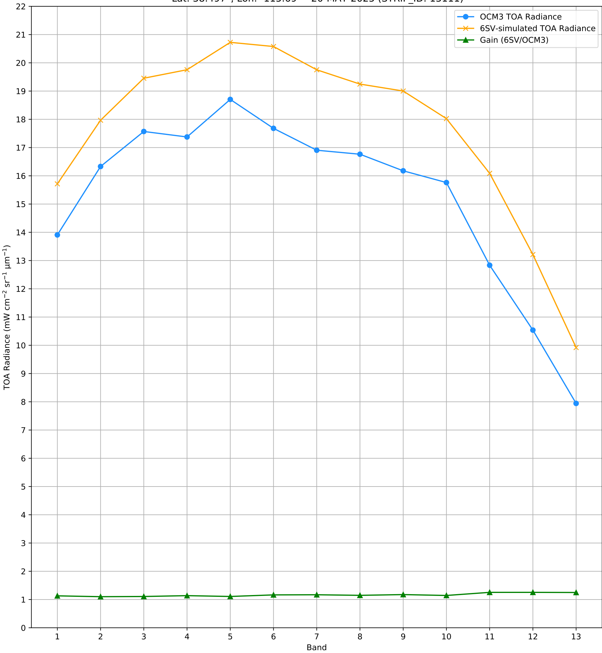
TOA Radiance (OCM3 vs. 6SV) over RVUS RadCalNet Site Lat: 38.497°, Lon: -115.69° - 20-MAY-2025 (STRIP_ID: 13111)
