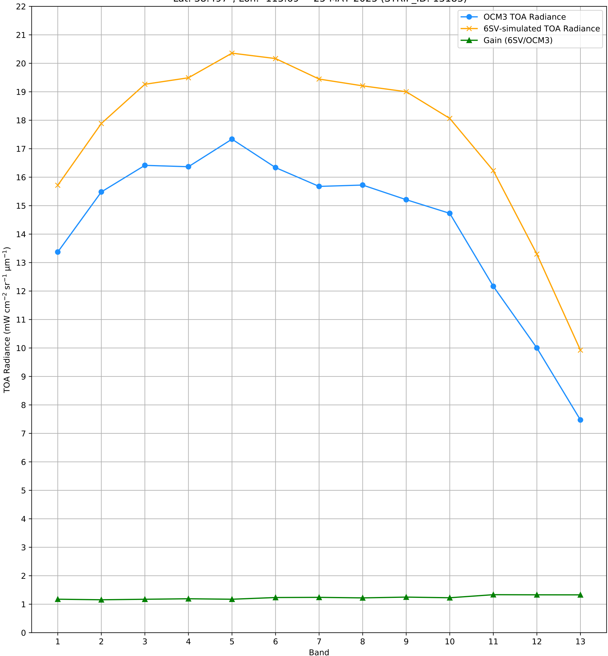
TOA Radiance (OCM3 vs. 6SV) over RVUS RadCalNet Site Lat: 38.497°, Lon: -115.69° - 25-MAY-2025 (STRIP_ID: 13183)
