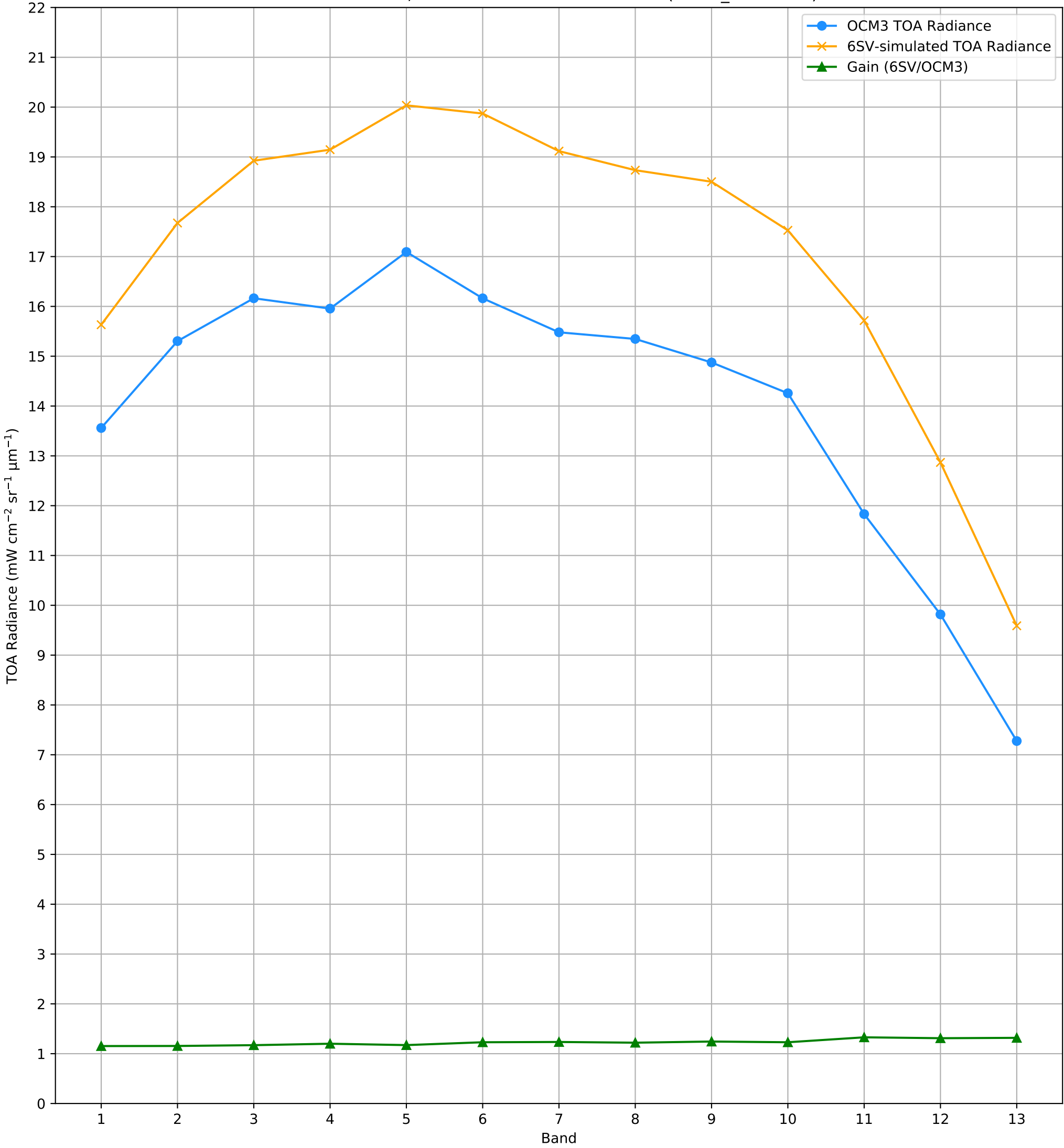
TOA Radiance (OCM3 vs. 6SV) over RVUS RadCalNet Site Lat: 38.497°, Lon: -115.69° - 30-MAY-2025 (STRIP_ID: 13256)
