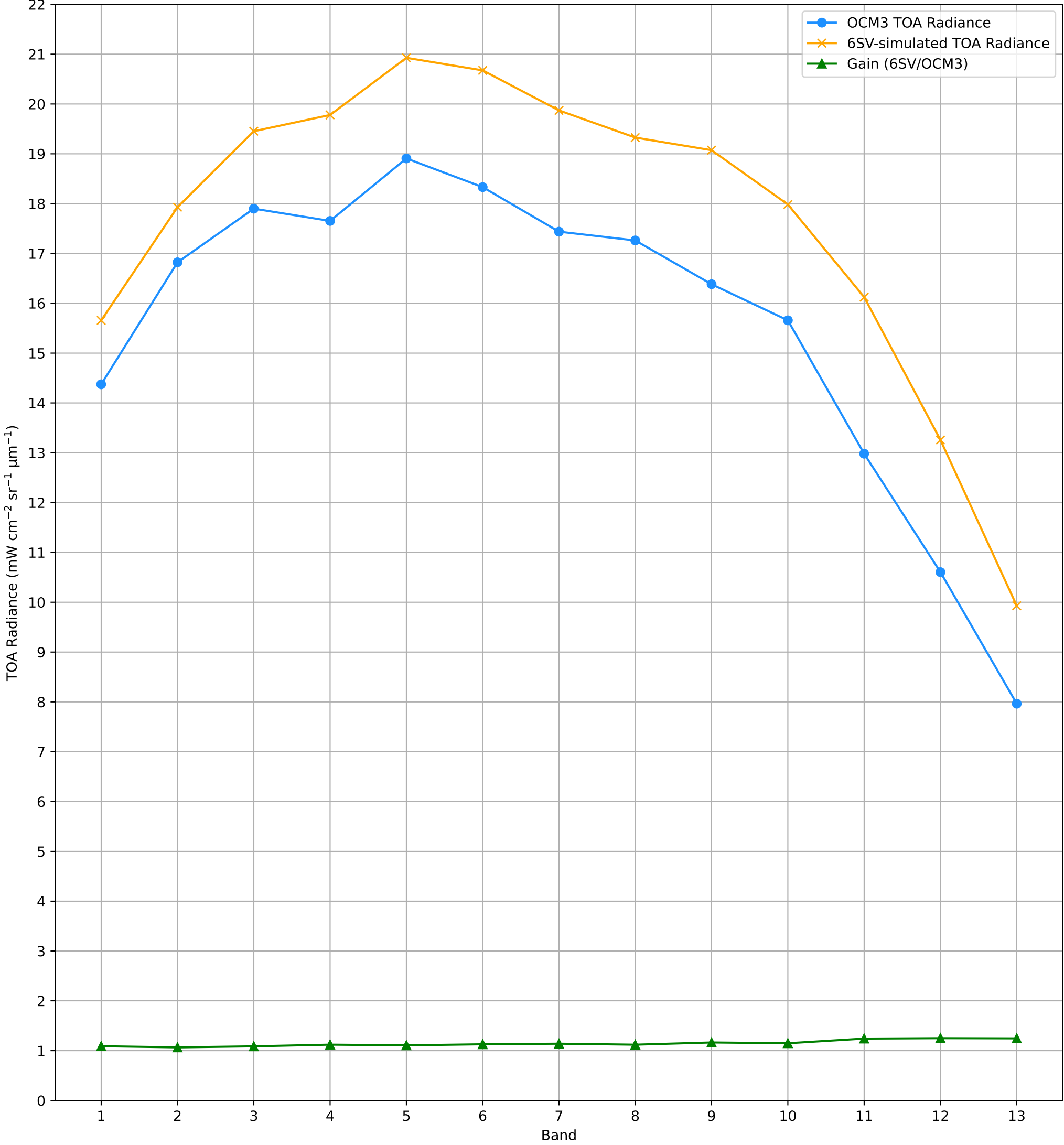
TOA Radiance (OCM3 vs. 6SV) over RVUS RadCalNet Site Lat: 38.497°, Lon: -115.69° - 02-JUN-2025 (STRIP_ID: 13299)
