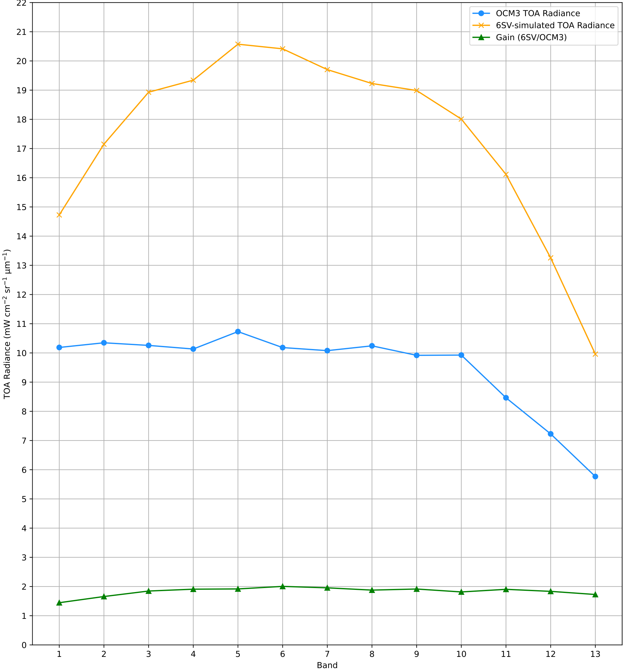
TOA Radiance (OCM3 vs. 6SV) over RVUS RadCalNet Site Lat: 38.497°, Lon: -115.69° - 04-JUN-2025 (STRIP_ID: 13328)
