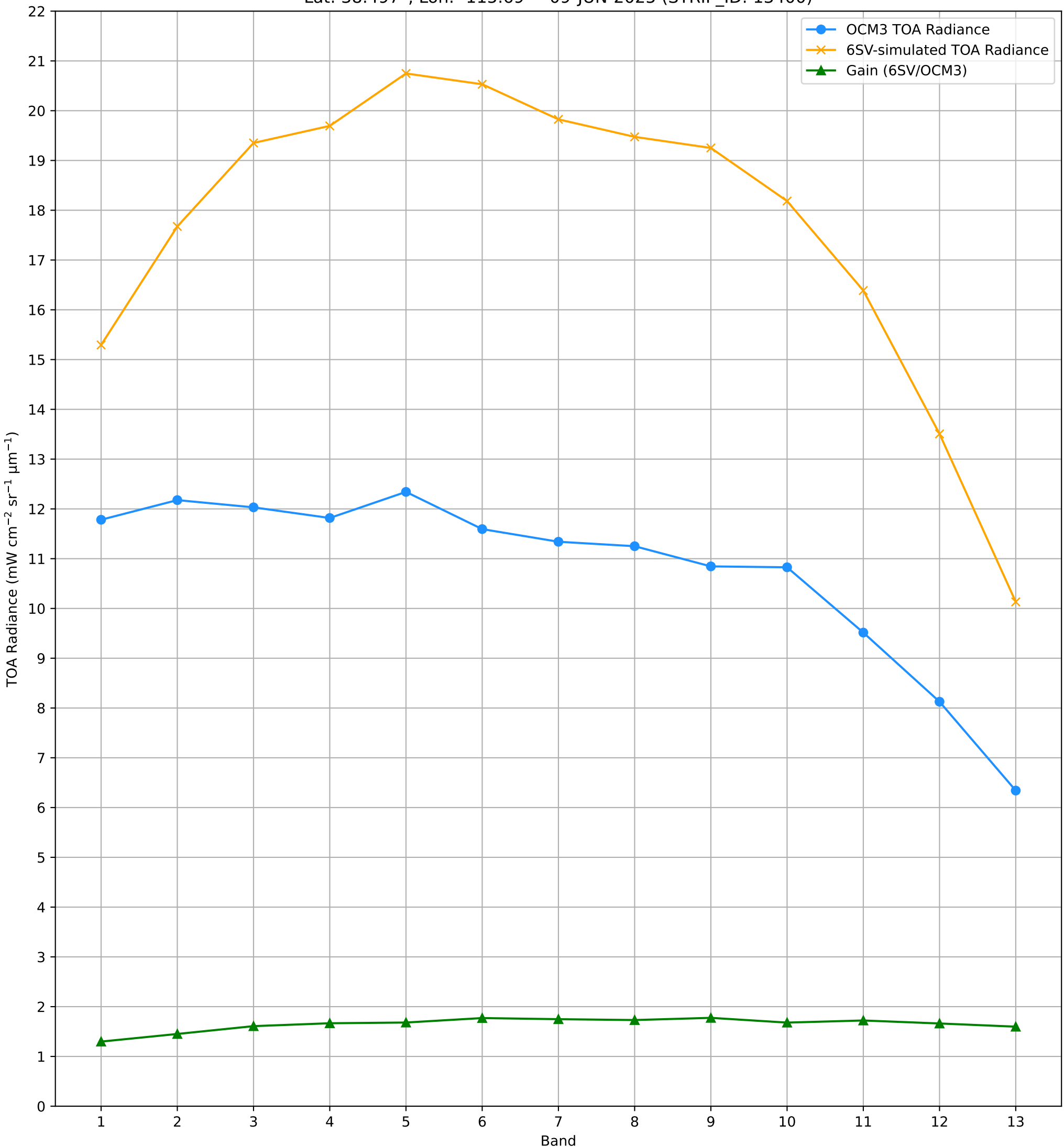
TOA Radiance (OCM3 vs. 6SV) over RVUS RadCalNet Site Lat: 38.497°, Lon: -115.69° - 09-JUN-2025 (STRIP_ID: 13400)
