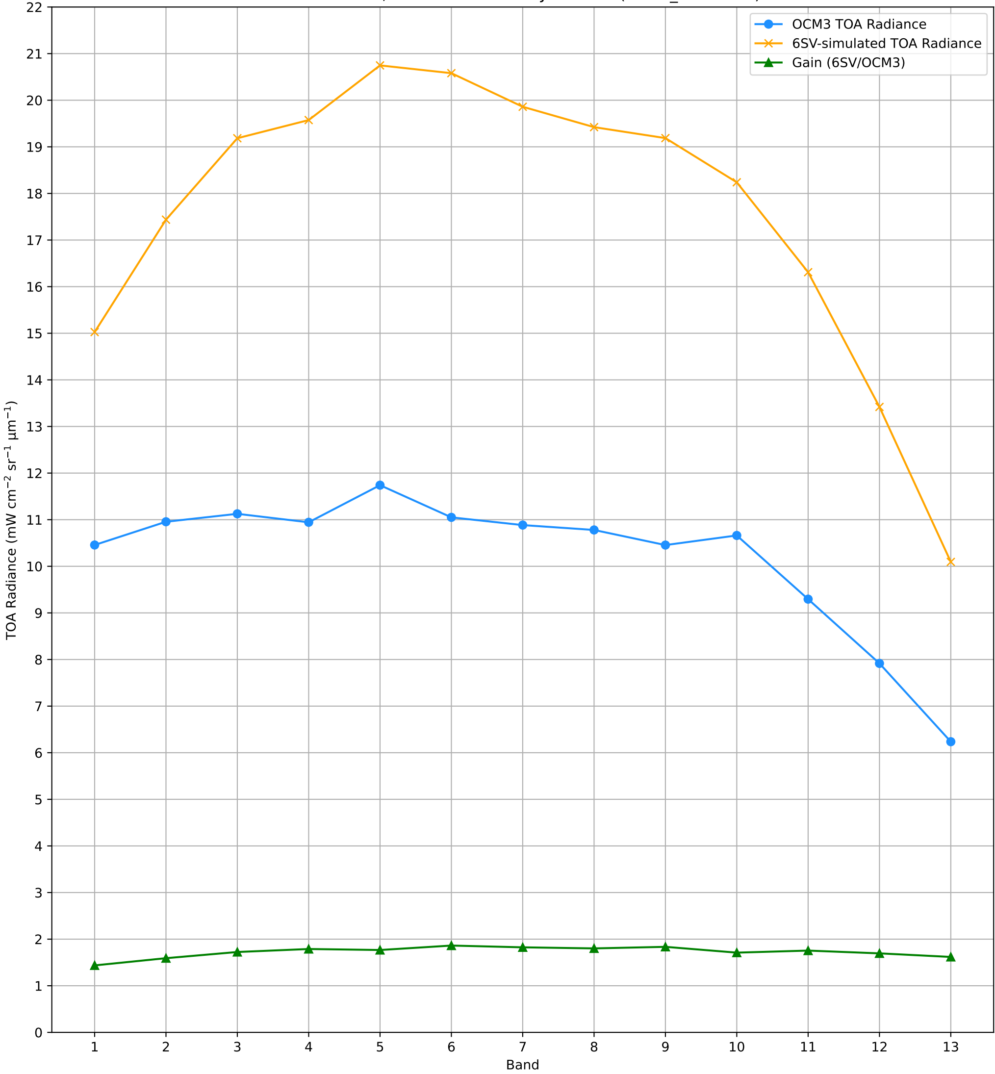
TOA Radiance (OCM3 vs. 6SV) over RVUS RadCalNet Site Lat: 38.497°, Lon: -115.69° - 11-JUN-2025 (STRIP_ID: 13429)
