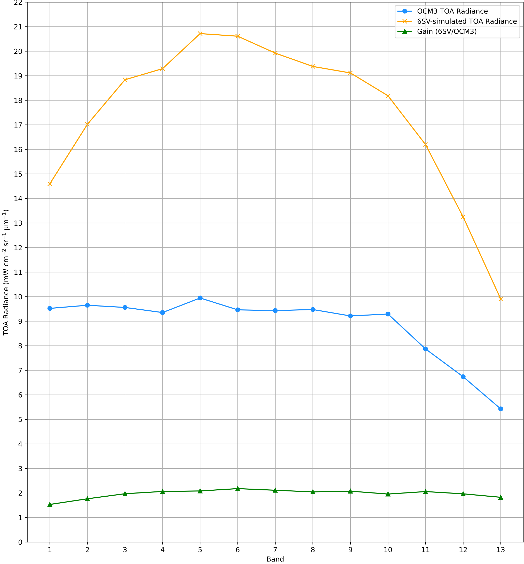
TOA Radiance (OCM3 vs. 6SV) over RVUS RadCalNet Site Lat: 38.497°, Lon: -115.69° - 19-JUN-2025 (STRIP_ID: 13545)
