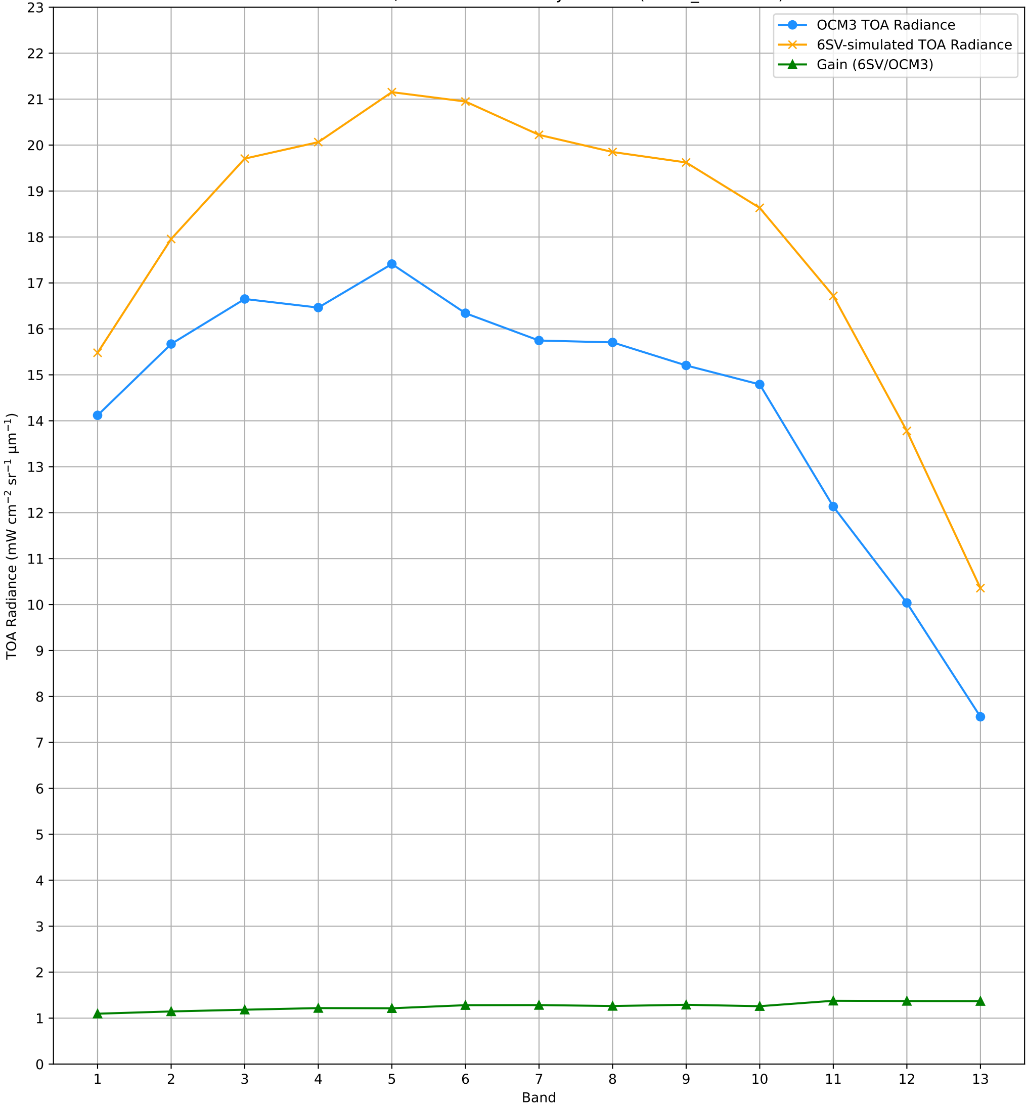
TOA Radiance (OCM3 vs. 6SV) over RVUS RadCalNet Site Lat: 38.497°, Lon: -115.69° - 24-JUN-2025 (STRIP_ID: 13617)
