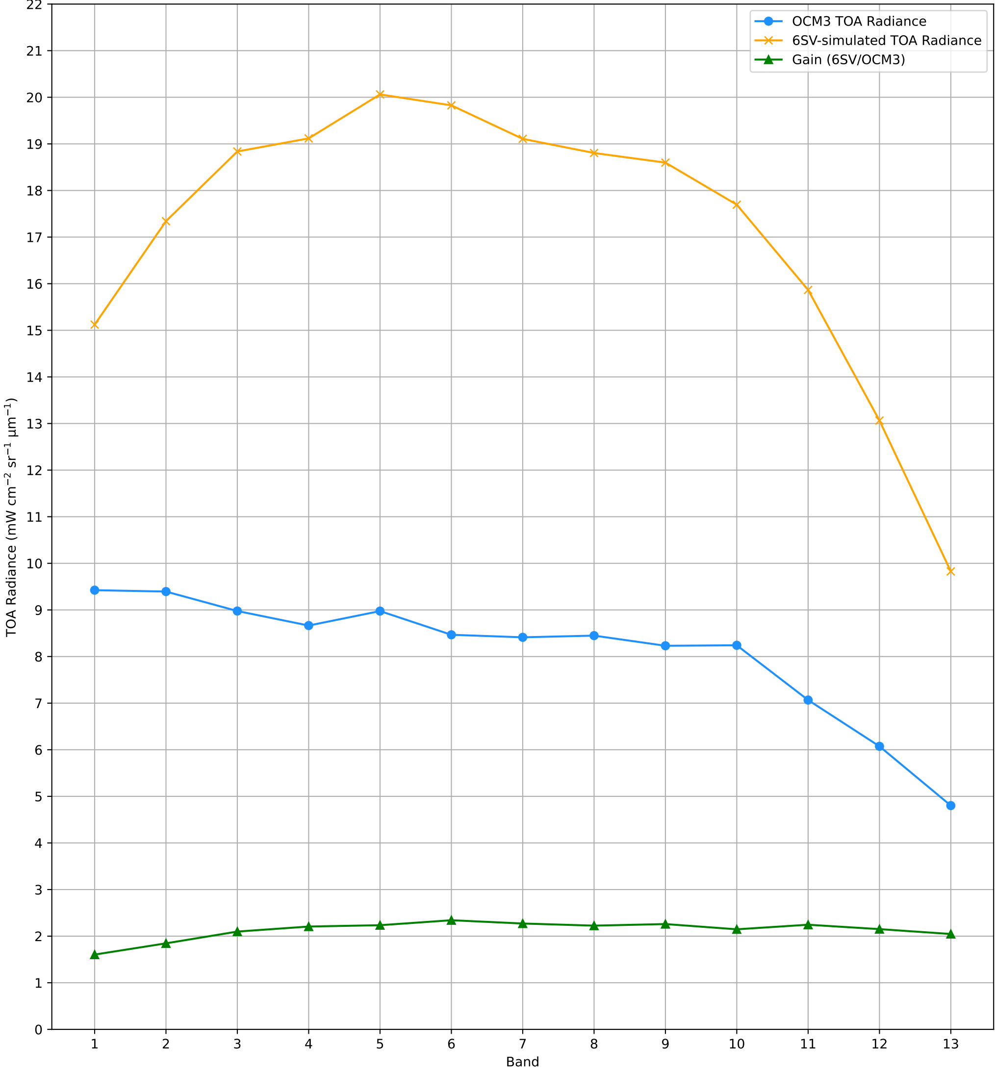
TOA Radiance (OCM3 vs. 6SV) over RVUS RadCalNet Site Lat: 38.497°, Lon: -115.69° - 25-JUN-2025 (STRIP_ID: 13632)
