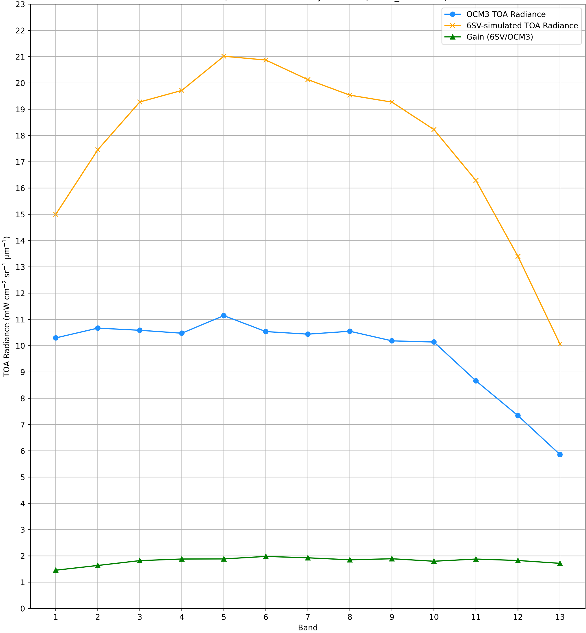
TOA Radiance (OCM3 vs. 6SV) over RVUS RadCalNet Site Lat: 38.497°, Lon: -115.69° - 30-JUN-2025 (STRIP_ID: 13704)
