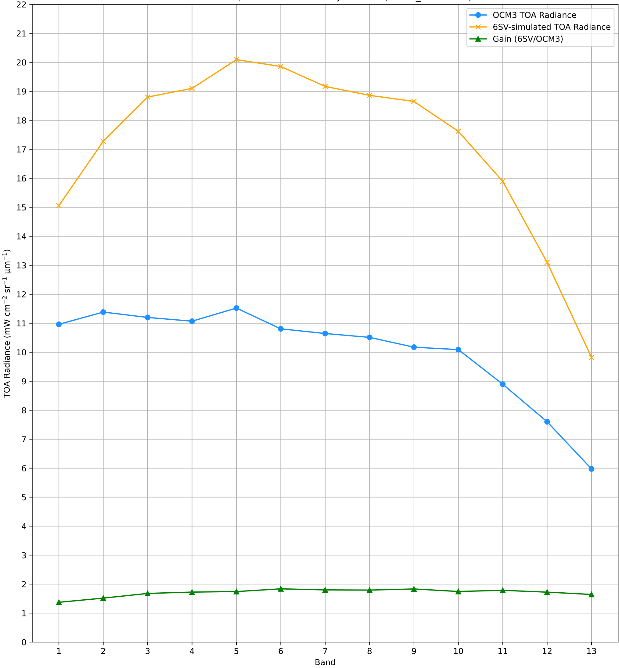
TOA Radiance (OCM3 vs. 6SV) over RVUS RadCalNet Site Lat: 38.497°, Lon: -115.69° - 03-JUL-2025 (STRIP_ID: 13747)
