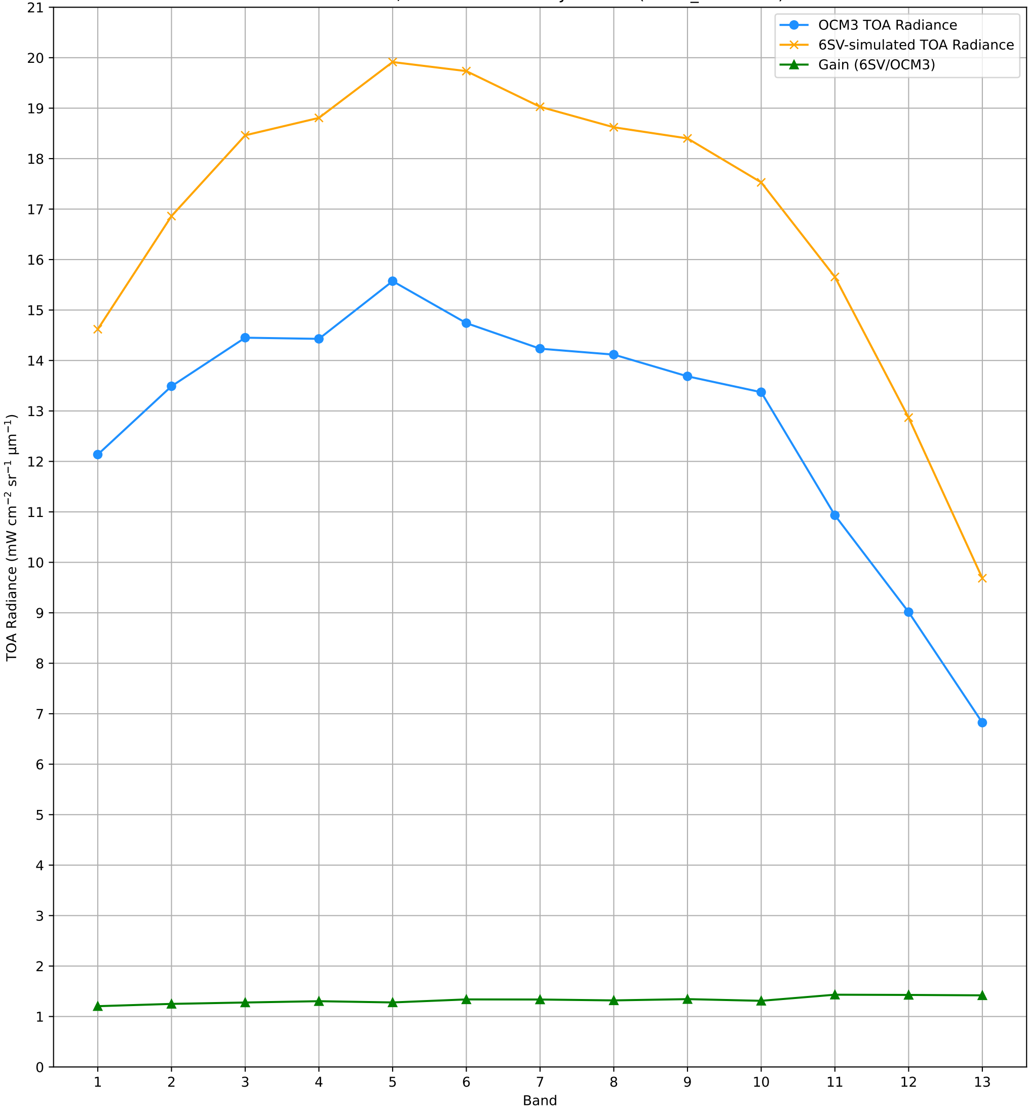
TOA Radiance (OCM3 vs. 6SV) over RVUS RadCalNet Site Lat: 38.497°, Lon: -115.69° - 06-JUL-2025 (STRIP_ID: 13791)
