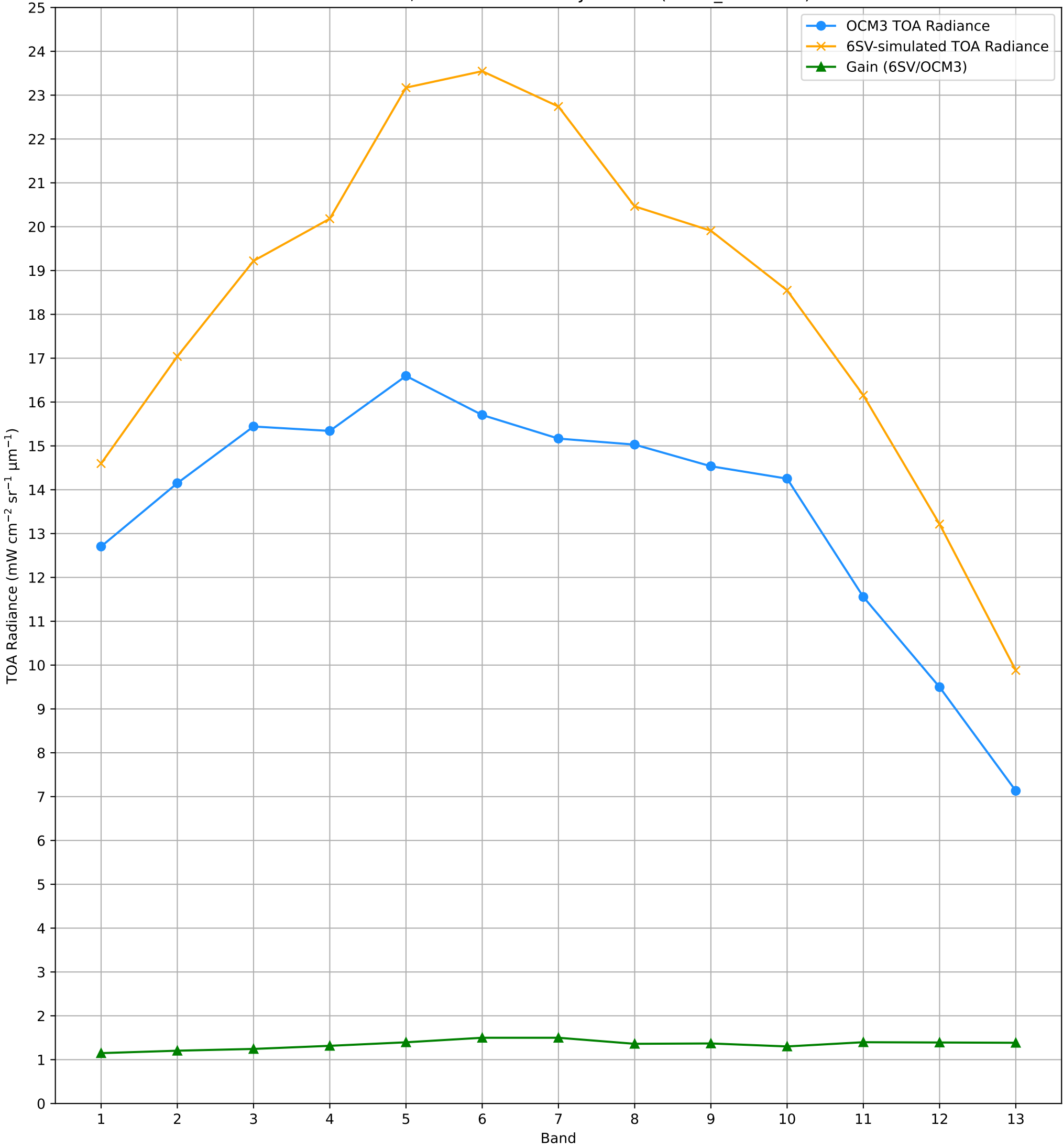
TOA Radiance (OCM3 vs. 6SV) over RVUS RadCalNet Site Lat: 38.497°, Lon: -115.69° - 07-JUL-2025 (STRIP_ID: 13805)
