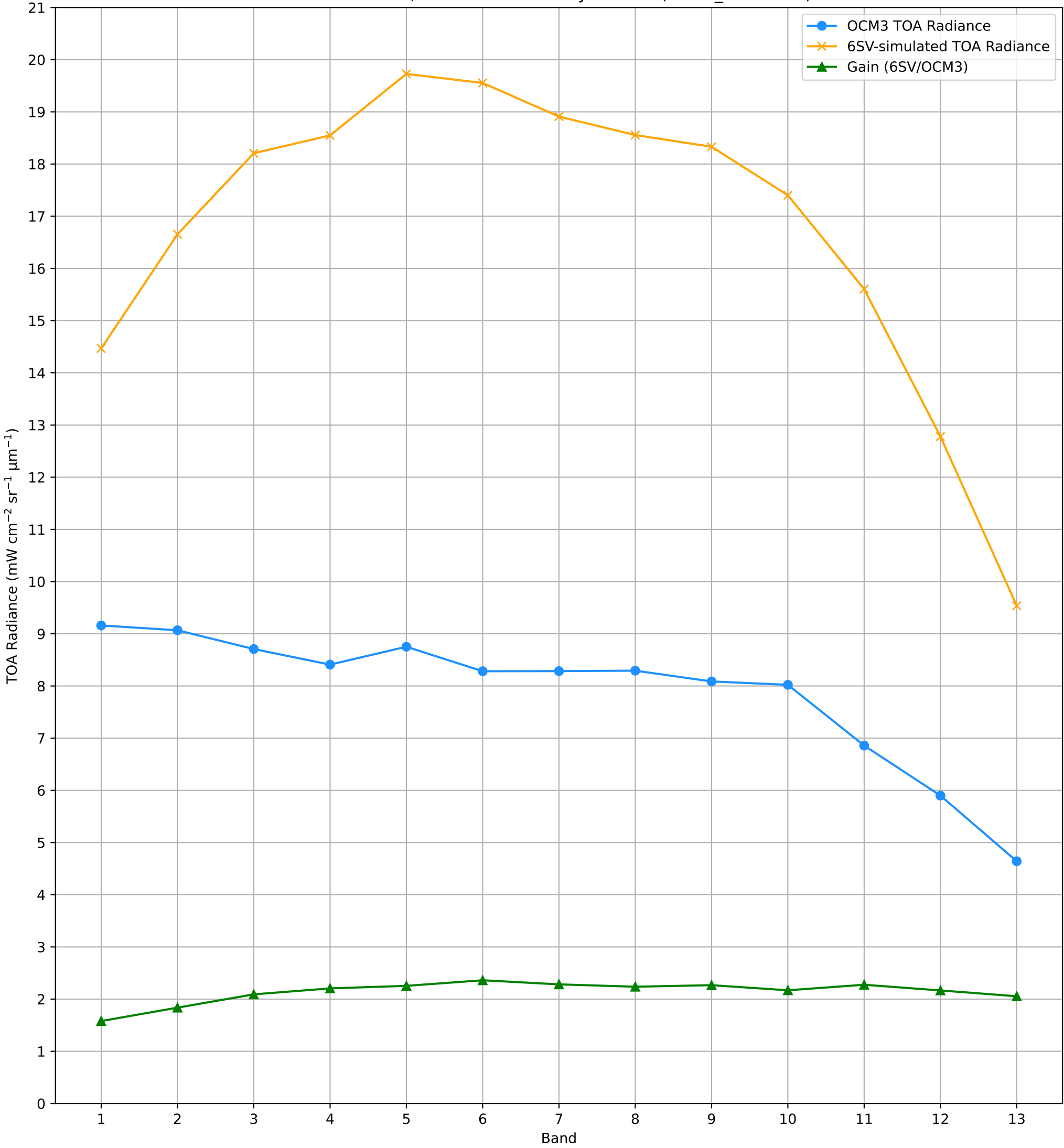
TOA Radiance (OCM3 vs. 6SV) over RVUS RadCalNet Site Lat: 38.497°, Lon: -115.69° - 08-JUL-2025 (STRIP_ID: 13820)
