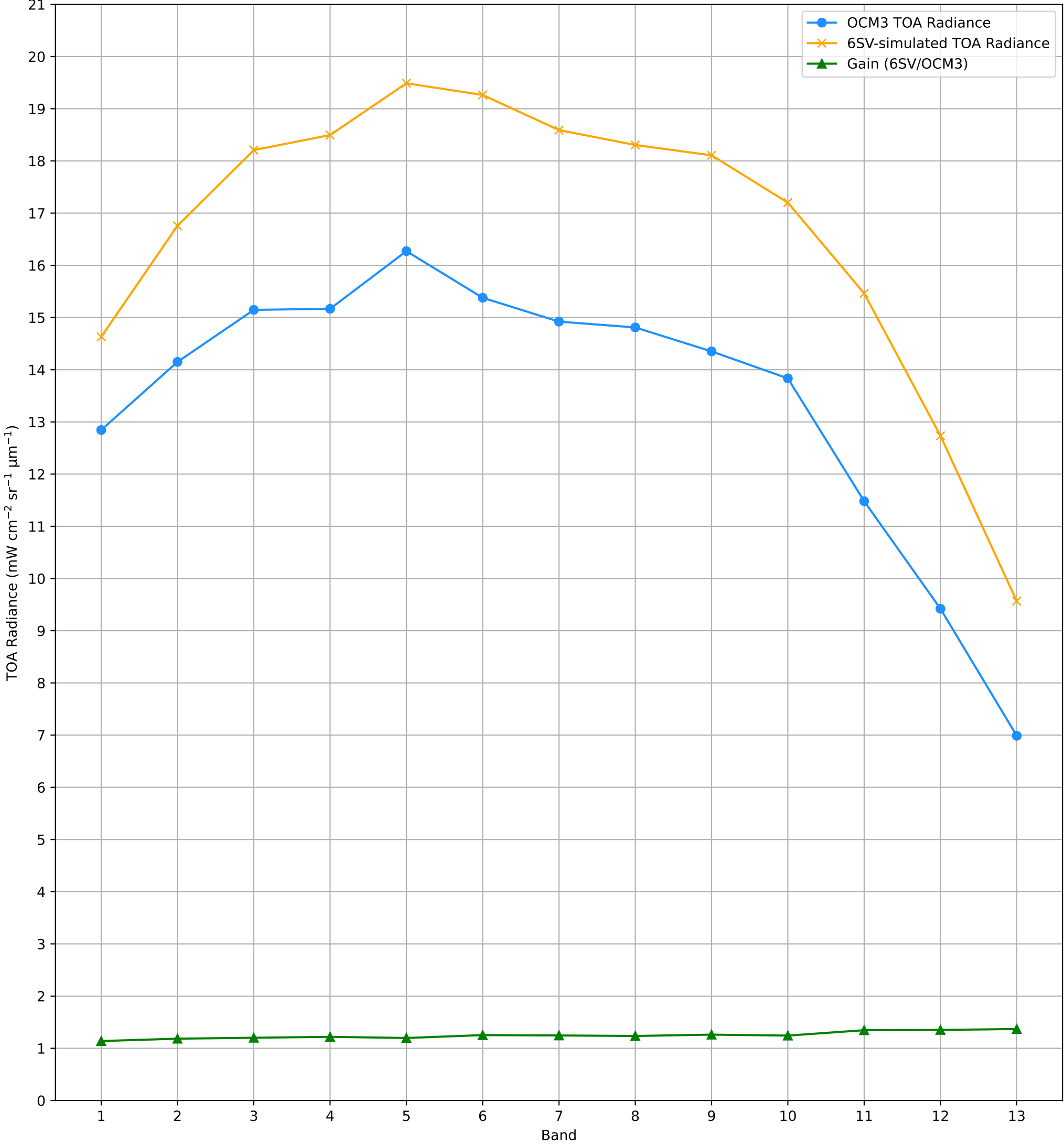
TOA Radiance (OCM3 vs. 6SV) over RVUS RadCalNet Site Lat: 38.497°, Lon: -115.69° - 16-JUL-2025 (STRIP_ID: 13935)
