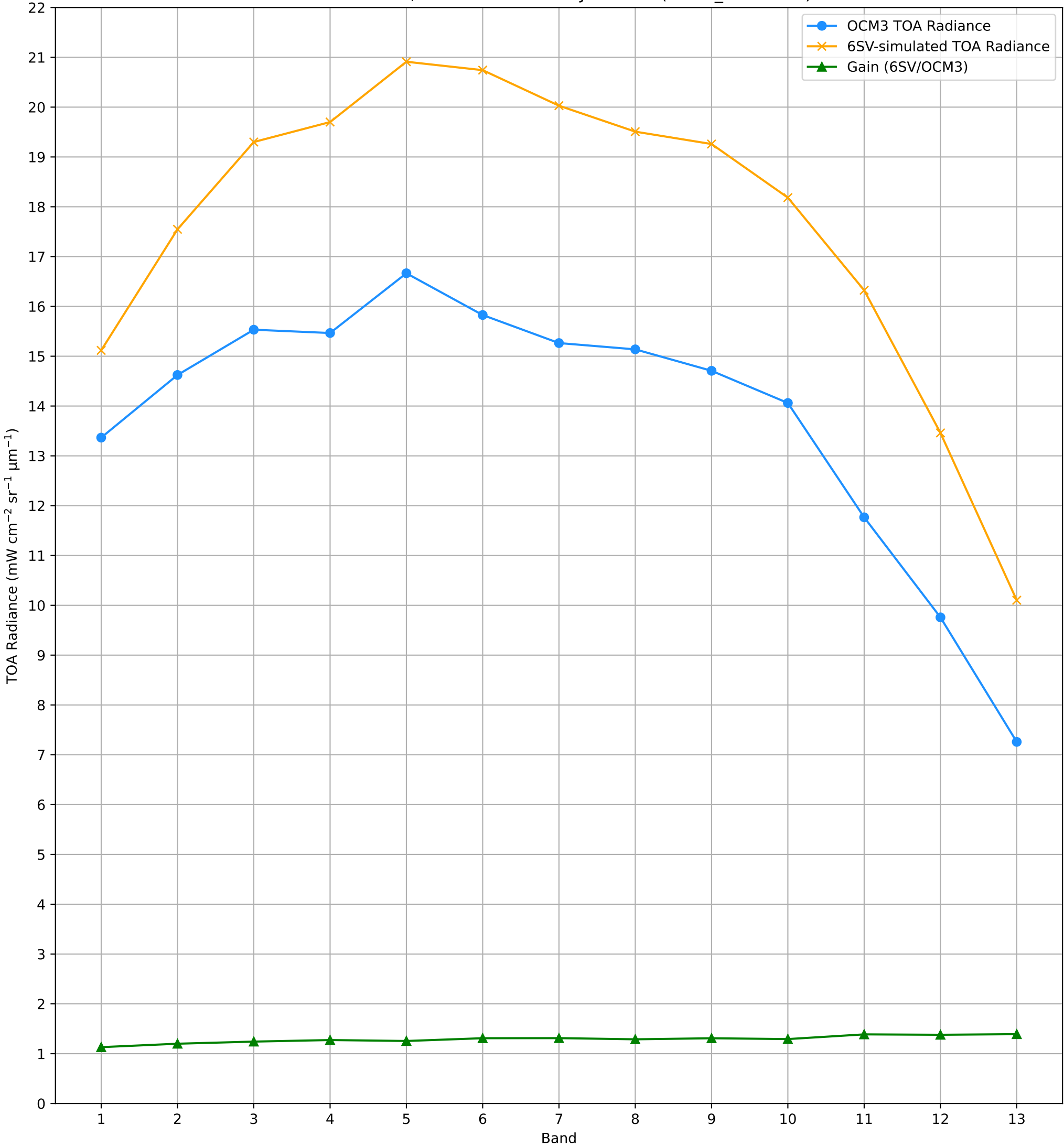
TOA Radiance (OCM3 vs. 6SV) over RVUS RadCalNet Site Lat: 38.497°, Lon: -115.69° - 17-JUL-2025 (STRIP_ID: 13950)
