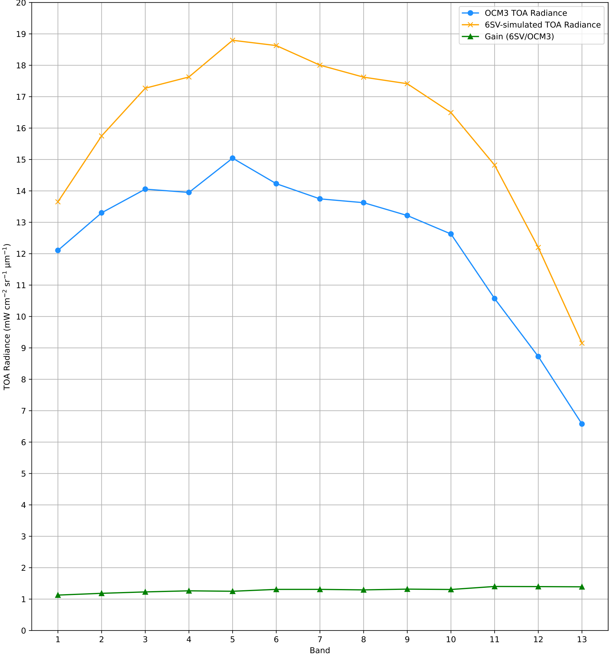
TOA Radiance (OCM3 vs. 6SV) over RVUS RadCalNet Site Lat: 38.497°, Lon: -115.69° - 19-JUL-2025 (STRIP_ID: 13979)
