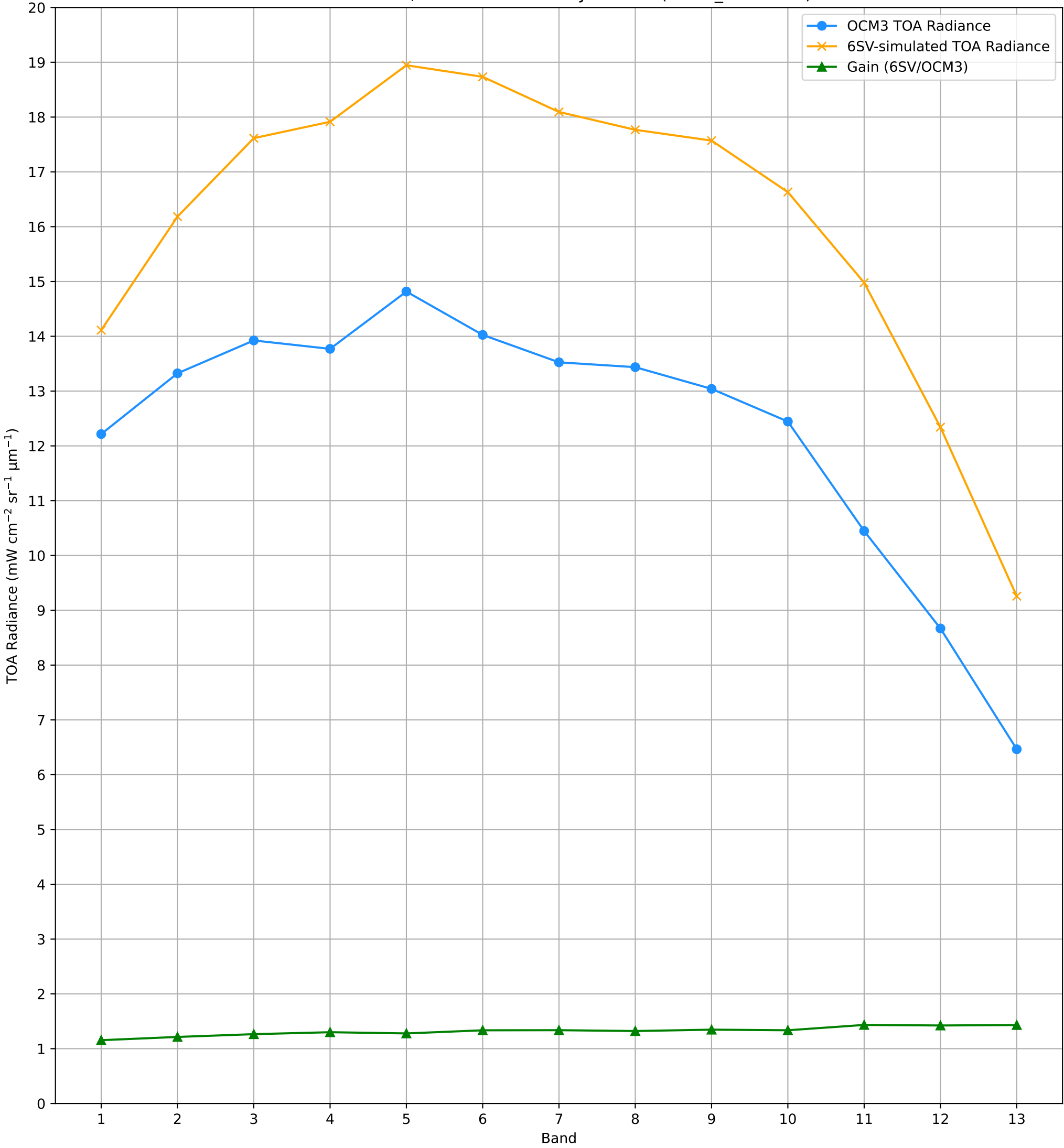
TOA Radiance (OCM3 vs. 6SV) over RVUS RadCalNet Site Lat: 38.497°, Lon: -115.69° - 21-JUL-2025 (STRIP_ID: 14008)
