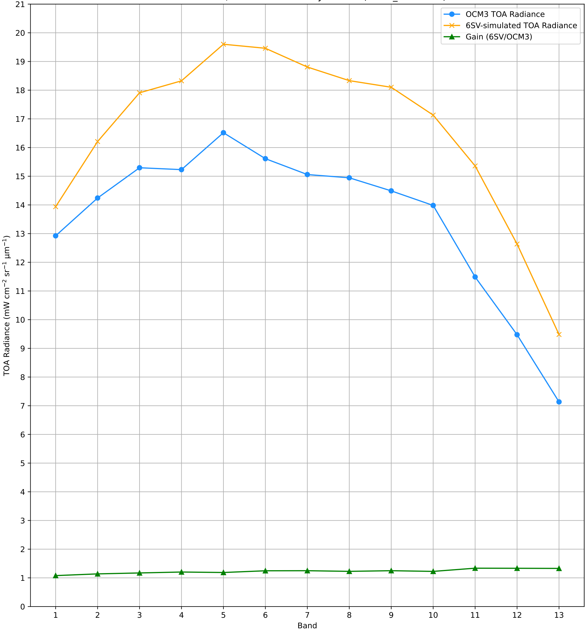
TOA Radiance (OCM3 vs. 6SV) over RVUS RadCalNet Site Lat: 38.497°, Lon: -115.69° - 22-JUL-2025 (STRIP_ID: 14022)
