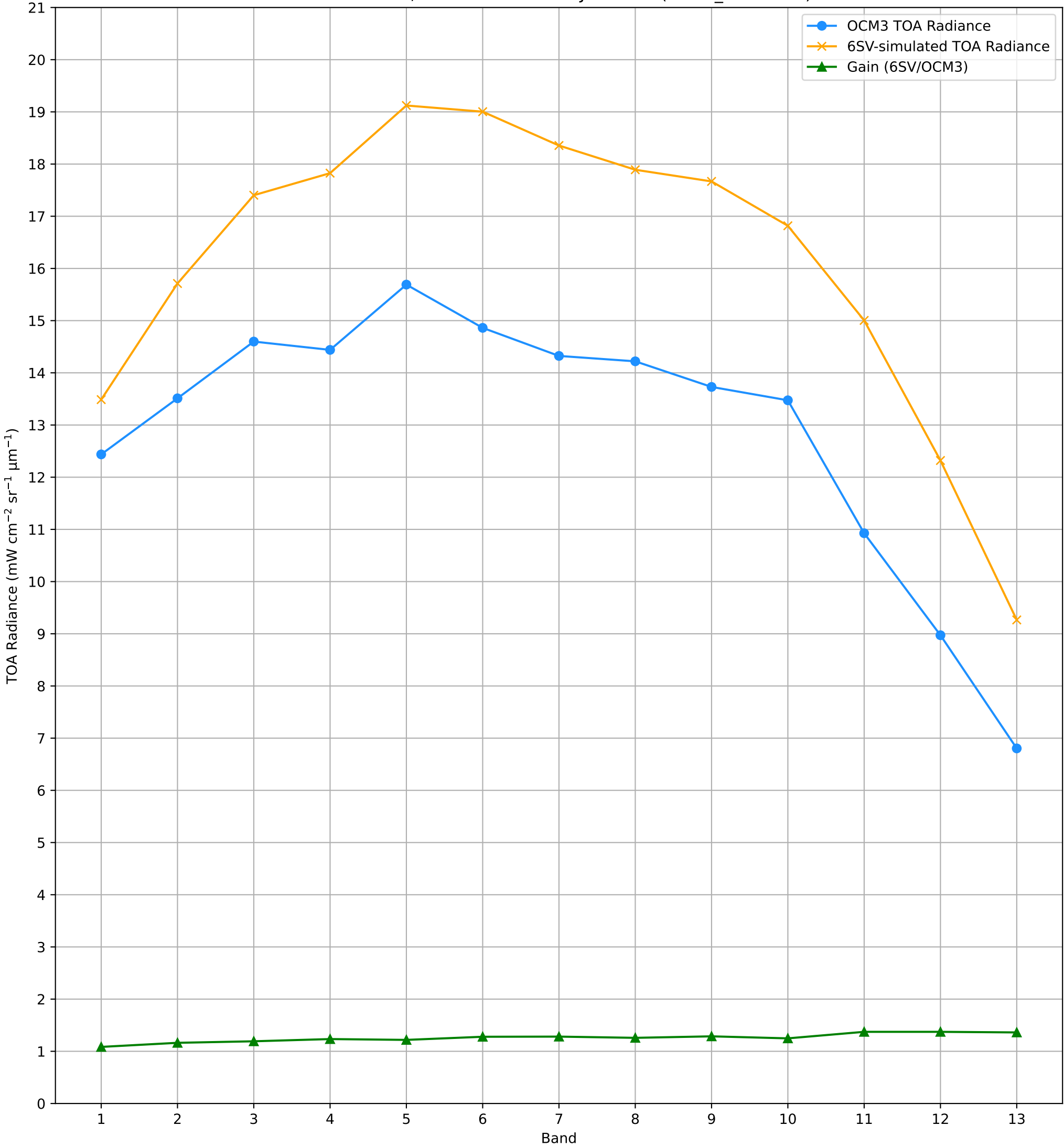
TOA Radiance (OCM3 vs. 6SV) over RVUS RadCalNet Site Lat: 38.497°, Lon: -115.69° - 24-JUL-2025 (STRIP_ID: 14051)
