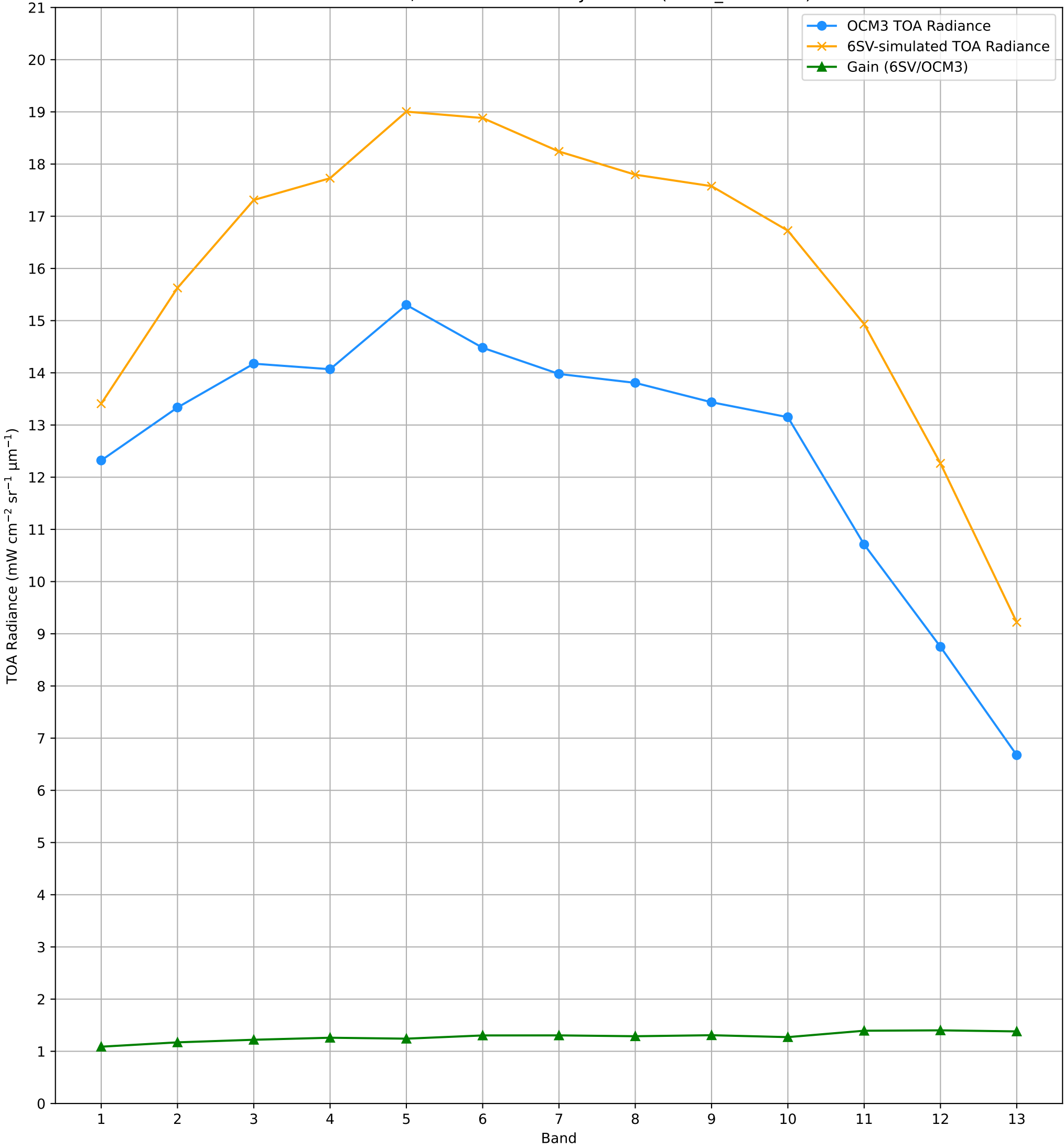
TOA Radiance (OCM3 vs. 6SV) over RVUS RadCalNet Site Lat: 38.497°, Lon: -115.69° - 26-JUL-2025 (STRIP_ID: 14080)
