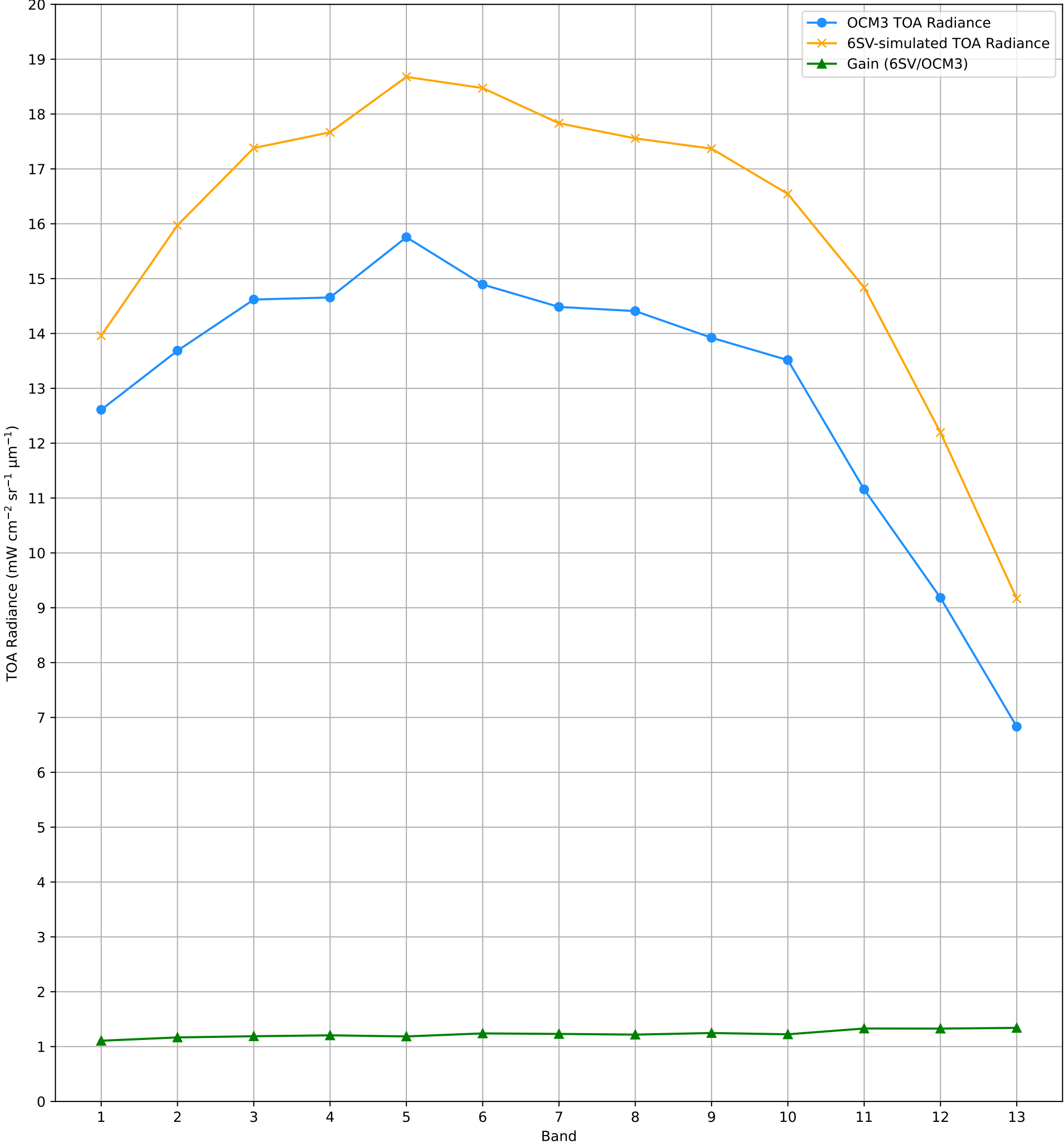
TOA Radiance (OCM3 vs. 6SV) over RVUS RadCalNet Site Lat: 38.497°, Lon: -115.69° - 29-JUL-2025 (STRIP_ID: 14123)
