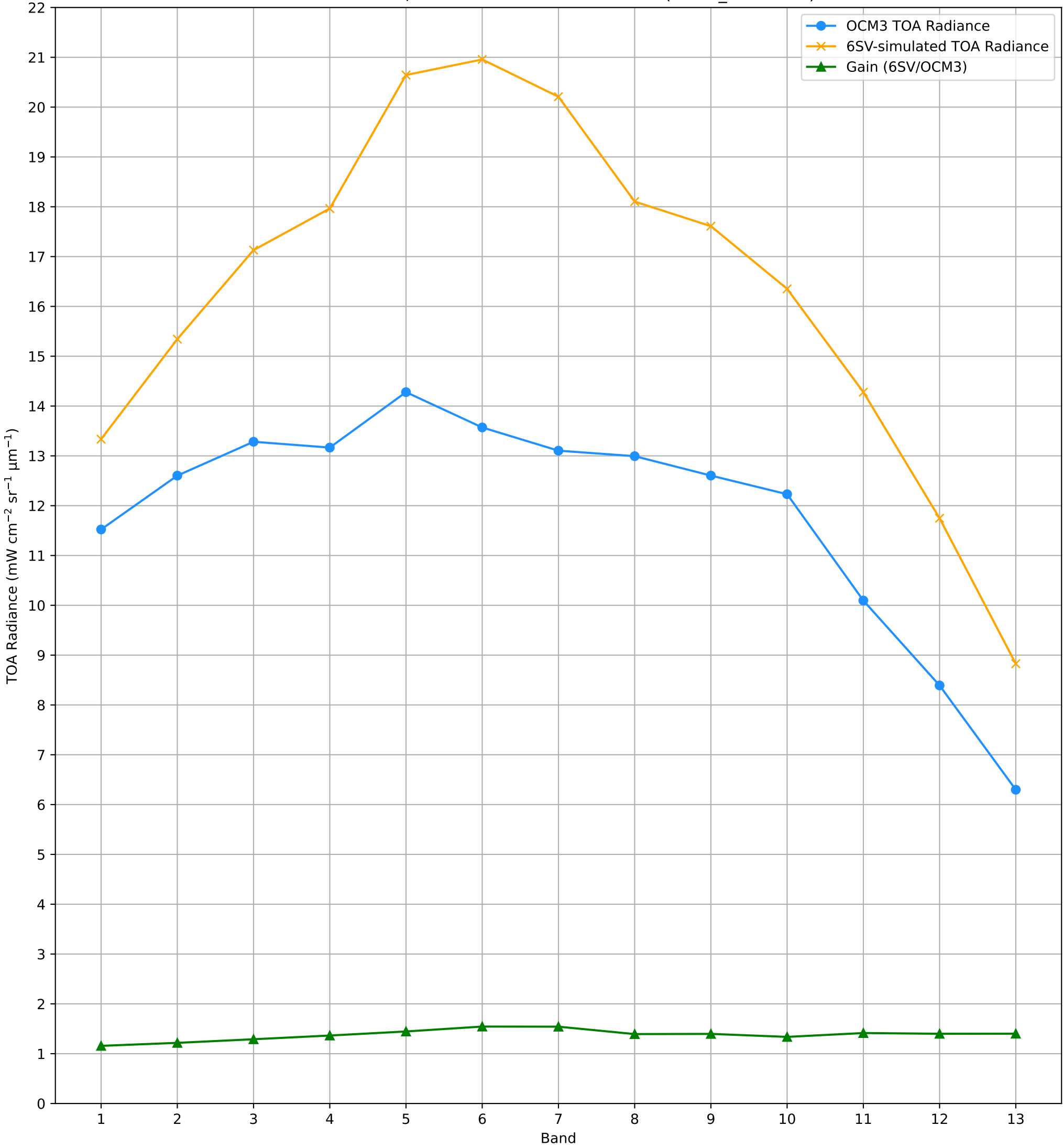
TOA Radiance (OCM3 vs. 6SV) over RVUS RadCalNet Site Lat: 38.497°, Lon: -115.69° - 03-AUG-2025 (STRIP_ID: 14196)
