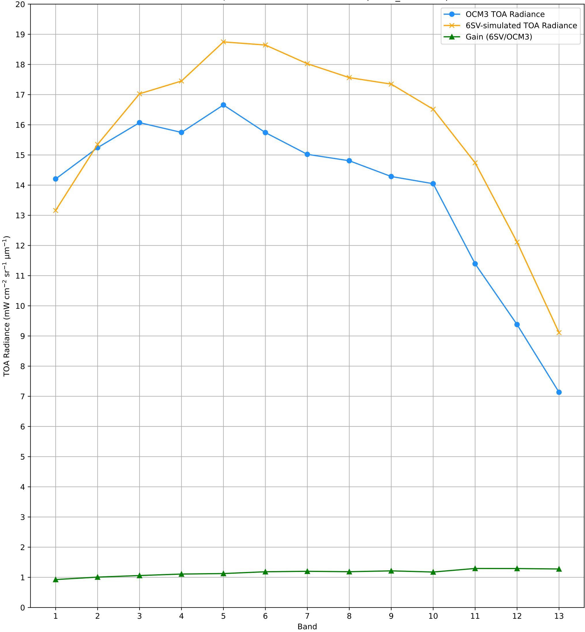
TOA Radiance (OCM3 vs. 6SV) over RVUS RadCalNet Site Lat: 38.497°, Lon: -115.69° - 06-AUG-2025 (STRIP_ID: 14239)
